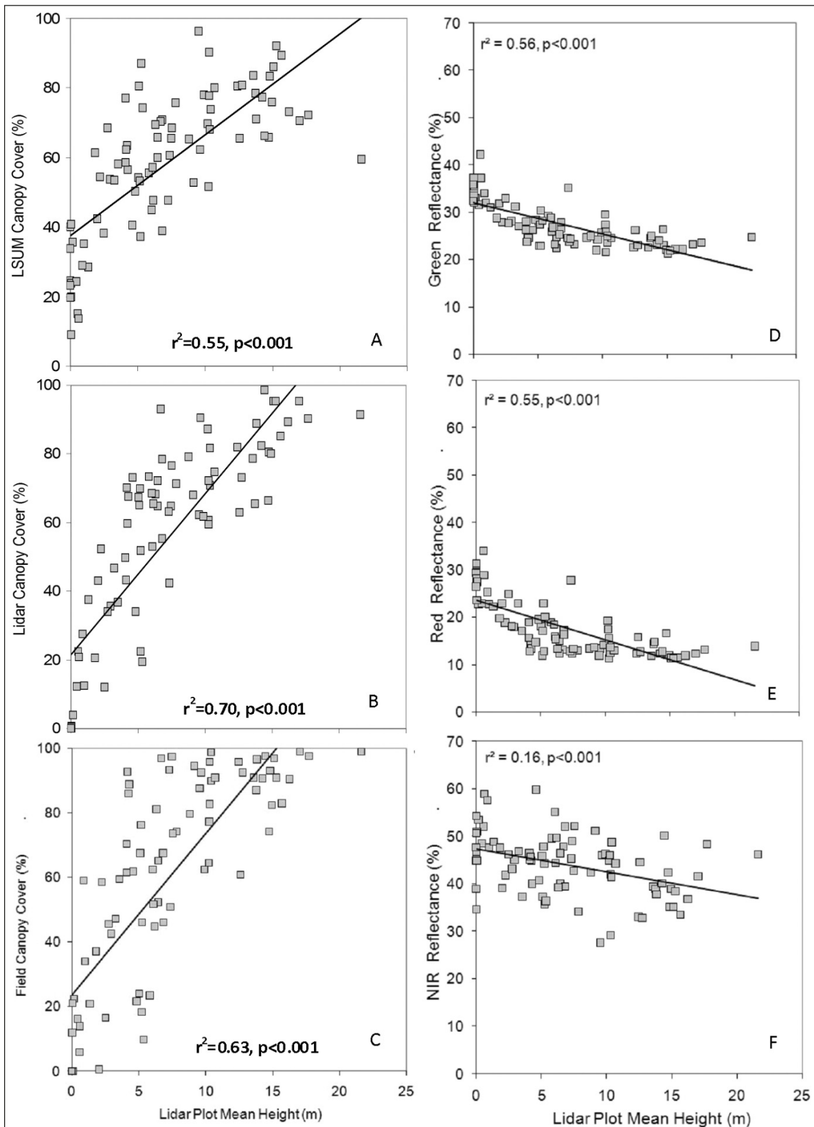
Figure 3. Comparison of the plot mean heights from the lidar data and the spectral (A), lidar (B), and field estimates (C) of percent canopy cover. (D–F) Comparison of plot mean height with reflectance of green (D), red (E), and near-infrared (F) ASTER bands.
