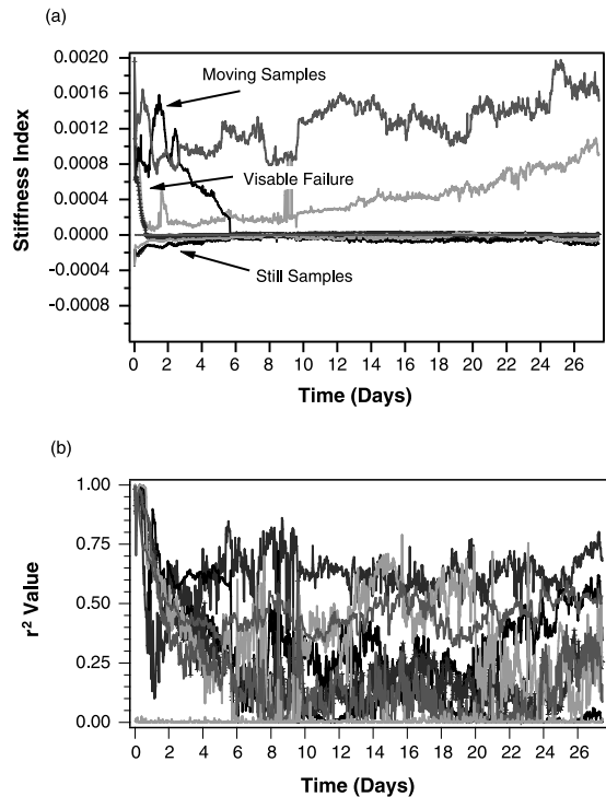
Figure 11—(a) Changes in stiffness index for both samples with movement and no movement. (b) Corresponding squared correlation coefficients, r^2 , as a function of exposure times in days for specimens under “fatigue/hot/wet” conditions. Visible failure is evident in the samples at times less than two days.
