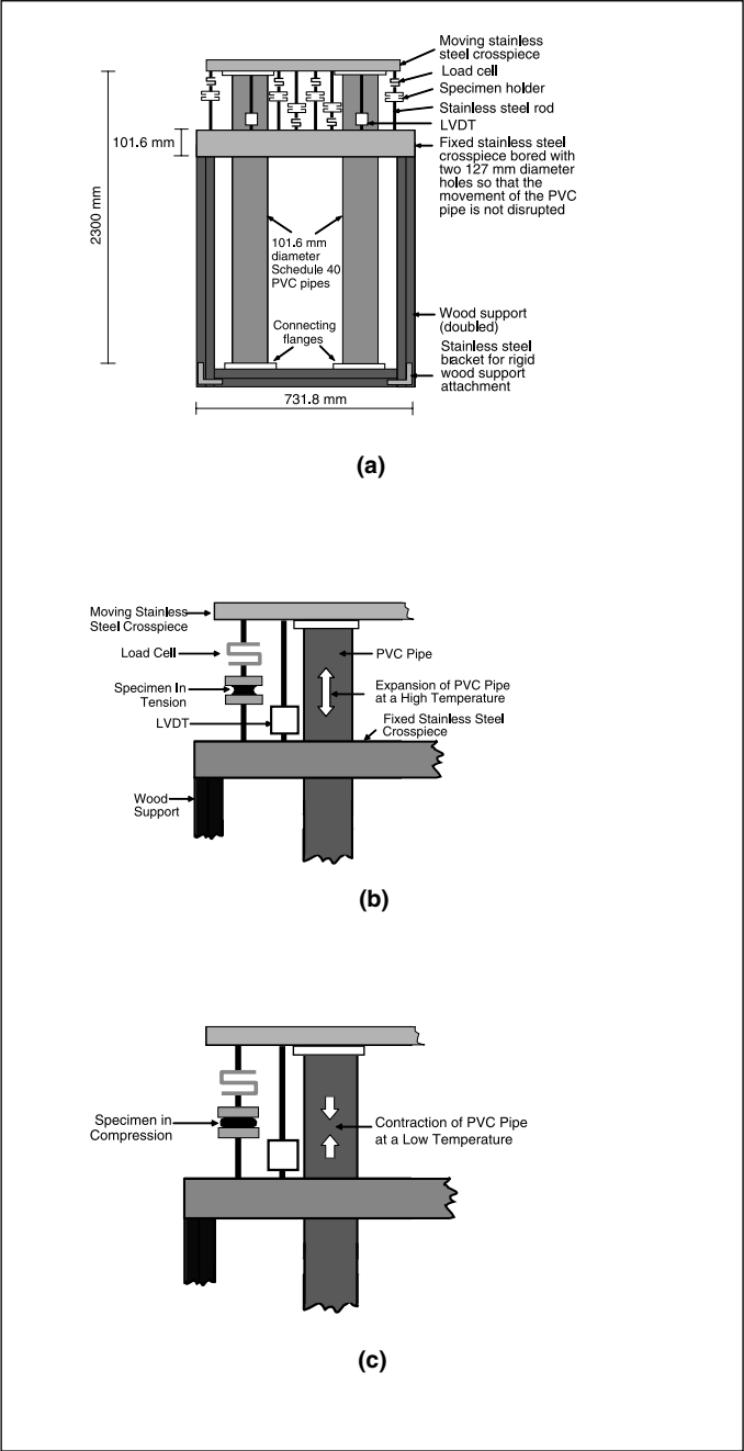
Figure 4—Schematic illustrations of (a) the thermally driven PVC engine, and the mechanism of the engine: (b) at a high temperature, the PVC pipe expands causing the specimen to be loaded in tension; and (c) at a low temperature, the pipe contracts causing the specimen to be loaded in compression. 15
