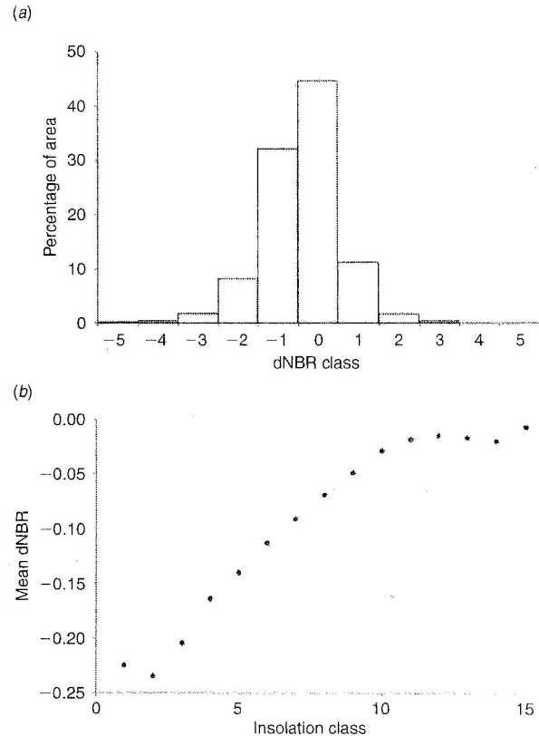
Fig. 5. (a) Histogram of post-fire differenced Normalized Burn Ratio (dNBR) values (4 August–6 September 2004). Each class has a width of 0.1 dNBR units, with class 0 ranging from -0.05 to +0.05 , class 1 ranging from 0.05 to 0.15 , class -1 ranging from -0.15 to -0.05 , etc. (b) Mean post-fire dNBR (4 August–6 September 2004) by insolation for 4 August 2004. Insolation classes correspond to \text{W m}^{-2} at the time of satellite overpass (1, <1 \text{ W m}^{-2} ; 2, 1\text{--}2 \text{ W m}^{-2} ; ... 14, 14\text{--}15 \text{ W m}^{-2} ; 15, >15 \text{ W m}^{-2} ).
