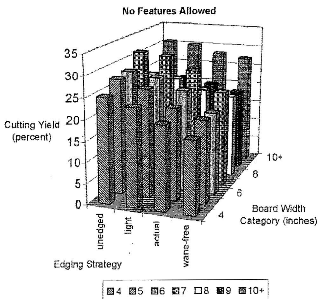
Figure 4. — Cutting yields by board width for all board grades combined using four edging strategies and allowing only clear, two-face parts. Yield percentages are based on the no (none) edging strategy board area.
