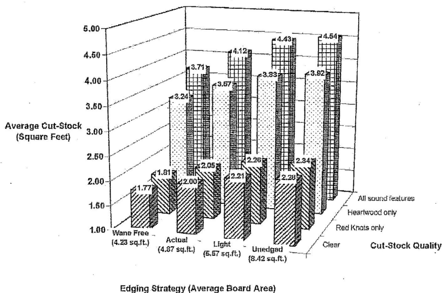
Figure 2. — Average cut-stock production by board edging strategy and cut-stock quality.
