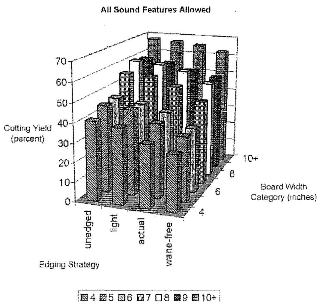
Figure 5. — Cutting yields by board width for all board grades combined using four edging strategies and allowing parts to contain all sound features. Yield percentages are based on the no (none) edging strategy board area.
