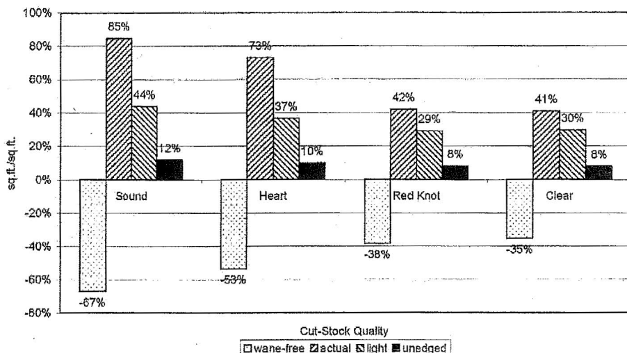
Figure 3. — Cut-stock produced or lost as bounding box area is added or removed from the actual edaina bounding box based on sound features allowed and edaina strategy.
