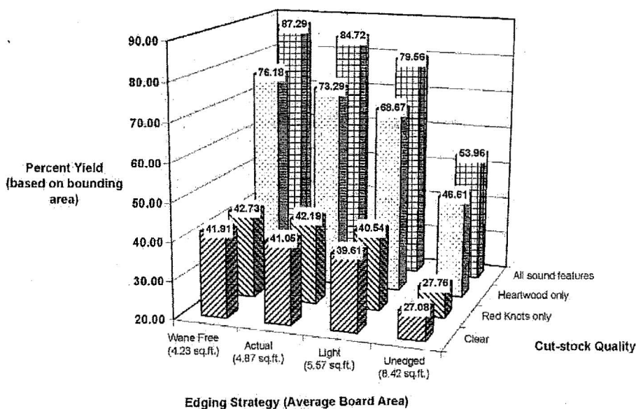
Figure 1. — Average yields for all grades by edging strategy and cut-stock quality.
