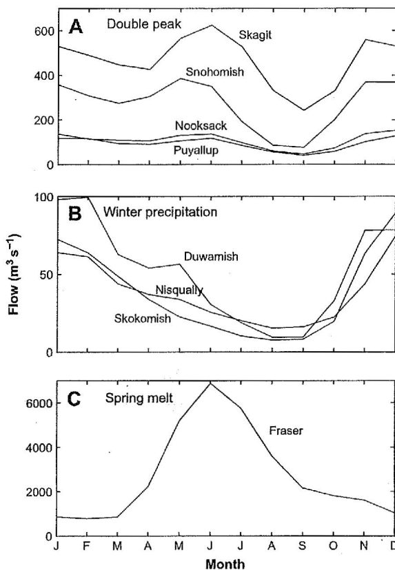
Fig. 4. Climatological monthly mean flow for (A) rivers with a double winter precipitation and spring melt peak (Skagit, Snohomish, Nooksack and Puyallup Rivers), (B) rivers with a single winter precipitation peak (Duwamish, Nisqually and Skokomish Rivers), and (C) the Fraser River with a single spring melt peak in flow from 1993 to 2002. Source: United States Geological Survey and Environment Canada.
