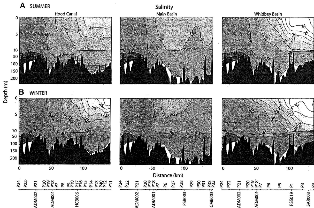
Fig. 6. Mean of summer (panel A) and winter (panel B) salinity along Puget Sound Regional Synthesis Model transects in Main Basin, Whidbey Basin, and Hood Canal from 1998 to 2003.
