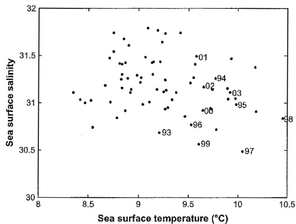
Fig. 8. Annual mean sea surface temperature and salinity at Race Rocks from 1937 to 2002. Values representing the time period examined in this study from 1993 to 2002 are labeled. Figure modified from Moore et al. (2008). Copyright (2008) by the American Society of Limnology and Oceanography, Inc.
