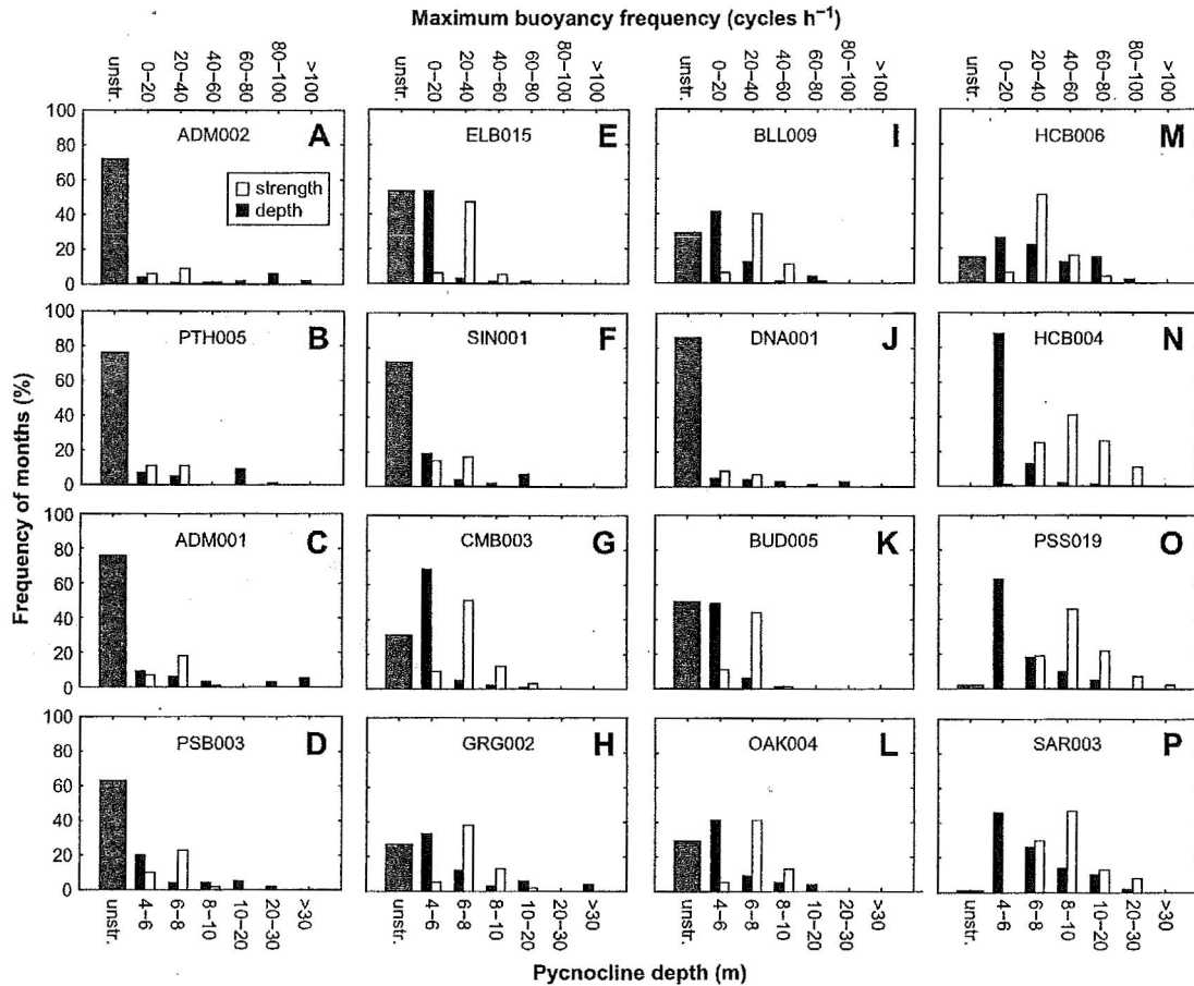
Fig. 7. Frequency distribution of the depth (m) and strength (i.e., maximum buoyancy frequency; cycles \text{h}^{-1} ) of pycnoclines at Marine Waters Monitoring stations for the time period 1993 – 2002. Gray bars indicate unstratified water column conditions.
