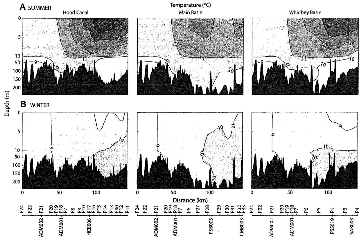
Fig. 5. Mean of summer ( panel A) and winter ( panel B) temperature (°C) along Puget Sound Regional Synthesis Model transects in Main Basin, Whidbey Basin, and Hood Canal from 1998 to 2003. Note that the upper 10 m of the water column is plotted on an enlarged depth scale.
