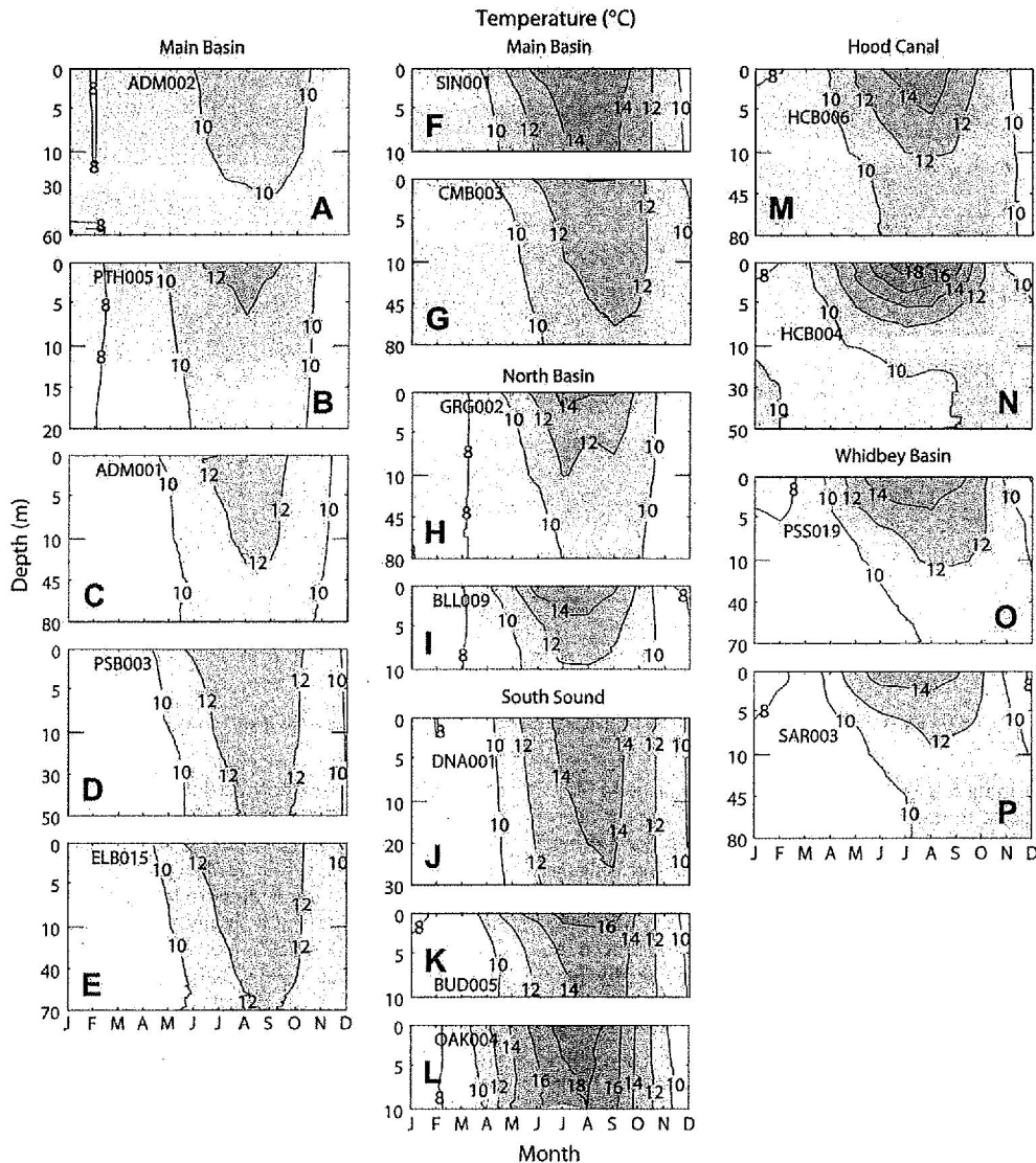
Fig. 2. Climatological monthly means of temperature (°C) at Marine Waters Monitoring stations from 1993 to 2002. Note that the upper 10 m of the water column is plotted on an enlarged depth scale since this is where the greatest variability in oceanographic properties is observed. Depth scaling on the y-axis of each subplot is consistent for the upper 10 m, but varies below this depth depending on the station.
