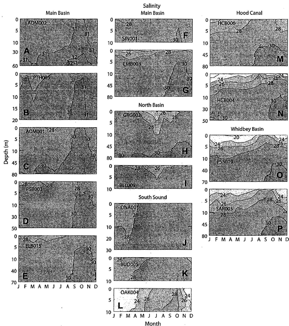
Fig. 3. Climatological monthly means of salinity at Marine Waters Monitoring stations from 1993 to 2002.
