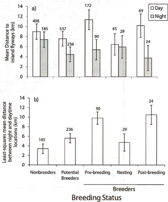
FIGURE 4. Movements and distribution of 32 radio-marked Marbled Murrelets in central California in 2000 and 2001, by breeding status: (a) mean ( \pm 1 SE) distance from flyways used to reach inland nesting habitat during the day and at night; (b) least-squares mean ( \pm 1 SE) distance between nighttime locations and locations the following day. Sample sizes (number of movements) given above bars.
