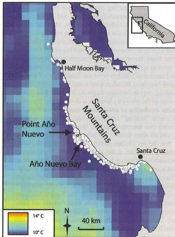
FIGURE 1. At-sea radio-telemetry locations for 32 Marbled Murrelets (white circles; n = 2207 locations) radio-marked in central California in 2000 and 2001. Shaded squares at sea represent sea-surface temperatures derived from a 1-month composite of AVHRR satellite images taken in May of 2000 ( http://las.pfeg.noaa.gov/oceanWatch/oceanwatch.php ). Note the plume of cold, upwelled water originating from Point Año Nuevo.
