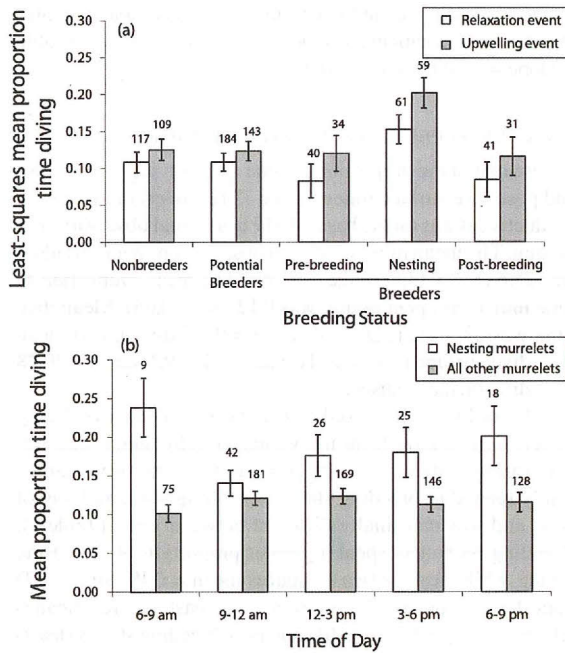
FIGURE 6. Diving behavior of 32 radio-marked Marbled Murrelets in central California in 2000 and 2001: (a) least-squares mean ( \pm 1 SE) proportion time spent diving by breeding status and upwelling state; (b) mean ( \pm 1 SE) proportion time spent diving by time of day and nesting status. Sample sizes (number of 1-hr dive surveys) given above bars.
