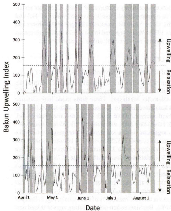
FIGURE 2. Bakun Upwelling Index (Bakun 1973) calculated at the National Oceanic and Atmospheric Administration's Buoy 46042 (36° N, 122° W) in the spring and summer of 2000 and 2001. The upwelling index was derived from the intensity of atmospheric pressure gradients that generate upwelling-favorable (i.e., northwesterly) winds and was measured as the volume ( m^3 ) of water transported offshore per second per 100 m of coastline. Days with an upwelling index >150 are shaded grey and assigned to "upwelling" events; days with an index <150 are shaded white and assigned to "relaxation" events.
