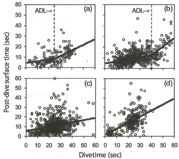
FIGURE 7. Relationship between dive time and post-dive surface time for four representative Marbled Murrelets radio-marked in central California in 2000 and 2001. Competing one-slope (indicative of aerobic respiration only) and two-slope (indicative of aerobic and anaerobic respiration) regression models were fit to the data and evaluated with AIC c . Two-slope models received more support for the two individuals in (a) and (b); one-slope models were better supported for the two individuals in (c) and (d). ADL = aerobic dive limit.
