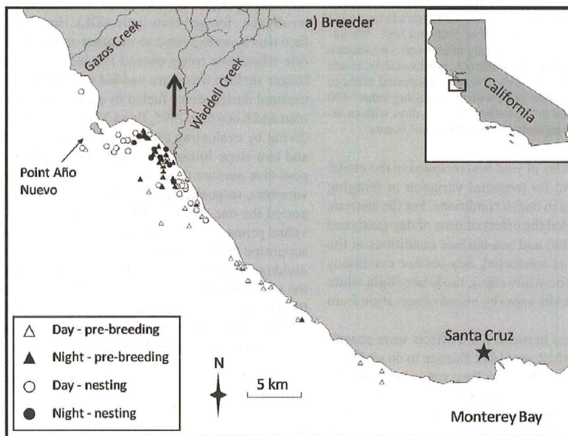
FIGURE 3. Daytime and nighttime radio-telemetry locations for three representative Marbled Murrelets radio-marked in central California in 2000 and 2001: (a) a breeder during the pre-breeding and nesting period; (b) a potential breeder that did not nest but was physiologically in breeding condition; (c) a nonbreeder. The breeder and potential breeder typically flew up Waddell Creek early in the morning to reach nesting habitat (denoted by the black arrow; Peery et al. 2004a). The nonbreeder was never detected flying inland.
