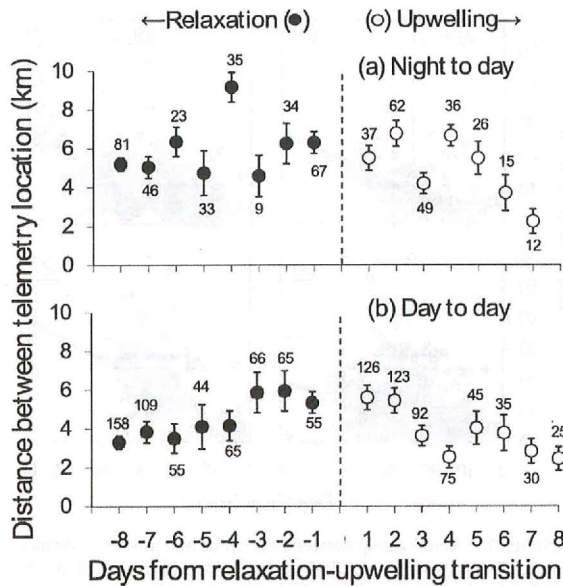
FIGURE 5. Mean ( \pm 1 SE) distance traveled by 32 radio-marked Marbled Murrelets in central California in 2000 and 2001 as a function of upwelling conditions: (a) between nighttime resting locations and foraging locations the following day; (b) daytime locations on consecutive days. Sample sizes (number of movements) given above and below symbols.
