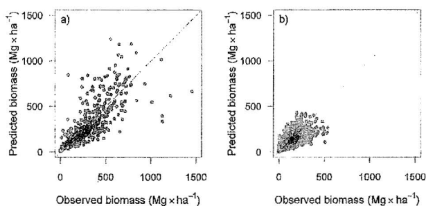
Figure 4. Observed versus predicted aboveground biomass (Mg ha -1 ) for the Cascade (left, RMSE = 174.7 Mg ha -1 , n = 362) and Appalachian study region (right, RMSE = 60.6 Mg ha -1 , n = 3,054)
