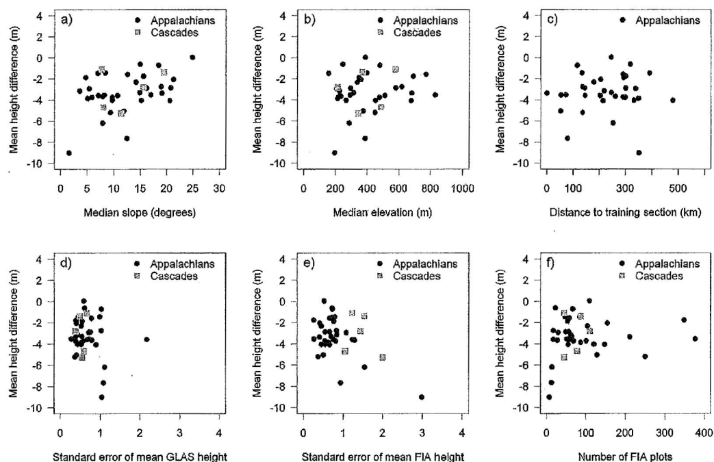
Figure 3. Scatterplots showing the bias (difference) between mean GLAS and mean FIA height at the ecosection level versus (a) median slope and (b) elevation of forested area, (c) distance to the geographic center of the ecological subsection with the training data, (d) standard error of mean GLAS height, (e) standard error of FIA dominant height, and (f) number of FIA plots.
