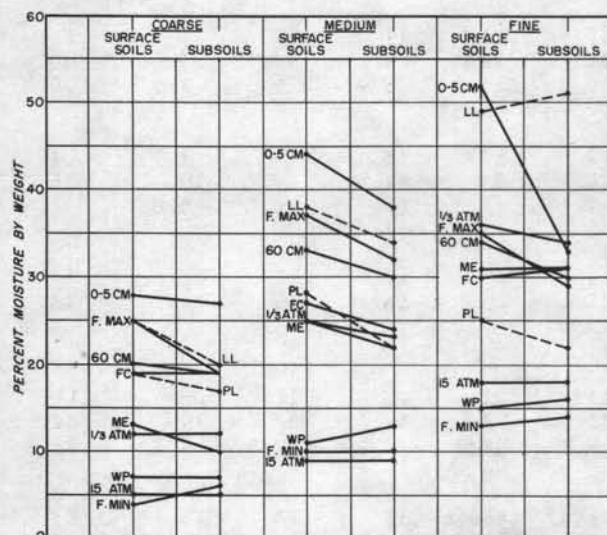
Figure 3.--Average moisture constants, by weight, for coarse, medium, and fine soils.
