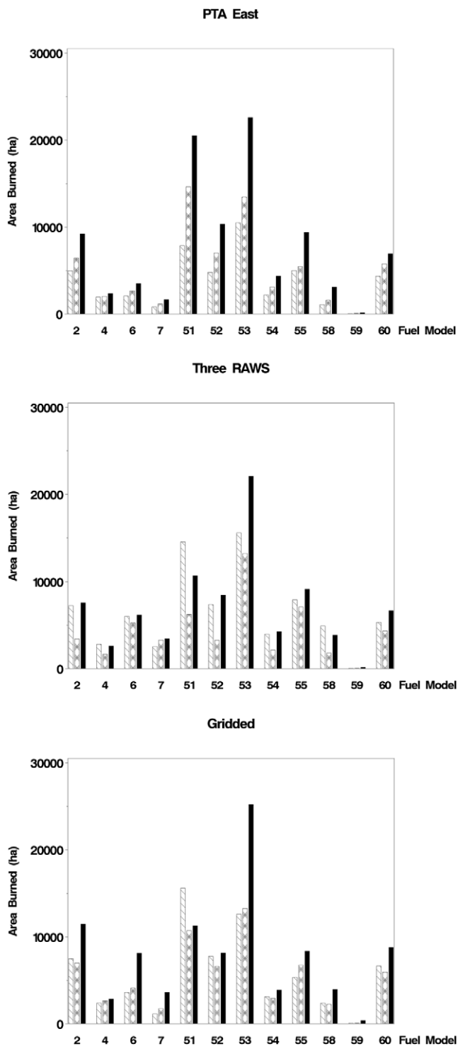
FIGURE 4. Total area burned for nine simulated weather scenarios (three weather percentiles \times three weather data sources), Pōhakuloa Training Area, Hawai'i. Within a fuel model, the weather percentiles from left to right are 50th, 75th, and 95th. Fuel model numbers are defined in Figure 3. Only PTA East simulations consistently resulted in positive correlation between area burned and weather percentile for all fuel models.
