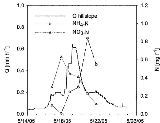
Fig. 5. Hillslope discharge and NO 3 -N and NH 4 -N patterns in transient groundwater from well E04, during storm 5.
