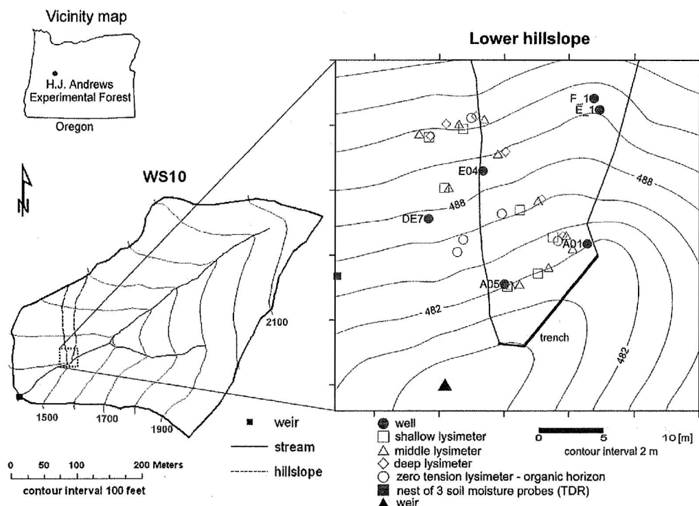
Fig. 1. Map of WS10 showing the location of the hillslope study area and lower hillslope with the instrumentation.
