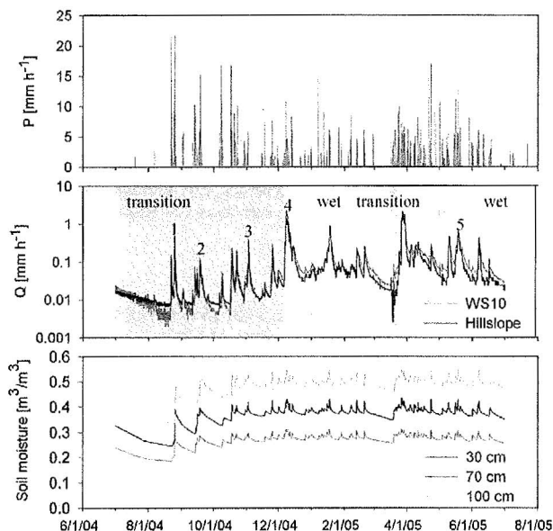
Fig. 2. Time series of hydrological data during the study period: (a) rainfall, (b) discharge from the hillslope and watershed with different hydrological conditions during the year: transition periods (light gray background) characterized by an increase in hillslope and watershed baseflow and soil moisture and a wet period (white background) characterized by high 'steady' hillslope and watershed baseflow conditions. The numbers in the graph refer to storms that were sampled and (c) soil moisture content ( m^3/m^3 ).
