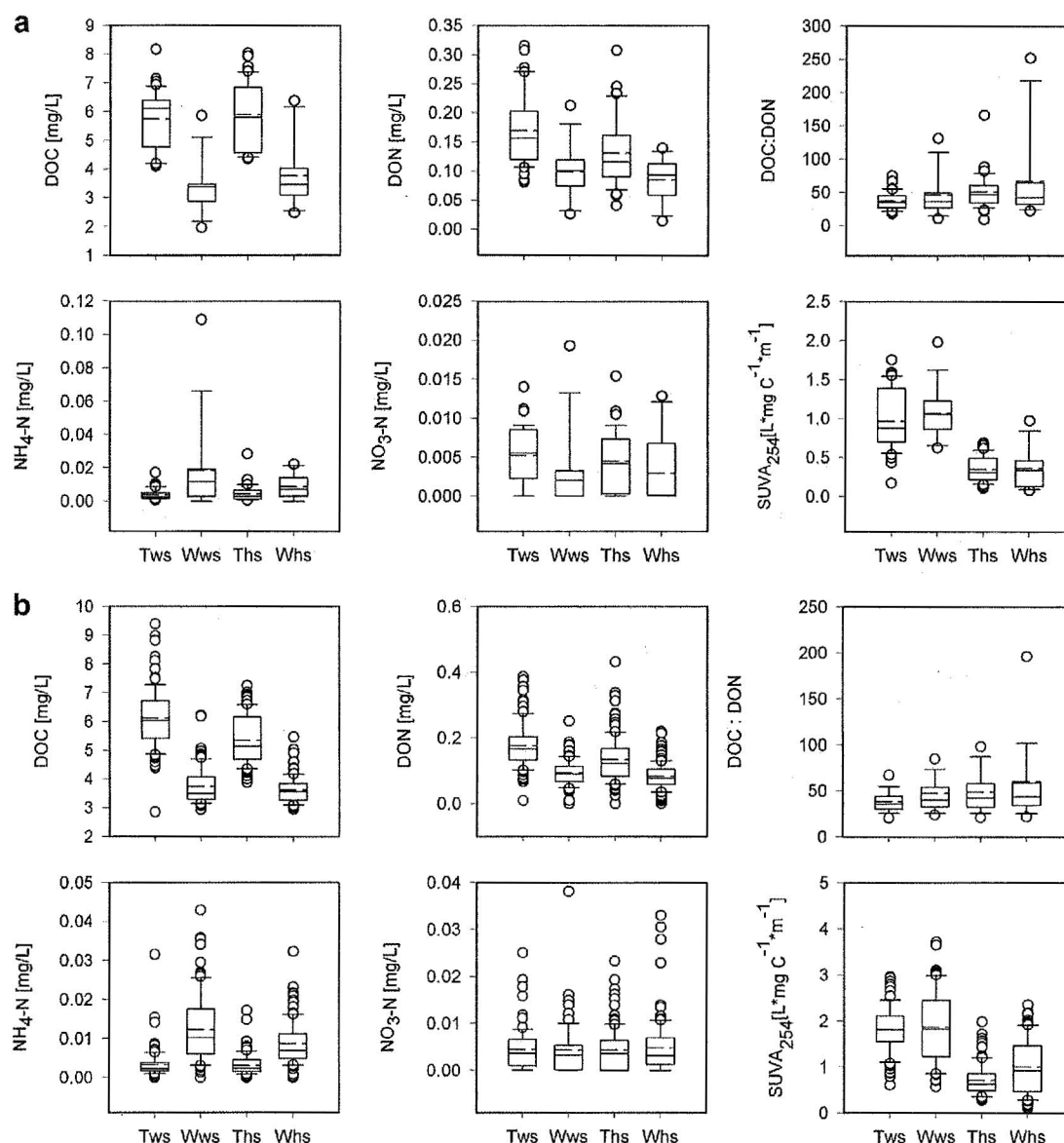
Fig. 3. Box plots of DOC, DON, NH 4 -N, NO 3 -N concentrations, DOC:DON and SUVA during (a) baseflow conditions and (b) stormflow conditions, during different hydrological conditions (T = transition period, W = wet period) for stream water at WS10-outlet (ws) and lateral subsurface flow from the trenched hillslope (hs). The dashed line in the box plot is the average value and the solid line is the median value. The boundary of the box indicates the 75th percentile. The error bars above and below the box indicate, respectively, the 90th and 10th percentile. Circles are outliers.
