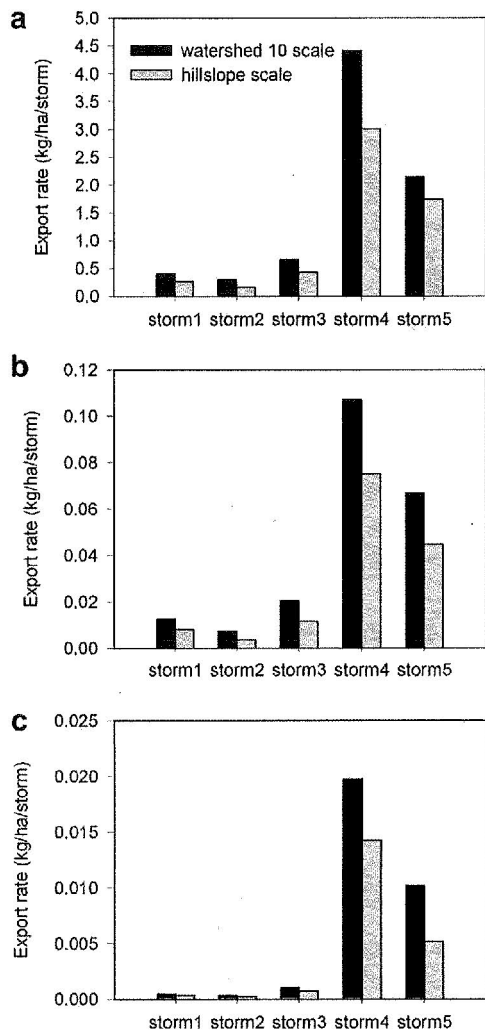
Fig. 4. Export rates of: (a) DOC, (b) DON and (c) DIN, during sampled storms at the watershed and hillslope scale.
