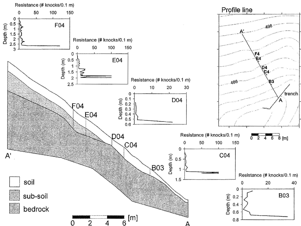
Figure 11 Cross-section of the hillslope above the trench along the profile line A–A'. Depth to bedrock and soil resistance was measured with a knocking pole. Maximum soil depth was assumed to be 1.1 m based on Ranken (1974) and Harr (1977). Depth to bedrock was defined as at least 20 knocks per 0.1 m.
