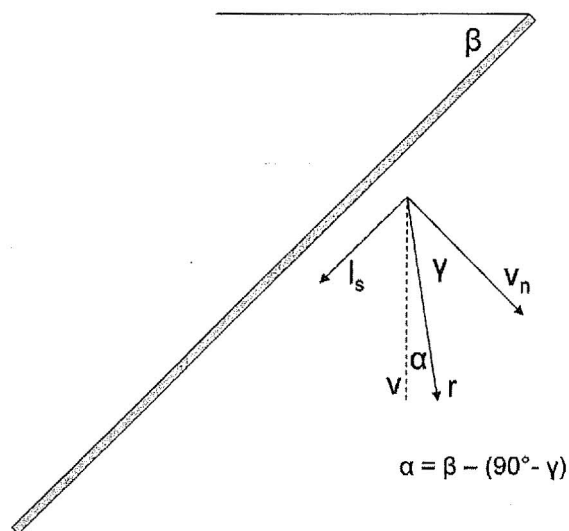
Figure 2 Schematic overview of gradients; l_s and v_n are the lateral (parallel to the slope) and vertical gradient (normal to slope), respectively, r is the resultant gradient of l_s and v_n , and v is the vertical. The flow direction deviation from the vertical is \alpha .
