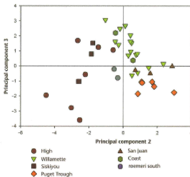
Figure 5. Plot of principal component 2 and 3 for Festuca roemerii in the common-garden study. The "Oregon" population cluster includes Willamette Valley and coastal populations. The "Washington" cluster includes both Puget Trough and San Juan populations.
