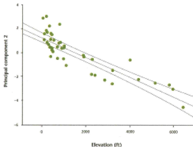
Figure 4. Regression of the second principal component and elevation of the source population for Festuca roemerii . R^2 = 0.7522 . 95% confidence intervals shown.
