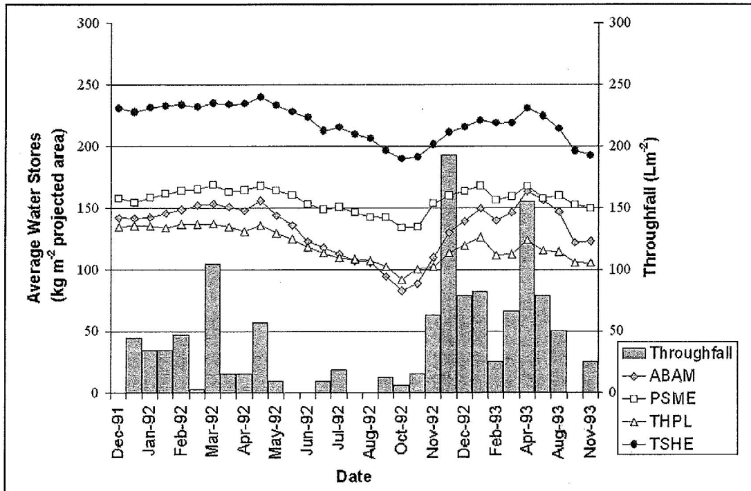
Figure 2. Average water stores ( \text{kg m}^{-2} ; left vertical axis) of projected surface area of decaying logs and throughfall ( \text{L m}^{-2} ) plotted through time. Two measurements were made from different sections of the same log for Abies amabilis (ABAM), Pseudotsuga menziesii (PSME), Thuja plicata (THPL), and Tsuga heterophylla (TSHE).
