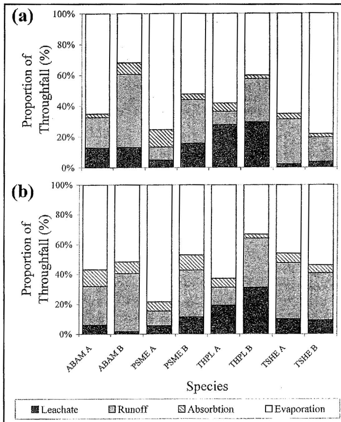
Figure 3. Partition of throughfall water for four species (ABAM = Abies amabilis , PSME = Pseudotsuga menziesii , THPL = Thuja plicata , and TSHE = Tsuga heterophylla ) of decomposing logs among measured absorption, runoff, and leachate, and calculated evaporation. Two sections taken from the same log for each species are shown. Two winters of precipitation were examined: (a) December, 1991 - June 1992 (377 mm throughfall) and (b) July 1992 - April 1993 (718 mm throughfall). The time period in 1991-1992 received below average precipitation, whereas the time period 1992-1993 received above average precipitation.
