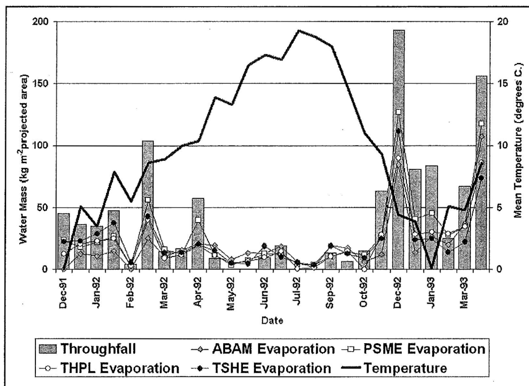
Figure 4. Average evaporated water mass ( \text{kg m}^{-2} ) and throughfall ( \text{kg m}^{-2} ) estimated by measurement period (approximately two weeks) through time. Two measurements were made from different sections of the same log for Abies amabilis (ABAM), Pseudotsuga menziesii (PSME), Thuja plicata (THPL), and Tsuga heterophylla (TSHE). Mean Temperature (right vertical axis) was measured at nearby Corvallis Water Bureau meteorological station 7 km to the west, at about the same elevation. Mean temperature is the mean of the daily maximum and minimum temperatures recorded for that day.
