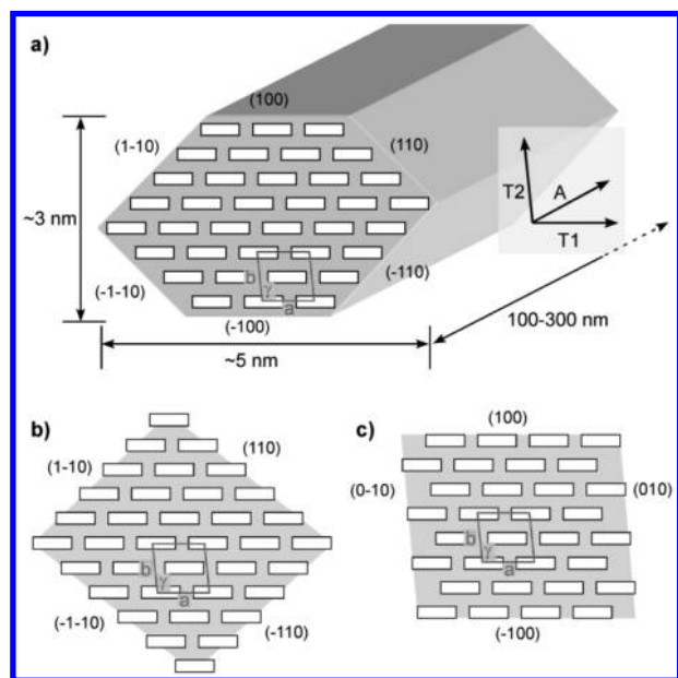
Figure 2. Schematic cross section of an idealized CNCs showing the monoclinic arrangement of 36 cellulose chains (cellulose I β crystalline structure). The box indicates the cellulose I β lattice with a = 0.786 nm, b = 0.817 nm, and \gamma = 97^\circ . 5 (a) shows the cross section as described by Ding and Himmel. 29 (b, c) Other possible cross sections. The anisotropic structures of cellulose I in the axial and transverse directions are labeled A, T1, and T2, respectively (consistent with Table 2).
