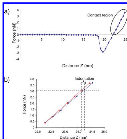
Figure 4. (a) Plot of F(z) data acquired on a CNC. (b) The area marked by an oval is shown with the measured F(z) curve (blue \diamond ) on CNC and on mica (red \blacktriangle ). By finding the difference between z values at a given force, the CNC indentation can be obtained at each force value, F(\delta) .
