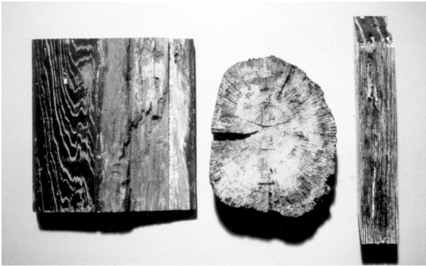
Figure 4. Fungal decay of wood by brown-rot decay fungi. (Source: Forest Products Society)
