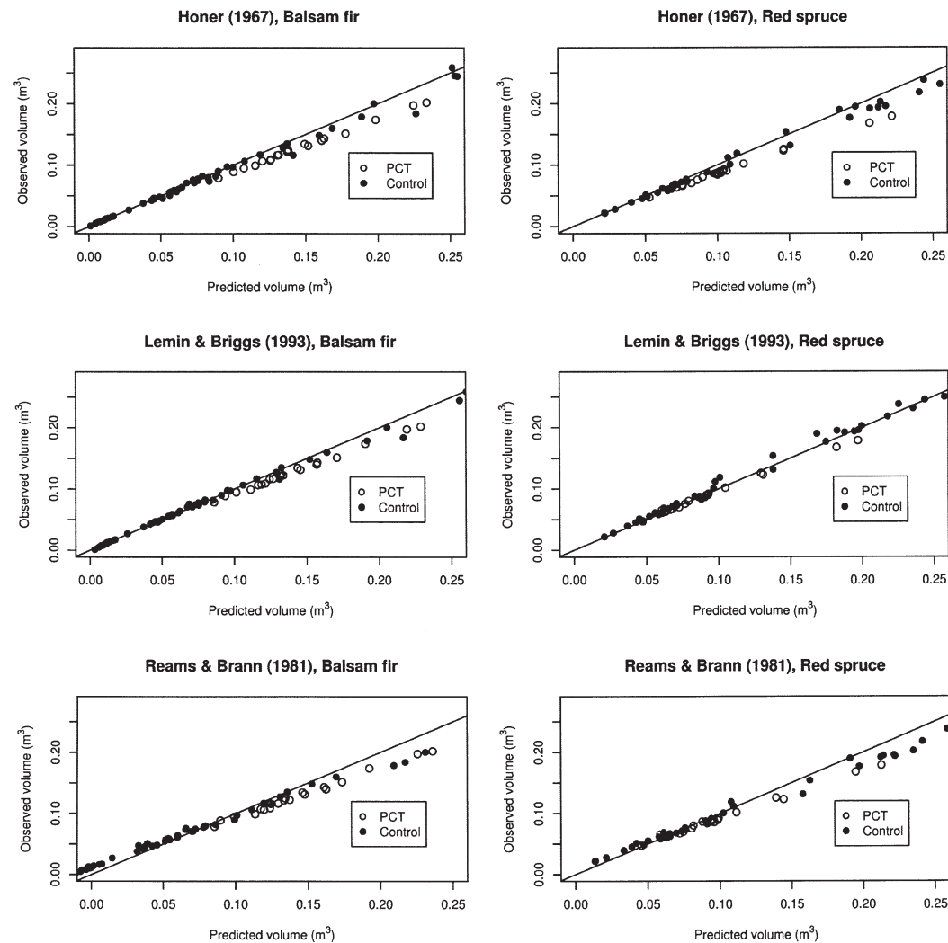
Fig. 2. Relationship between observed and predicted volume ( \text{m}^3 ) for PCT and control trees by species. Volume was predicted using the Honer (1967), Lemin and Briggs (1993), and Reams and Brann (1981) equations.
