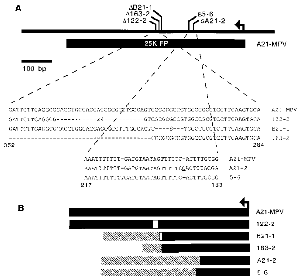
FIG. 5. Sequence analysis of the 25K FP genes in the FP mutants. (A) Schematic presentation of the locations and sequences of the 25K FP mutations within the LdMNPV FP mutants. The sequences are numbered with respect to the ATG start codon of the wild-type 25K FP gene. Dashes indicated the positions of the deletions or insertions (IS) in the FP mutants. The inserted base in A21-2 is underlined. (B) Predicted effects of the mutations on the 25K FP proteins expressed in the FP mutants. Solid areas, regions homologous to the wild-type protein; open areas, deleted regions; hatched areas, nonhomologous regions within the fusion proteins as a consequence of the frameshift mutations.
