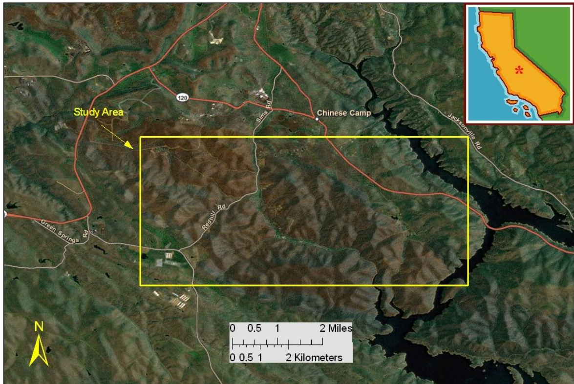
Figure 1. Red Hills (podiform chromite) study area location map, Toulumne County, California. The red soil coloration visible in the imagery is due to limited vegetative cover and high soil-iron content.
