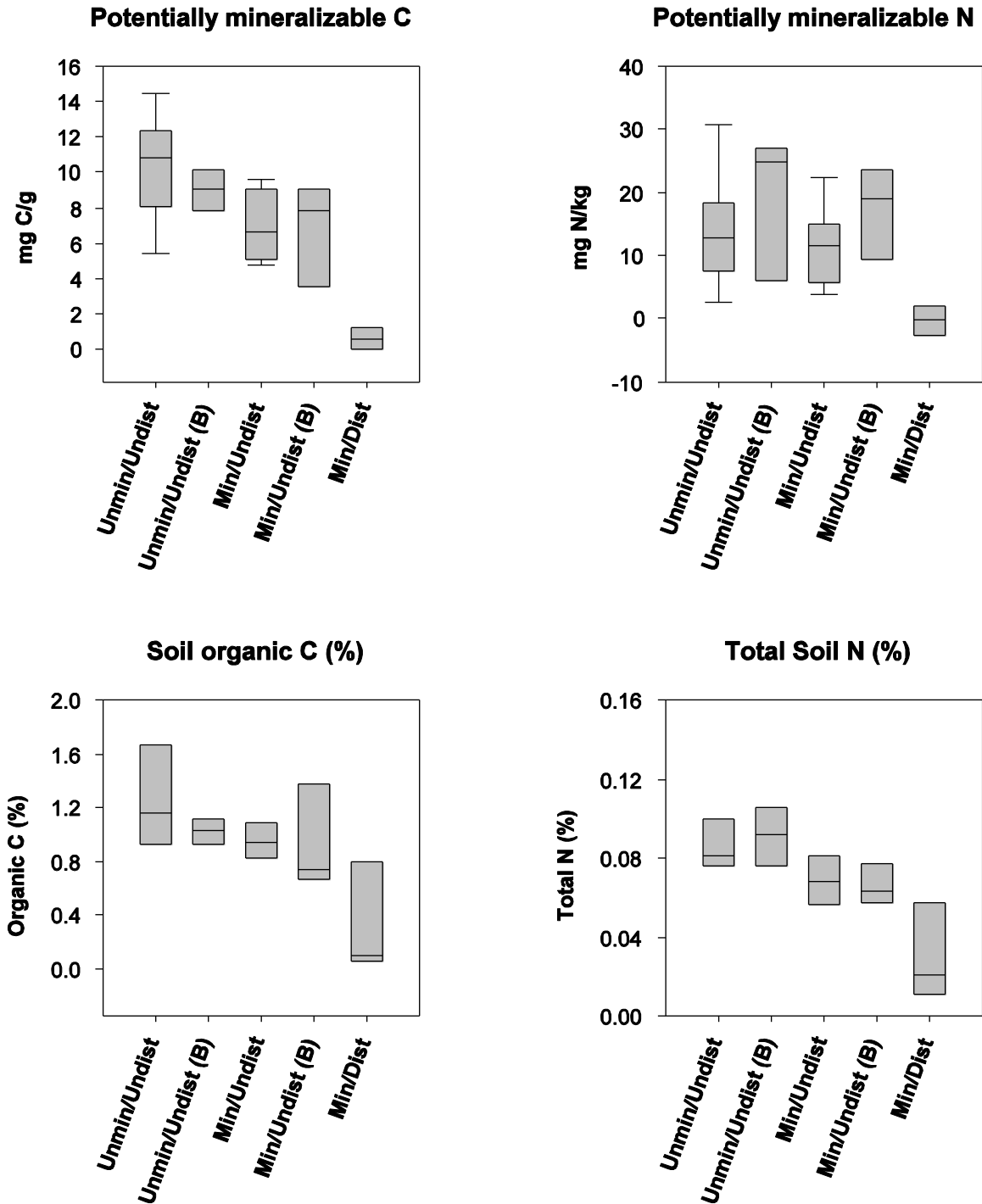
Figure 23. Buckingham study area, north-central, Nevada: Soil microbial data (Mineralizeable C and N, Organic C, Total N) across the study-design levels. Unmin/Undist, unmineralized/undisturbed soils; Min/Undist, mineralized/undisturbed soils; Min/Dist, mineralized/disturbed (waste-rock and tailings piles); (B), samples taken between shrub canopies (Min/Dist samples were also taken between shrub canopies).
