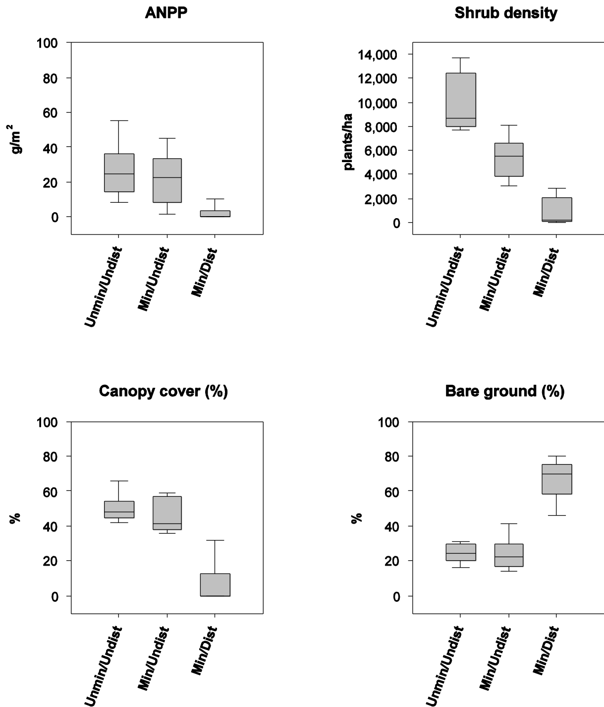
Figure 30. Buckingham study area, north-central, Nevada: Selected vegetation data (Aboveground net primary productivity (ANPP), Shrub density, Canopy cover, Bare ground) across the study-design levels. Unmin/Undist, unmineralized/undisturbed soils; Min/Undist, mineralized/undisturbed soils; Min/Dist, mineralized/disturbed (waste-rock and tailings piles).
