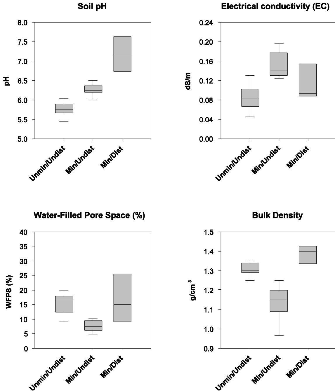
Figure 8. Red Hills study area, Tuolumne County, Calif.: Selected soil physical and chemical data (Soil pH, Electrical conductivity, Water-filled pore space (WFPS), and Bulk density) across the study-design levels. Unmin/Undist, unmineralized/undisturbed (serpentinite soils); Min/Undist, mineralized/undisturbed (andesite soils); Min/Dist, mineralized/disturbed (waste-rock and tailings piles); dS = decisiemens.
