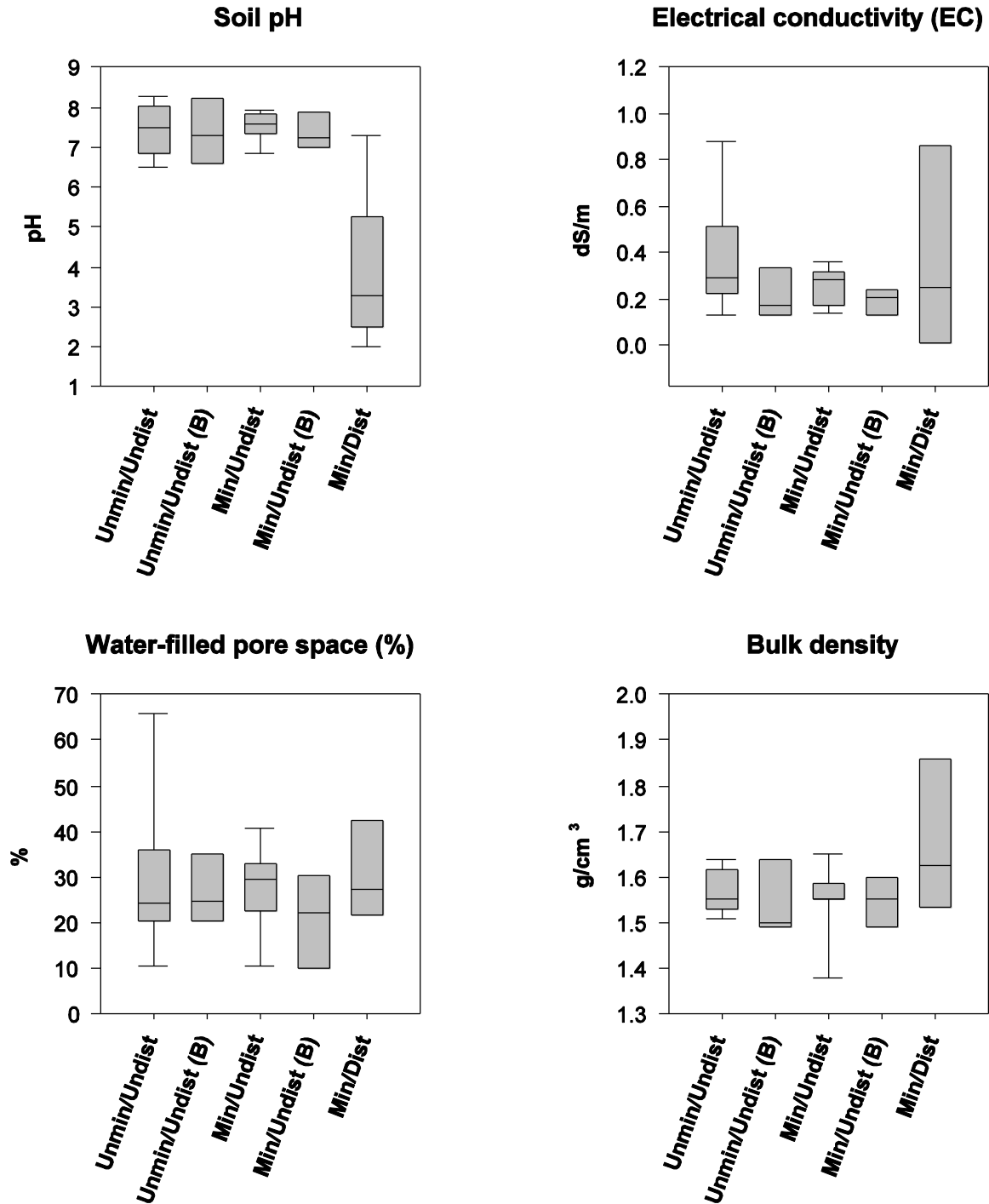
Figure 25. Buckingham study area, north-central, Nevada: Selected soil chemical and physical data (Soil pH, Electrical conductivity, Water-filled pore space (WFPS), Bulk density) across the study-design levels. Unmin/Undist, unmineralized/undisturbed soils; Min/Undist, mineralized/undisturbed soils; Min/Dist, mineralized/disturbed (waste-rock and tailings piles); (B), samples taken between shrub canopies (Min/Dist samples were also taken between shrub canopies); dS = decisiemens.
