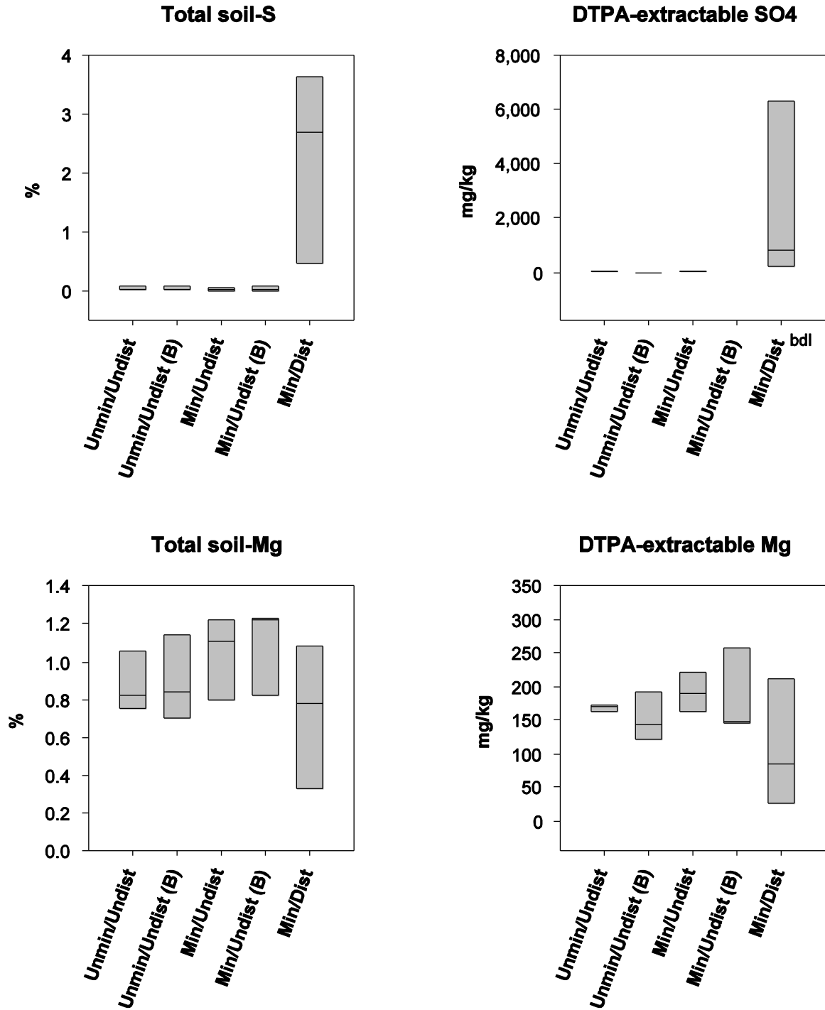
Figure 27. Buckingham study area, north-central, Nevada: Selected soil macronutrient data (Total and DTPA-extractable S and Mg) across the study-design levels. Unmin/Undist, unmineralized/undisturbed soils; Min/Undist, mineralized/undisturbed soils; Min/Dist, mineralized/disturbed (waste-rock and tailings piles); (B), samples taken between shrub canopies (Min/Dist samples were also taken between shrub canopies); bdl, below detection limit; SO 4 , sulfate.
