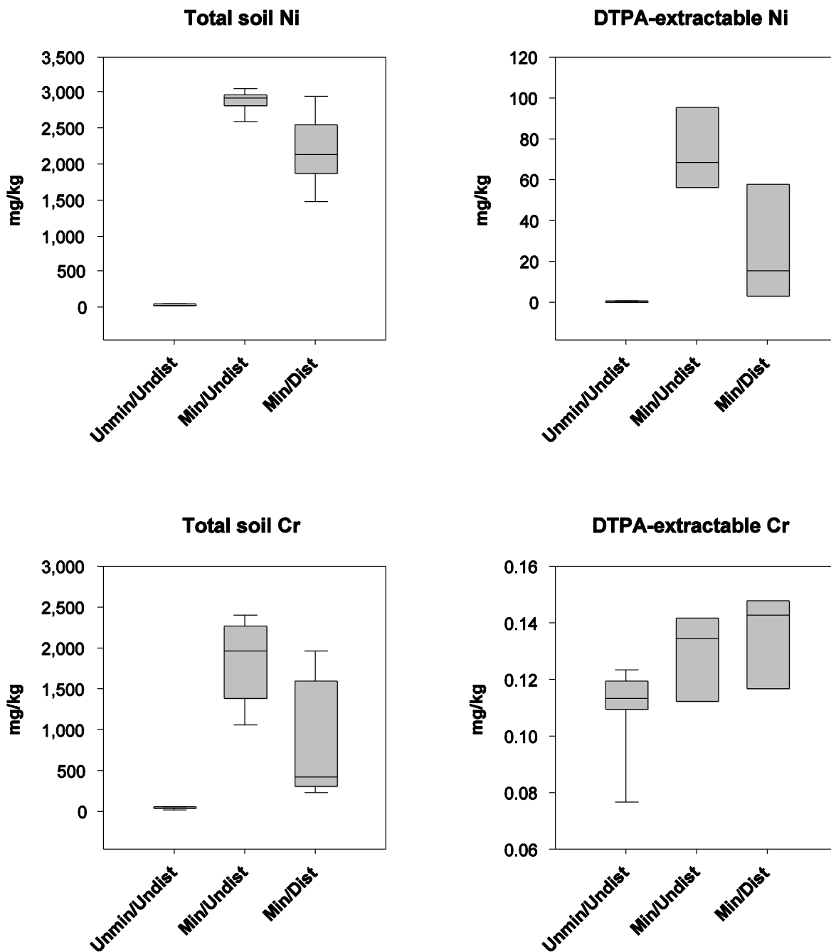
Figure 11. Red Hills study area, Tuolumne County, Calif.: Selected soil trace metals (Total and DTPA-extractable Ni and Cr) across the study-design levels. Unmin/Undist, unmineralized/undisturbed (serpentine soils); Min/Undist, mineralized/undisturbed (andesite soils); Min/Dist, mineralized/disturbed (waste-rock and tailings piles).
