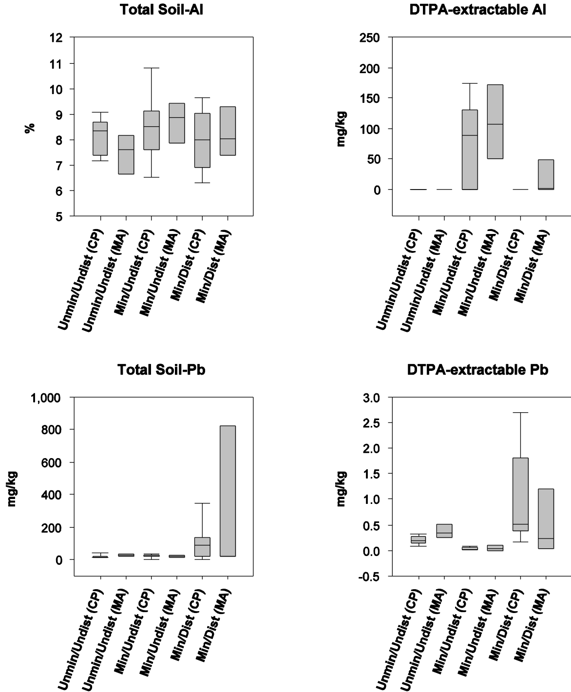
Figure 19. Quartz-alunite study sites: Selected soil metal data (Total and DTPA-extractable Al and Pb) across the study-design levels. Unmin/Undist, unmineralized/undisturbed (andesite soils); Min/Undist = mineralized/undisturbed (quartz-alunite soils); Min/Dist = mineralized/disturbed (waste-rock and tailings piles); CP, Castle Peak; MA, Masonic.
