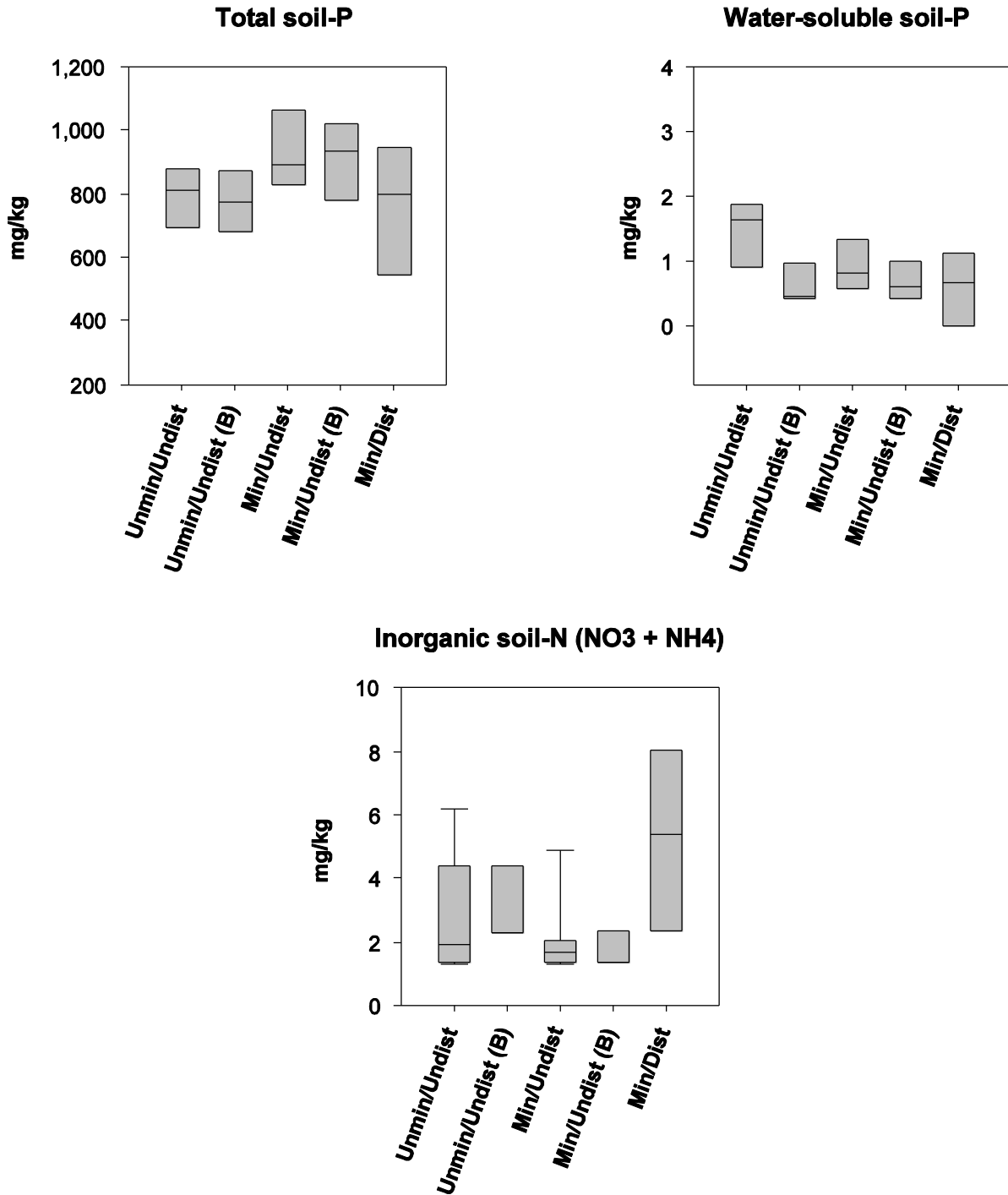
Figure 26. Buckingham study area, north-central, Nevada: Selected soil macronutrient data (Total and Water-soluble P, Inorganic N) across the study-design levels. Unmin/Undist, unmineralized/undisturbed soils; Min/Undist, mineralized/undisturbed soils; Min/Dist, mineralized/disturbed (waste-rock and tailings piles); (B), samples taken between shrub canopies (Min/Dist samples were also taken between shrub canopies); NO 3 , nitrate; NH 4 , ammonium.
