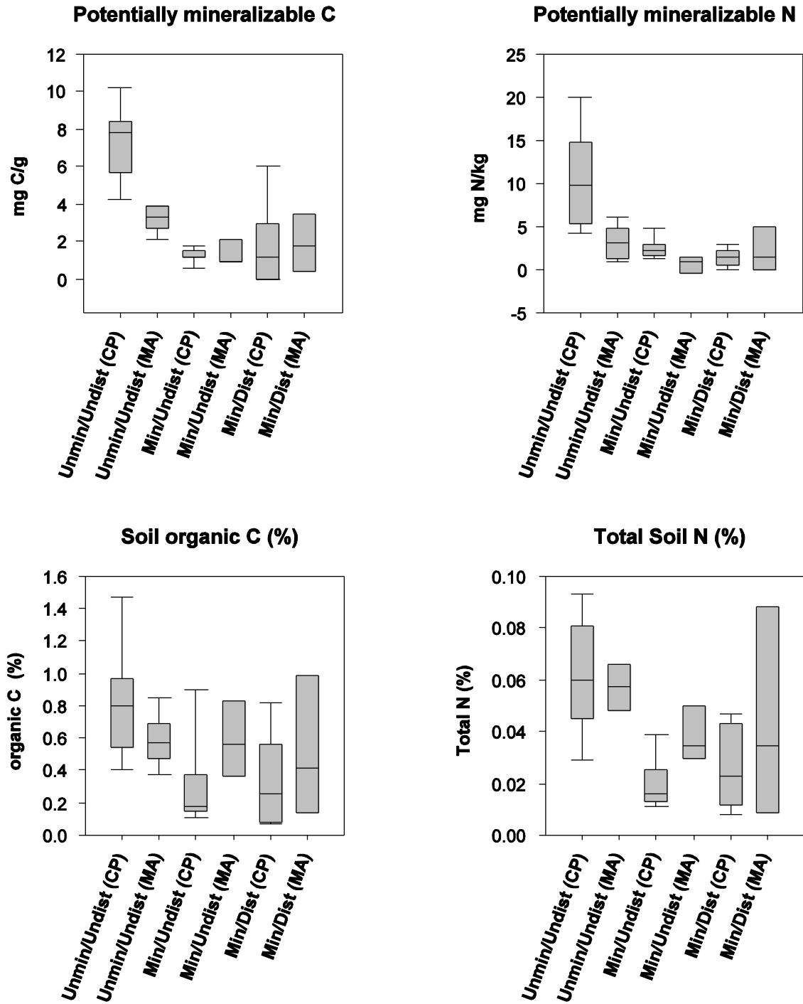
Figure 14. Quartz-alunite study sites: Soil microbial data (Mineralizeable C and N, Organic C, and Total N) across the study-design levels. Unmin/Undist, unmineralized/undisturbed (andesite soils); Min/Undist, mineralized/undisturbed (quartz-alunite soils); Min/Dist, mineralized/disturbed (waste-rock and tailings piles); CP, Castle Peak; MA, Masonic.
