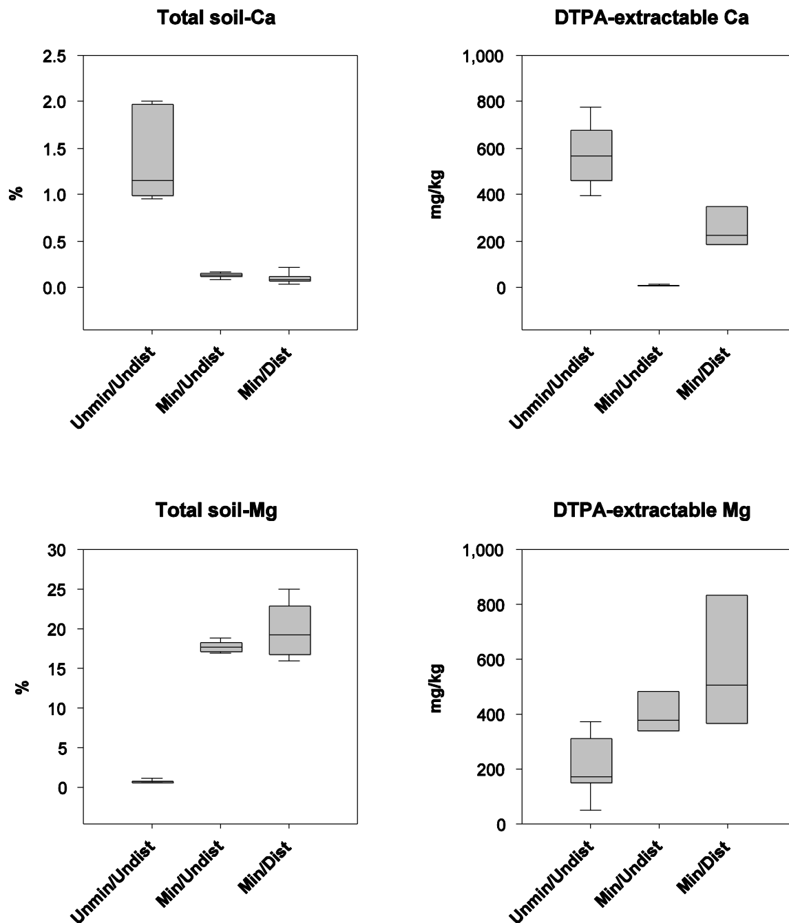
Figure 9. Red Hills study area, Tuolumne County, Calif.: Selected soil macronutrient data (Total and DTPA-extractable Ca and Mg) across the study-design levels. Unmin/Undist, unmineralized/undisturbed (serpentinite soils); Min/Undist, mineralized/undisturbed (andesite soils); Min/Dist, mineralized/disturbed (waste-rock and tailings piles).
