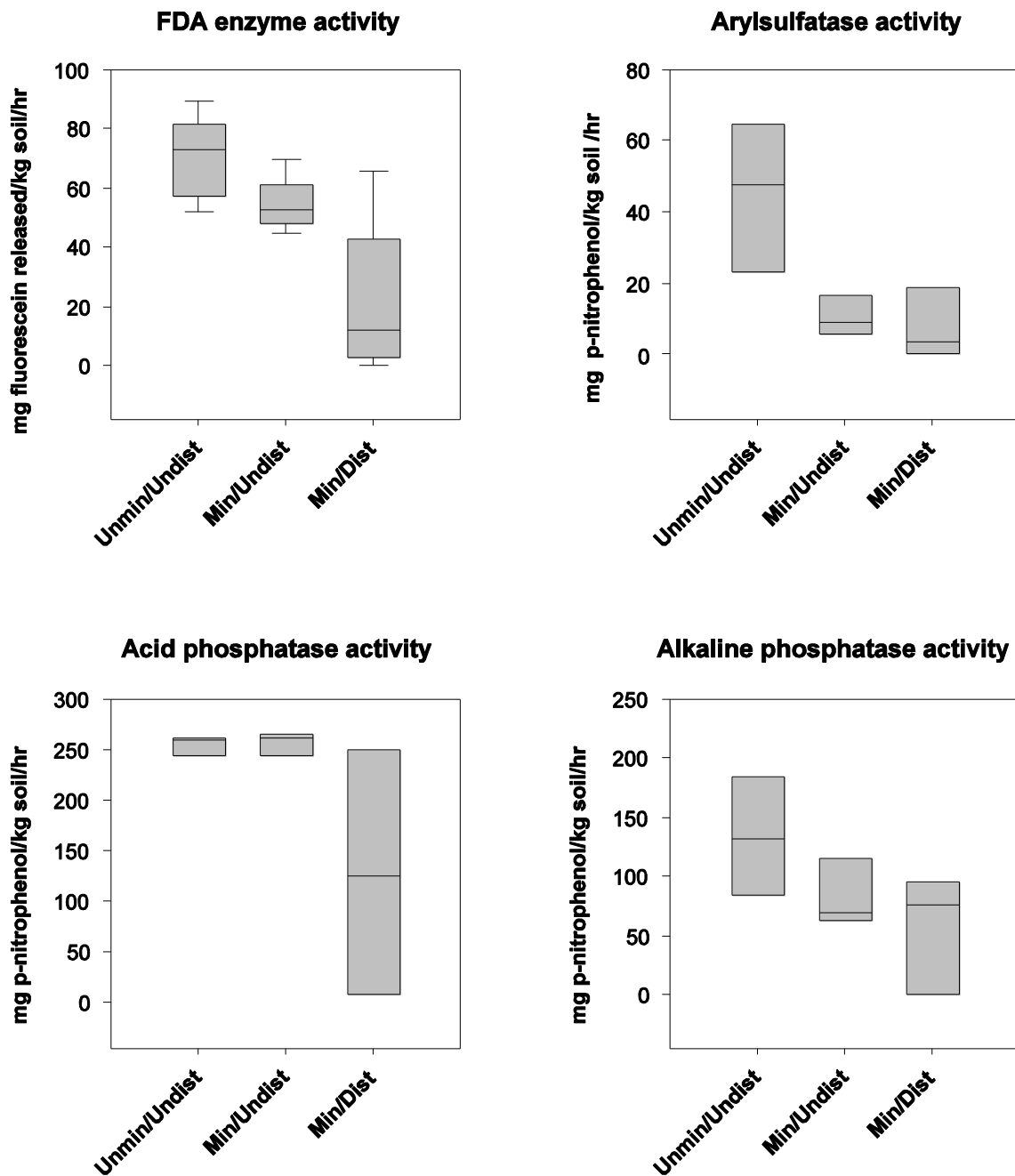
Figure 5. Red Hills study area, Tuolumne County, Calif.: Soil microbial data (Enzyme activity) across the study-design levels. Unmin/Undist, unmineralized/undisturbed (serpentinite soils); Min/Undist, mineralized/undisturbed (andesite soils); Min/Dist = mineralized/disturbed (waste-rock and tailings piles); FDA, Fluorescein diacetate.
