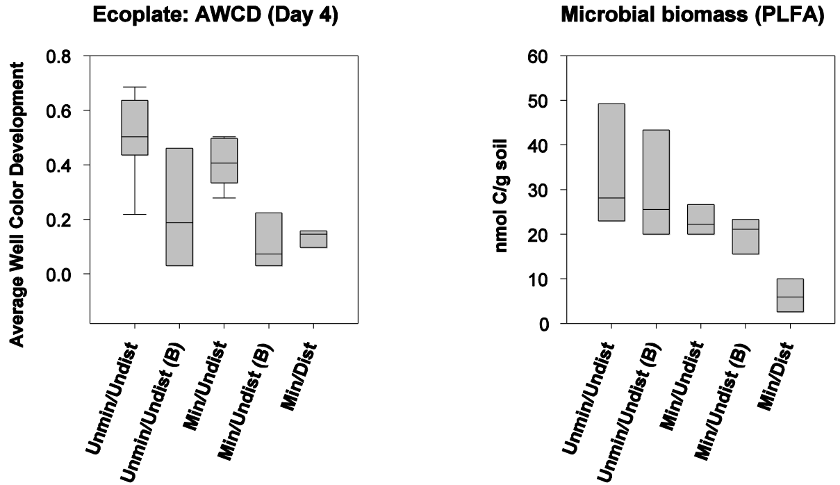
Figure 24. Buckingham study area, north-central, Nevada: Soil microbial data (Ecoplate AWCD, Microbial biomass (PLFA)) across the study-design levels. Unmin/undist, unmineralized/undisturbed soils; Min/Undist, mineralized/undisturbed soils; Min/Dist, mineralized/disturbed (waste-rock and tailings piles). (B), samples taken between shrub canopies (Min/Dist samples were also taken between shrub canopies); AWCD, Average well color development; PLFA, Phospholipid fatty acids.
