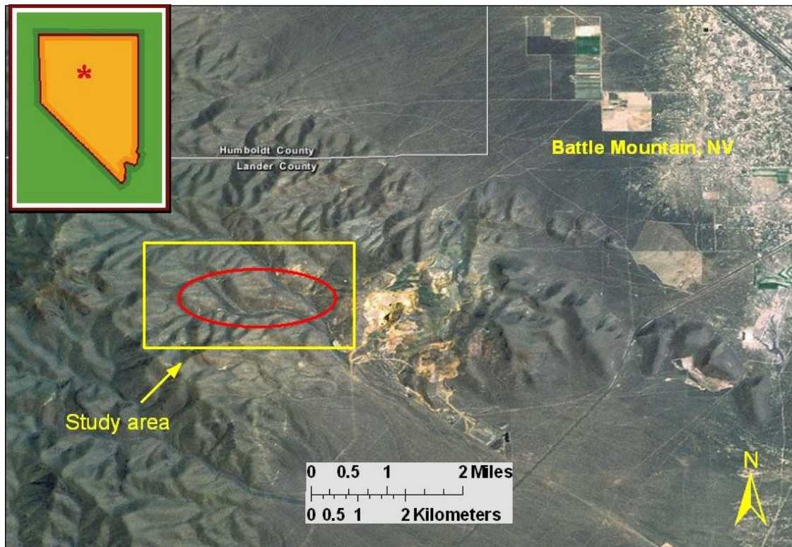
Figure 3. Buckingham (Mo/Cu porphyry) study area location map, north-central, Nevada. The mineralized area is depicted by the red oval within the overall study area.
