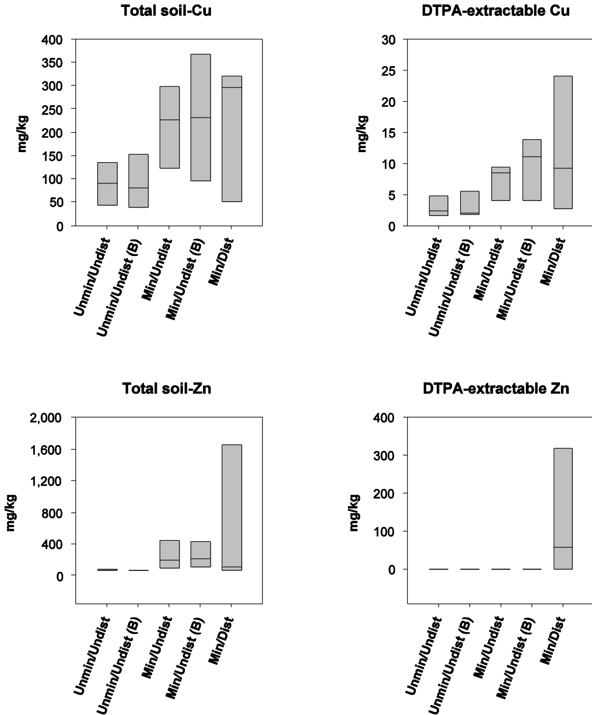
Figure 28. Buckingham study area, north-central, Nevada: Selected soil metal data (Total and DTPA-extractable Cu and Zn) across the study-design levels. Unmin/Undist, unmineralized/undisturbed soils; Min/Undist, mineralized/undisturbed soils; Min/Dist, mineralized/disturbed (waste-rock and tailings piles); (B), samples taken between shrub canopies (Min/Dist samples were also taken between shrub canopies).
