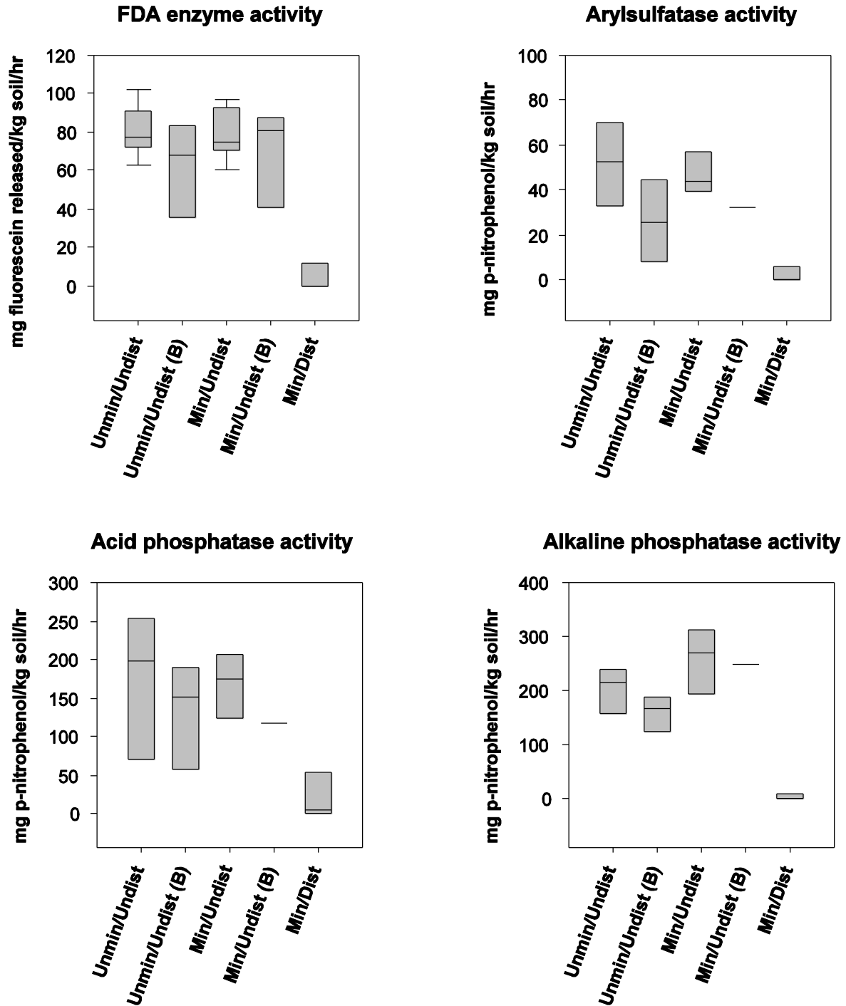
Figure 22. Buckingham study area, north-central, Nevada: Soil microbial data (Enzyme activity) across the study-design levels. Unmin/Undist, unmineralized/undisturbed soils; Min/Undist, mineralized/undisturbed soils; Min/Dist, mineralized/disturbed (waste-rock and tailings piles); (B), samples taken between shrub canopies (Min/Dist samples were also taken between shrub canopies); FDA, Fluorescein diacetate.
