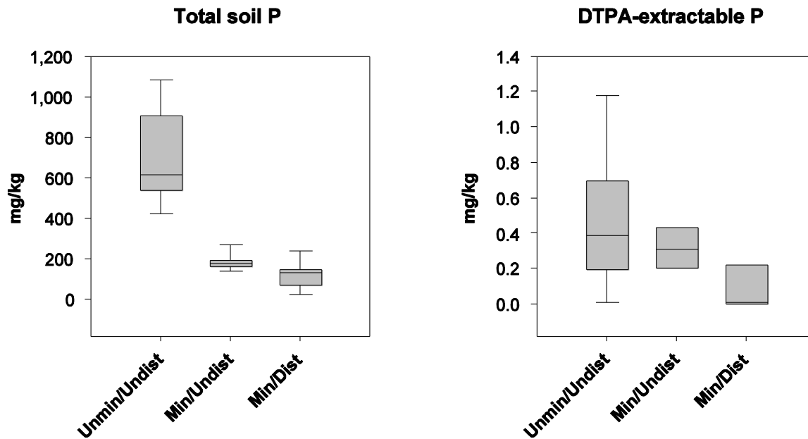
Figure 10. Red Hills study area, Tuolumne County, Calif.: Selected soil macronutrient data (Total and DTPA-extractable P) across the study-design levels. Unmin/Undist, unmineralized/undisturbed (serpentine soils); Min/Undist, mineralized/undisturbed (andesite soils); Min/Dist, mineralized/disturbed (waste-rock and tailings piles).
