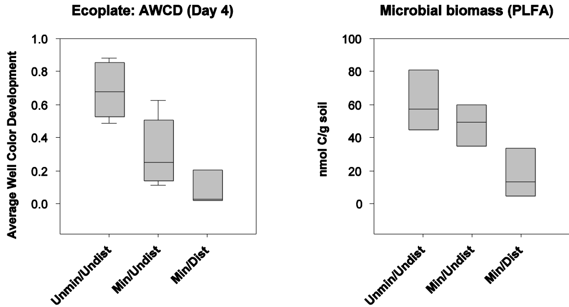
Figure 7. Red Hills study area, Tuolumne County, Calif.: Soil microbial data (Ecoplate AWCD, Microbial biomass (PLFA)) across the study-design levels. Unmin/Undist, unmineralized/undisturbed (serpentinite soils); Min/Undist, mineralized/undisturbed (andesite soils); Min/Dist, mineralized/disturbed (waste-rock and tailings piles), AWCD, Average well color development; PLFA, Phospholipid fatty acids.
