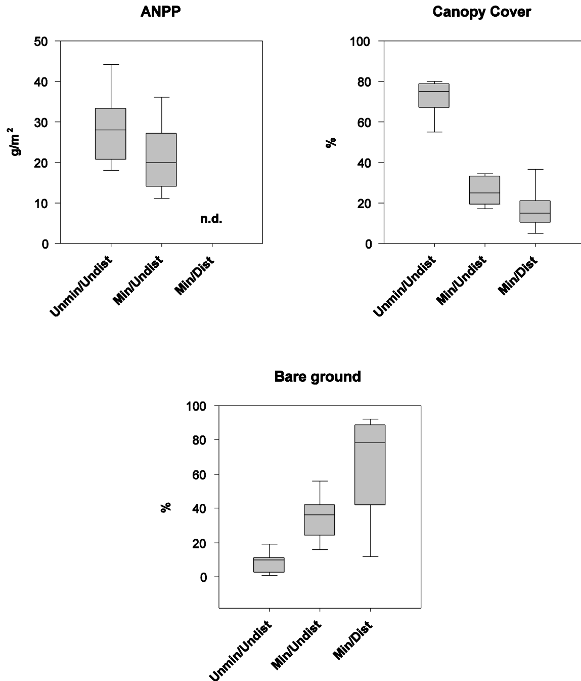
Figure 12. Red Hills study area, Tuolumne County, Calif.: Selected vegetation data (Aboveground net primary productivity (ANPP), Canopy cover, Bare ground) across the study-design levels. Unmin/Undist, unmineralized/undisturbed (serpentinite soils); Min/Undist, mineralized/undisturbed (andesite soils); Min/Dist, mineralized/disturbed (waste-rock and tailings piles); n.d., not determined.
