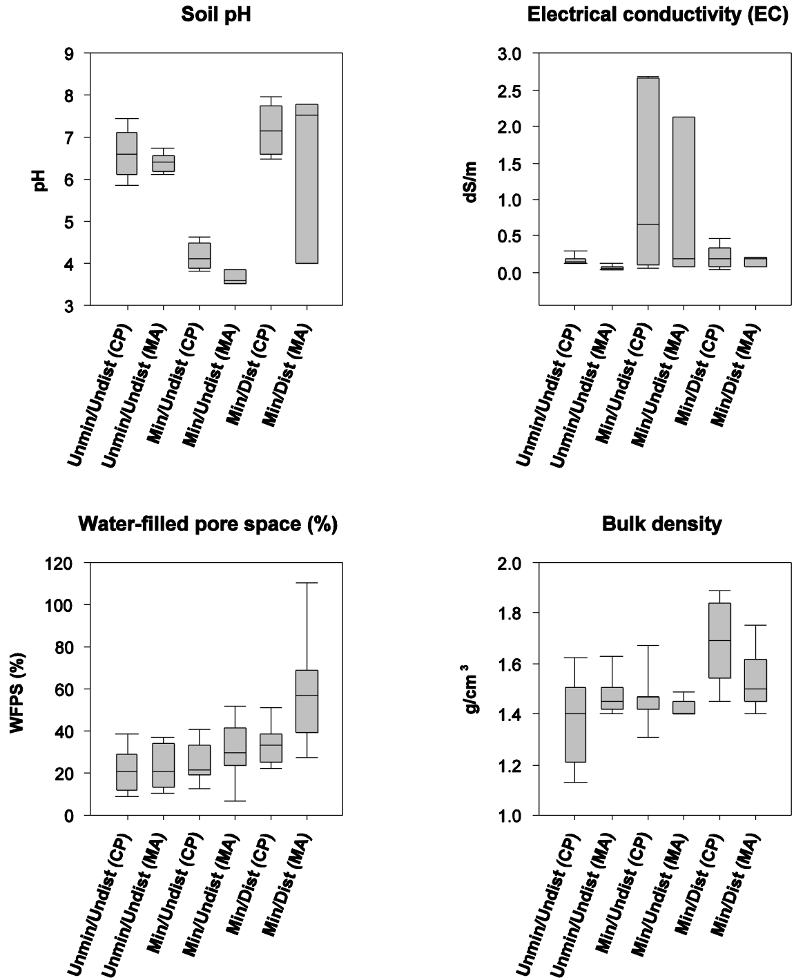
Figure 16. Quartz-alunite study sites: Selected soil chemical and physical data (Soil pH, Electrical conductivity, Water-filled pore space (WFPS), Bulk density) across the study-design levels. Unmin/Undist, unmineralized/undisturbed (andesite soils); Min/Undist, mineralized/undisturbed (quartz-alunite soils); Min/Dist, mineralized/disturbed (waste-rock and tailings piles); CP, Castle Peak; MA, Masonic; dS = decisiemens.
