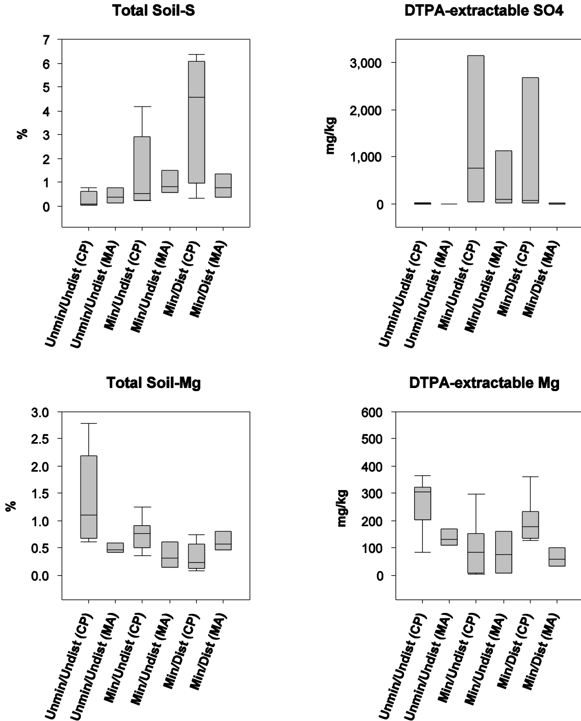
Figure 18. Quartz alunite study sites: Selected soil macronutrient data (Total and DTPA-extractable S and Mg) across the study-design levels. Unmin/Undist, unmineralized/undisturbed (andesite soils); Min/Undist, mineralized/undisturbed (quartz-alunite soils); Min/Dist, mineralized/disturbed (waste-rock and tailings piles); SO 4 , sulfate; CP, Castle Peak; MA, Masonic.
