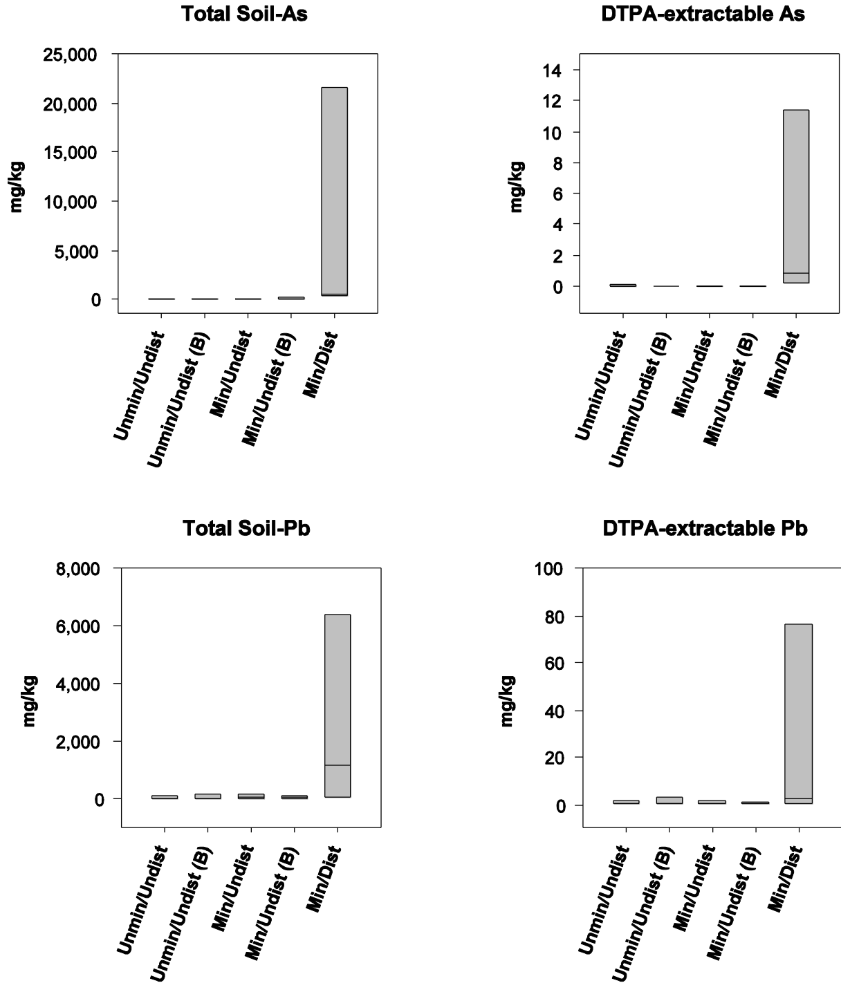
Figure 29. Buckingham study area, north-central, Nevada: Selected soil metal data (Total and DTPA-extractable As and Pb) across the study-design levels. Unmin/Undist, unmineralized/undisturbed soils; Min/Undist, mineralized/undisturbed soils; Min/Dist, mineralized/disturbed (waste-rock and tailings piles); (B), samples taken between shrub canopies (Min/Dist samples were also taken between shrub canopies).
