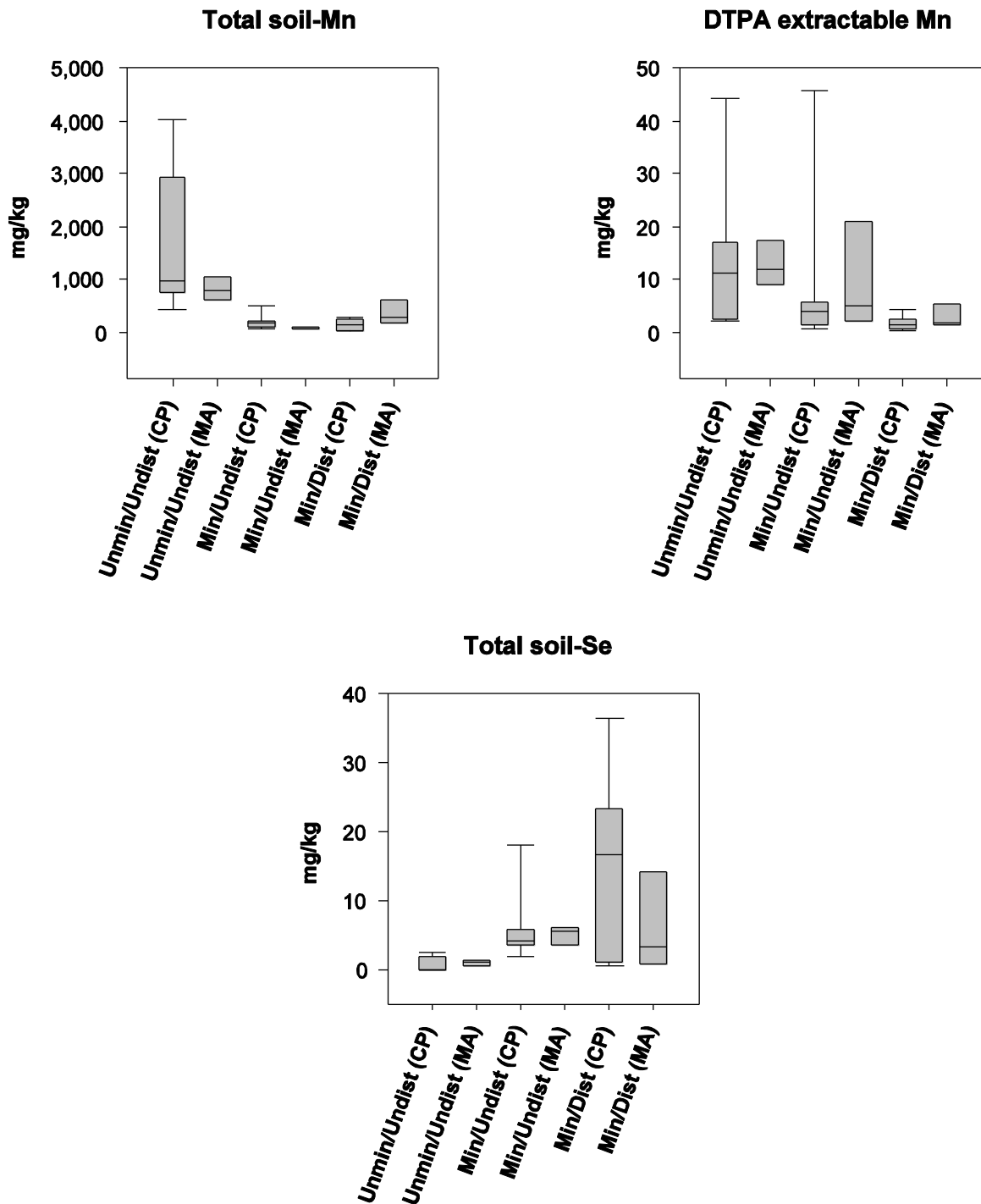
Figure 20. Quartz-alunite study sites: Selected soil metal data (Total and DTPA-extractable Mn and Total Se) across the study-design levels. Unmin/Undist = unmineralized/undisturbed (andesite soils); Min/Undist = mineralized/undisturbed (quartz-alunite soils); Min/Dist = mineralized/disturbed (waste-rock and tailings piles); CP, Castle Peak; MA, Masonic.
