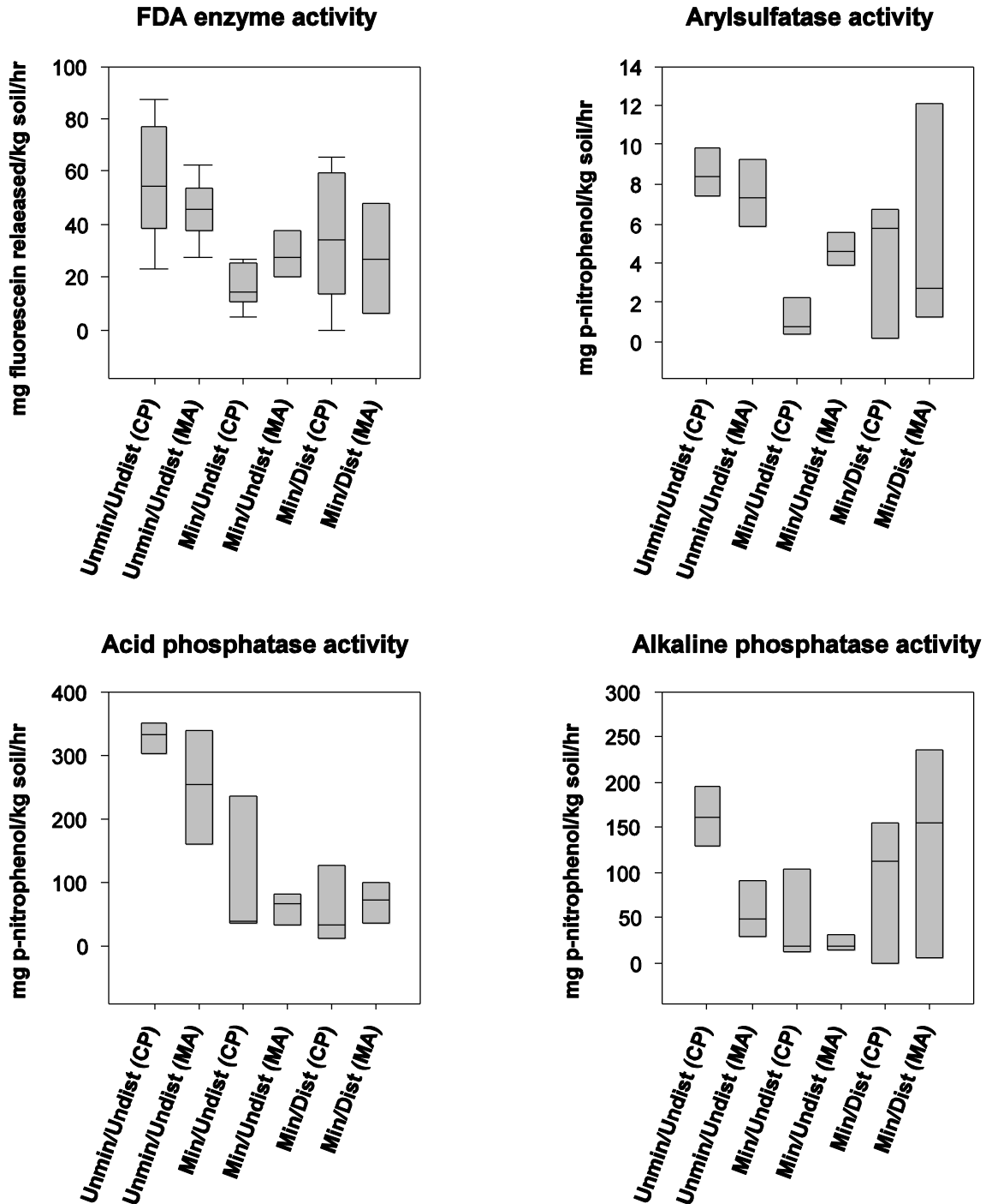
Figure 13. Quartz-alunite study sites: Soil microbial data (Enzyme activity) across the study-design levels. Unmin/Undist, unmineralized/undisturbed (andesite soils); Min/Undist, mineralized/undisturbed (quartz-alunite soils); Min/Dist, mineralized/disturbed (waste-rock and tailings piles), CP, Castle Peak; MA, Masonic; FDA, Fluorescein diacetate.
