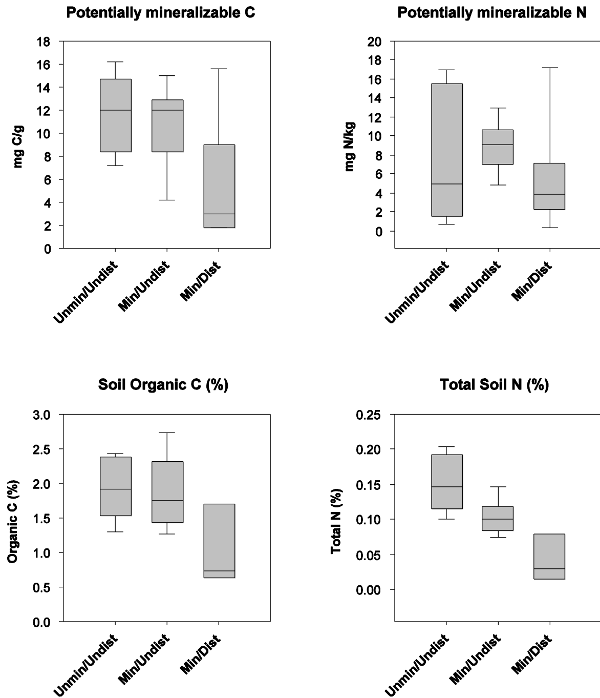
Figure 6. Red Hills study area, Tuolumne County, Calif.: Soil microbial data (Mineralizable C and N, Organic C, and Total N) across the study-design levels. Unmin/Undist, unmineralized/undisturbed (serpentinite soils); Min/Undist, mineralized/undisturbed (andesite soils); Min/Dist = mineralized/disturbed (waste-rock and tailings piles).
