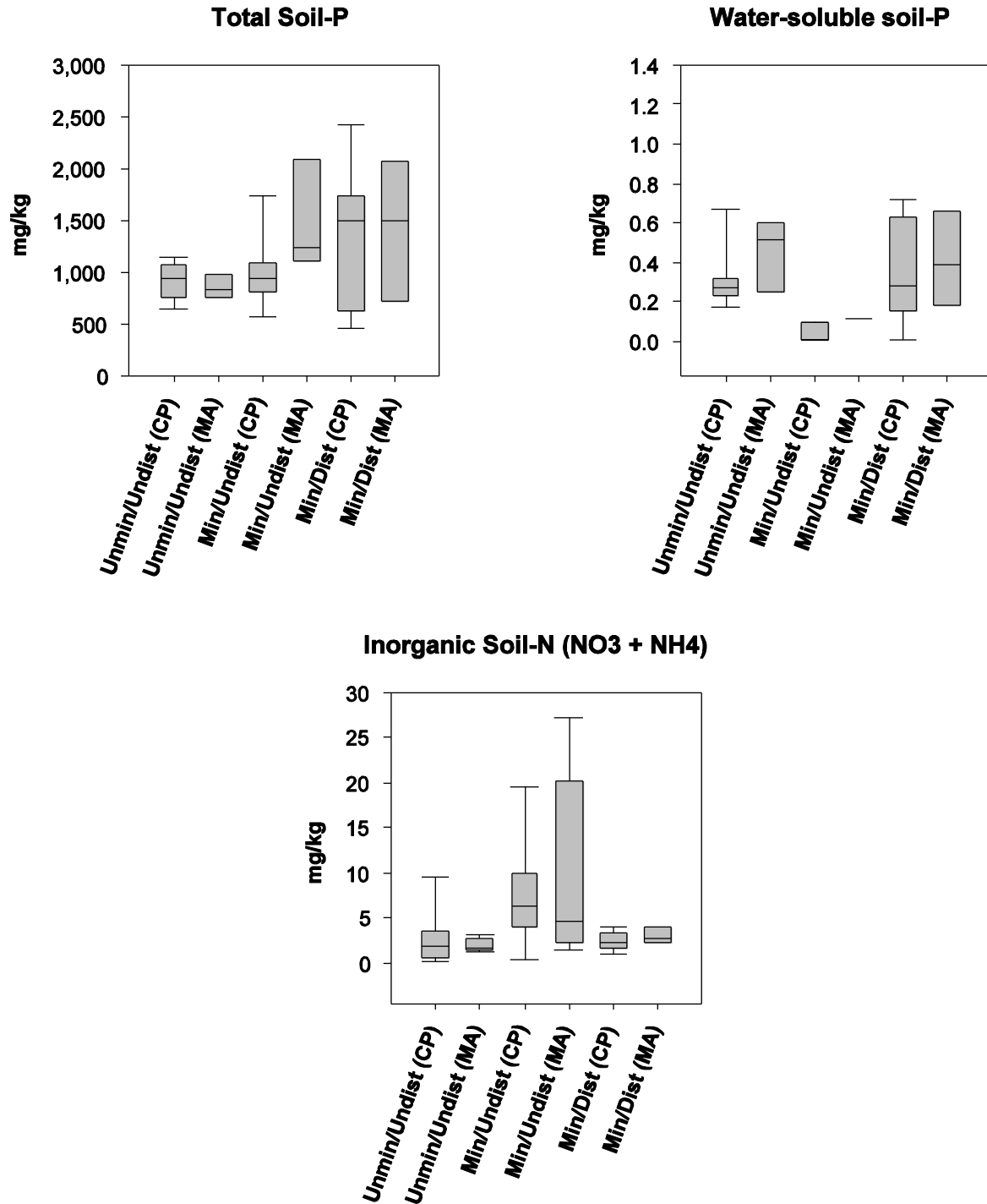
Figure 17. Quartz-alunite study sites: Selected soil macronutrient data (Total and Water-soluble P, and Inorganic N) across the study-design levels. Unmin/Undist, unmineralized/undisturbed (andesite soils); Min/Undist, mineralized/undisturbed (quartz-alunite soils); Min/Dist, mineralized/disturbed (waste-rock and tailings piles); NO 3 , nitrate; NH 4 , ammonium; CP, Castle Peak; MA, Masonic.
