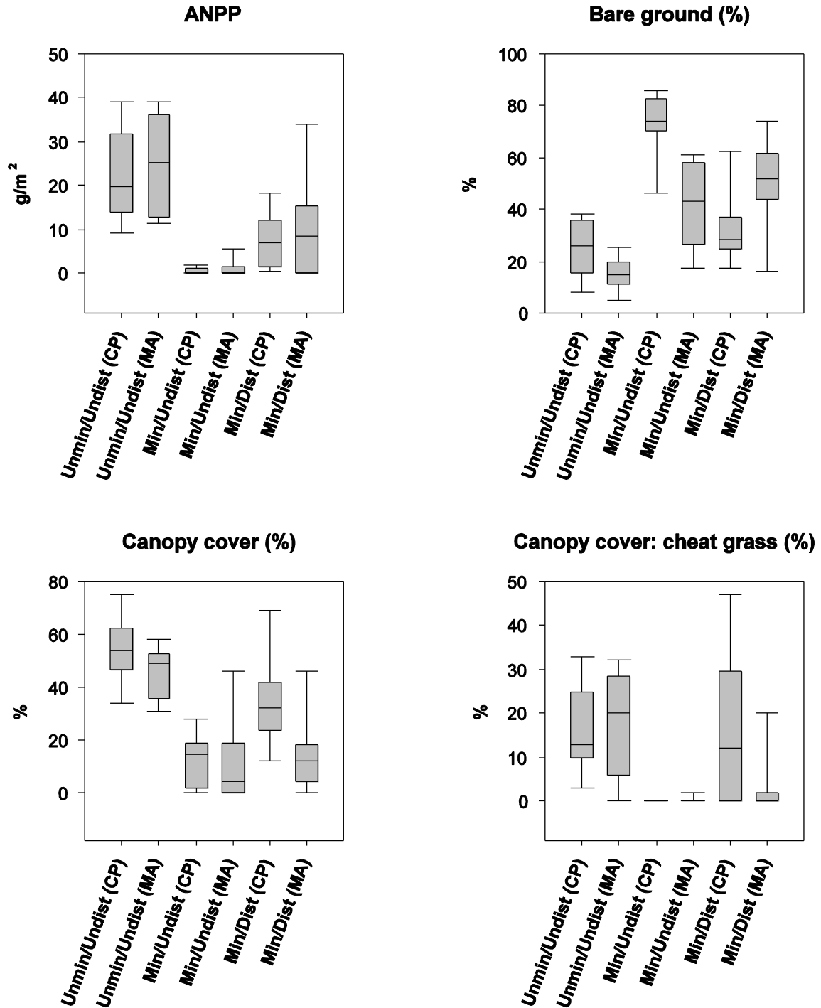
Figure 21. Quartz-alunite study sites: Selected vegetation data (Aboveground net primary productivity (ANPP), Bare ground, Canopy cover, Canopy cover comprised of cheat grass) across the study-design levels. Unmin/Undist, unmineralized/undisturbed (andesite soils); Min/Undist, mineralized/undisturbed (quartz-alunite soils); Min/Dist = mineralized/disturbed (waste-rock and tailings piles); CP, Castle Peak; MA, Masonic.
