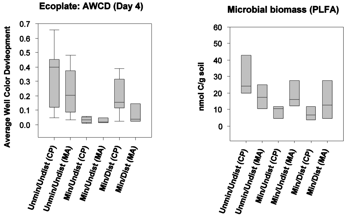
Figure 15. Quartz-alunite study sites: Soil microbial data (Ecoplate AWCD, Microbial biomass (PLFA)) across the study-design levels. Unmin/Undist, unmineralized/undisturbed (andesite soils); Min/Undist, mineralized/undisturbed (quartz-alunite soils); Min/Dist, mineralized/disturbed (waste-rock and tailings piles); CP, Castle Peak; MA, Masonic; AWCD, average well color development; PLFA, Phospholipid fatty acids.
