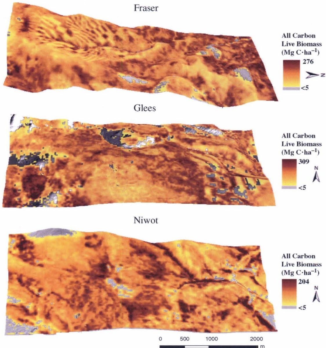
Fig. 2. Spatial map of all carbon in live biomass (Alllive) for the Fraser, Glees, and Niwot study sites using CCA explanatory variable regression equation (see Table 5).
