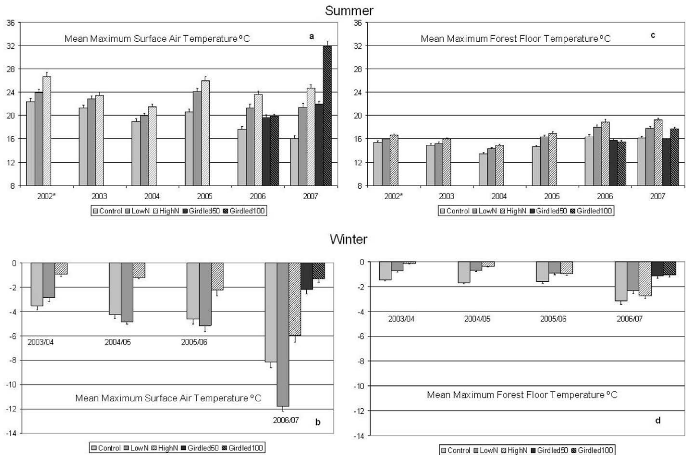
Figure 1.—Summer and winter mean maximum surface air and forest floor temperature in original control and N addition plots and new girdled plots in a high-elevation red spruce forest, Mount Ascutney, VT. Summer defined as June, July, and August and winter defined as December of previous year and January, February, and March of following year. *August 2002 only.
