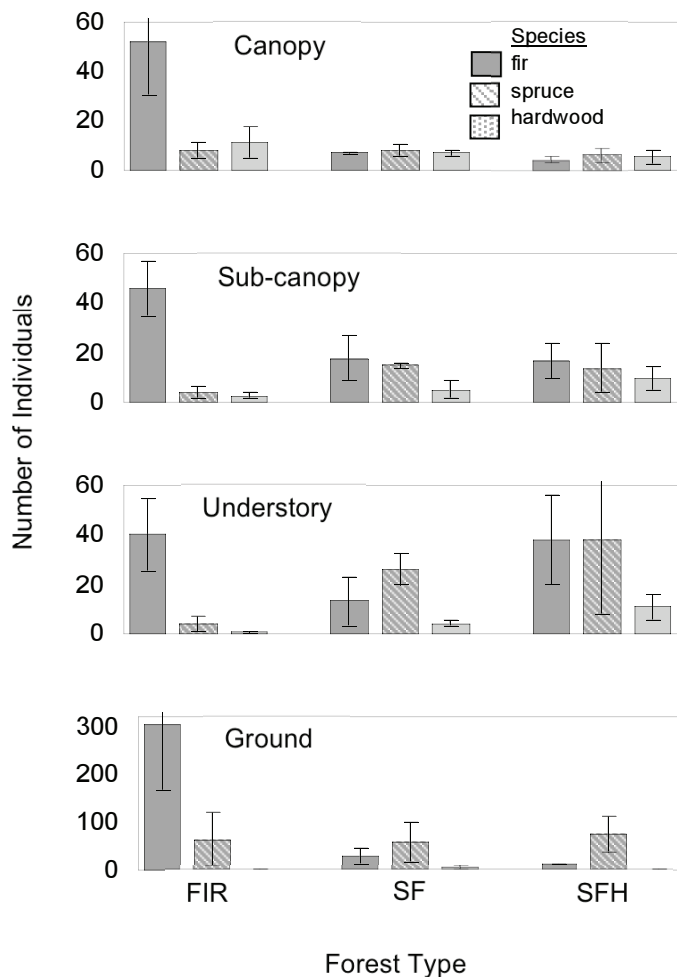
Figure 2.—Number of trees in each forest stratum by species and forest type. From 2008 census. Error bars represent standard error of the mean of three plots within each forest type. Area of three plots represents 1/40 acre. Forest Types: FIR; SF=Spruce-Fir; SFH=spruce-fir-hardwood.
