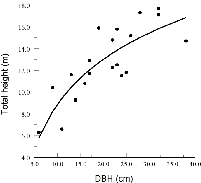
Figure 3.—Relationship of total height to d.b.h. for red spruce ranging in crown class from suppressed to dominant for 21 trees planted in the Pisgah National Forest from 1941-1943.
