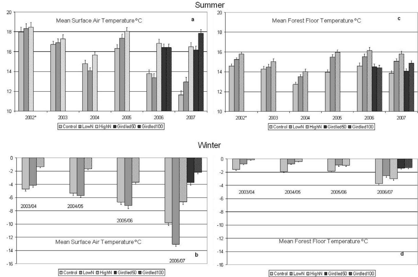
Figure 3.—Summer and winter mean surface air and forest floor temperature in original control and N addition plots and new girdled plots in a high-elevation red spruce forest, Mount Ascutney, VT. Summer defined as June, July, and August and winter defined as December of previous year and January, February, and March of following year. *August 2002 only.
