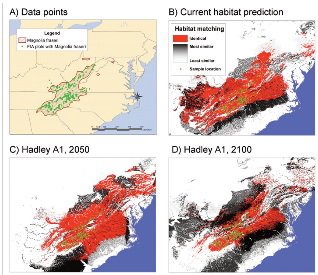
Figure 3.—Multivariate Spatio-Clustering predictions of current and future acceptable environmental conditions for mountain magnolia. The small green dots in all four subfigures depict the 562 Forest Inventory and Analysis plot locations that were used as training data (A) to predict the location of currently acceptable habitat conditions (B), which was in turn used to predict the locations of acceptable environmental conditions in 2050 (C) and 2100 (D) using the Hadley A1 (higher-emissions) scenario.
