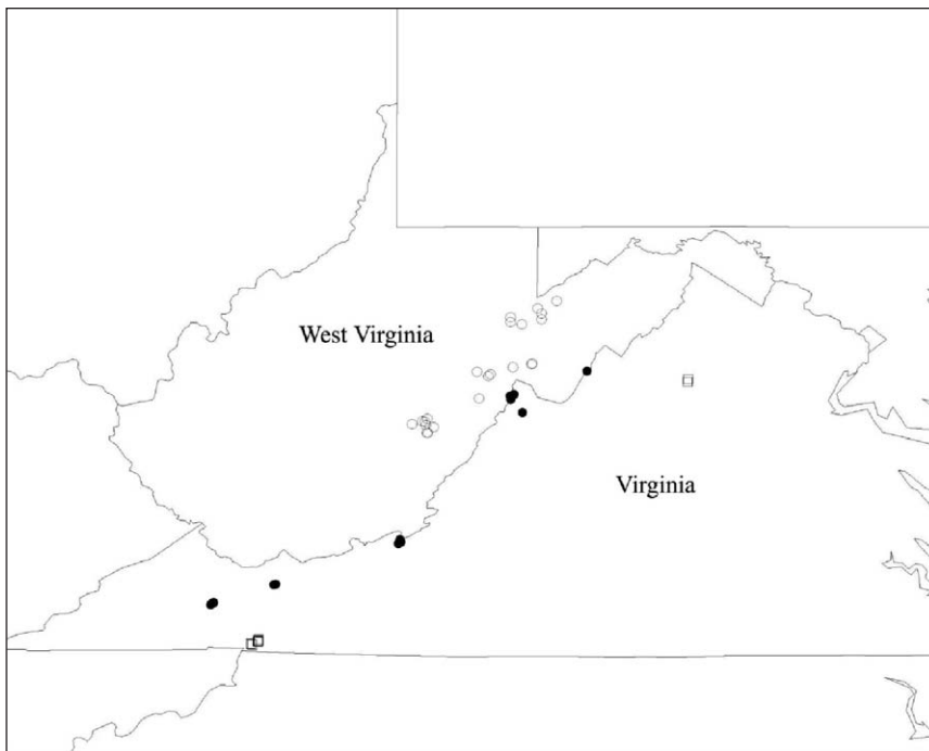
Figure 1.—General locations of stands sampled in southwestern Virginia and eastern central West Virginia. Note: squares = Blue Ridge, closed circles = Ridge and Valley, and open circles = Appalachian Plateau.
