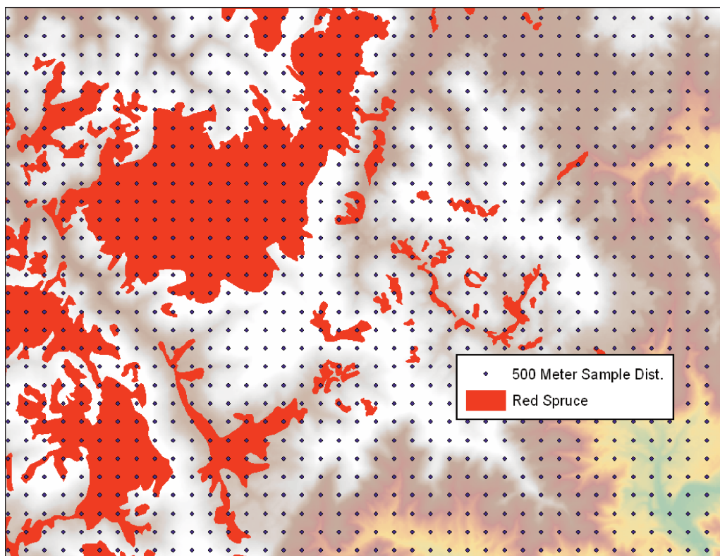
Figure 3.—Close-up illustration of 500-m point locations superimposed on the 1988 West Virginia red spruce layer. Background colors represent an elevation gradient ranging from 195 to 1,481 m (lowest to highest elevation: green, yellow, dark red, white).
