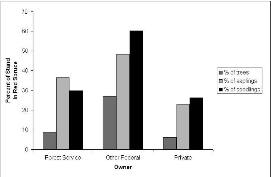
Figure 4.—Percent of tallied trees, saplings, and seedlings in red spruce in the maple/beech/birch forest-type group, North Carolina, Pennsylvania, Tennessee, Virginia, West Virginia, 2006.
