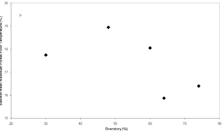
Figure 4b.—Relationship between estimated percent canopy cover and summer mean maximum forest floor temperature across the original and girdled plots.
