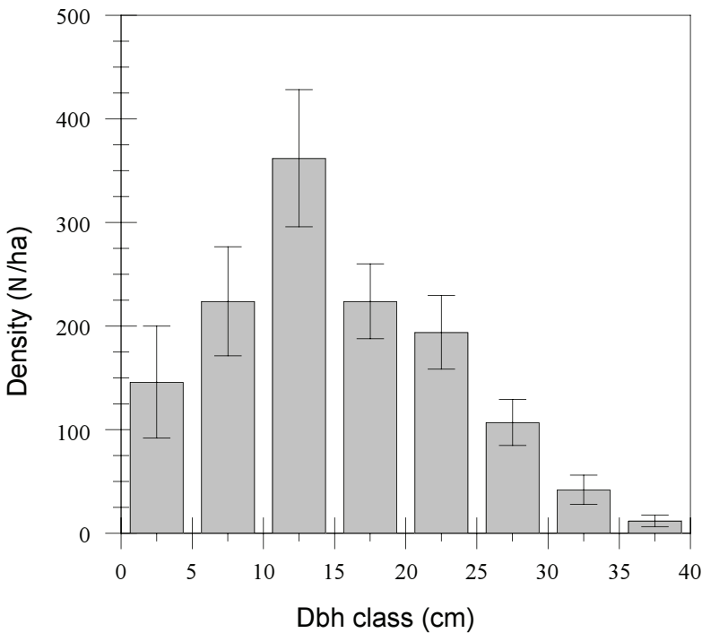
Figure 2.—Density ( \pm SE mean) of the red spruce component of a stand established by planting in the Pisgah National Forest from 1941-1943.
