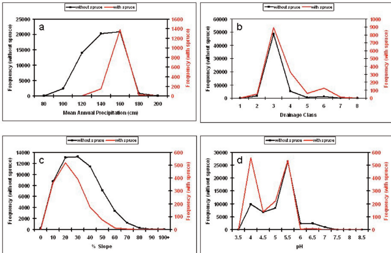
Figure 5.—Frequency distributions of mean annual precipitation (a), drainage class (b), percent slope (c), and soil pH (d) for spruce and non-spruce sites. See Table 1 for variable descriptions.
