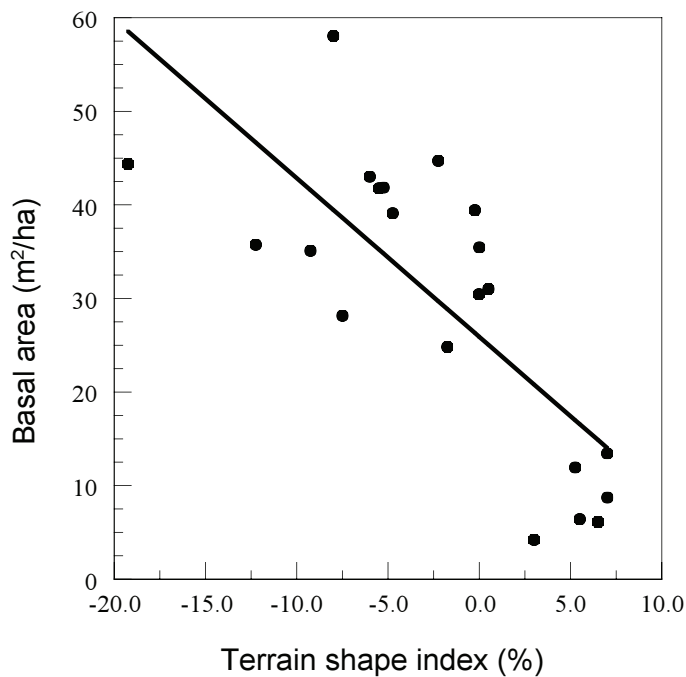
Figure 4.—Relationship of basal area of red spruce to terrain shape index for a planting established in the Pisgah National Forest from 1941-1943.
