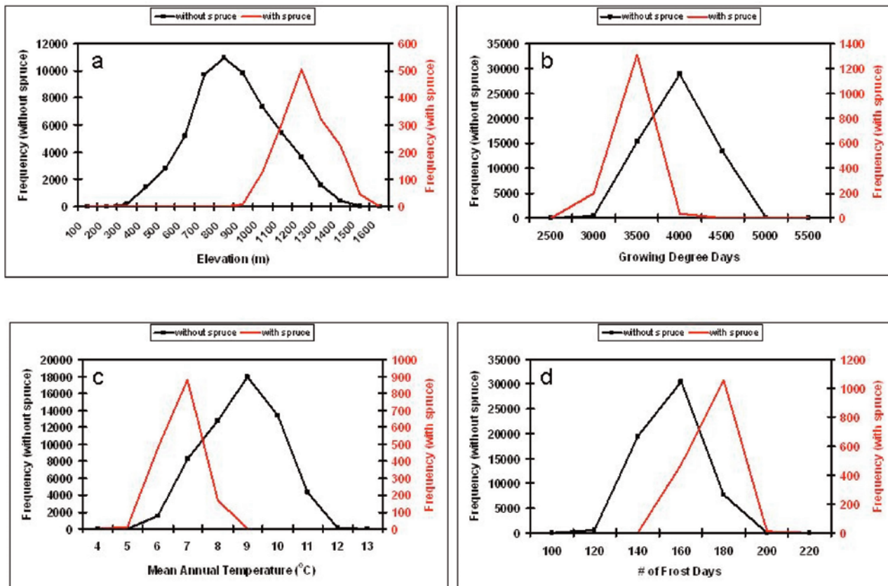
Figure 4.—Frequency distributions of elevation (a), growing degree days (b), mean annual temperature (c), and number of frost days (d) for spruce and non-spruce sites. See Table 1 for variable descriptions.
