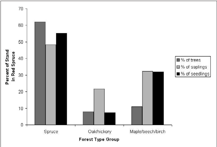
Figure 3.—Percent of tallied trees, saplings, and seedlings in red spruce by forest-type group, North Carolina, Pennsylvania, Tennessee, Virginia, West Virginia, 2006.
