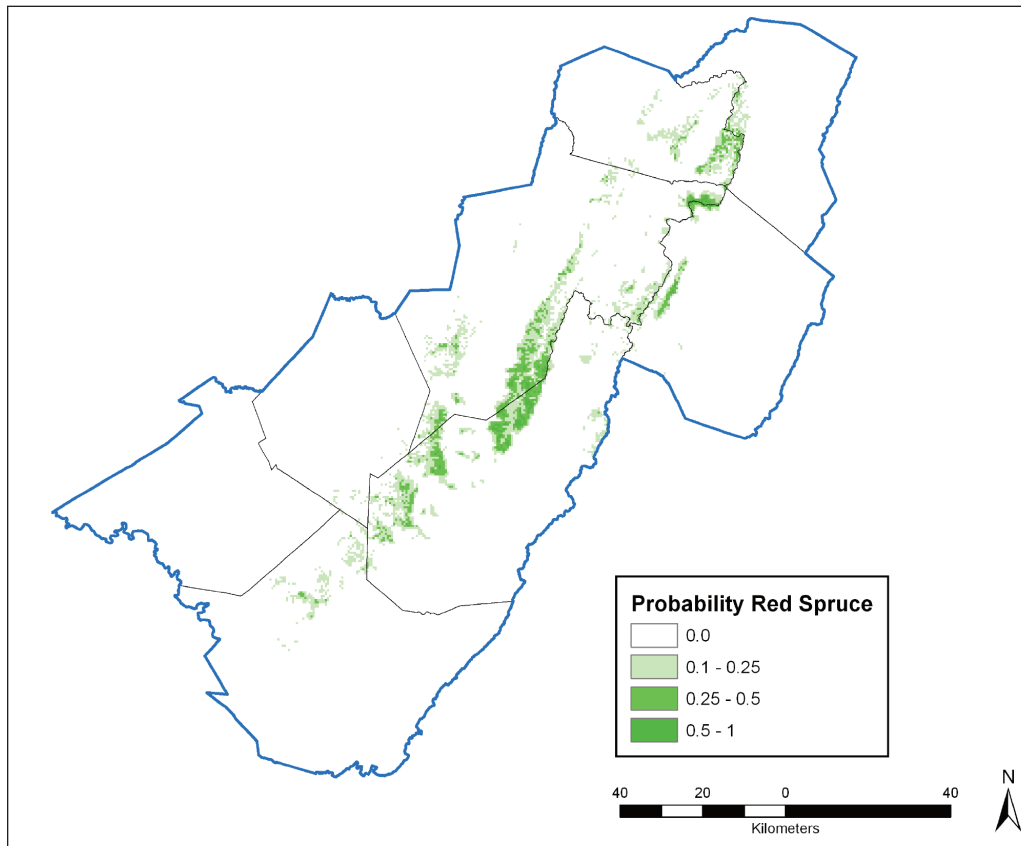
Figure 6.—Probability classes of red spruce occurrence based on the top four factors of stepwise logistical regression.
