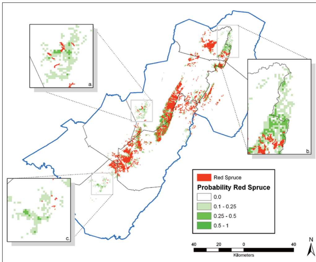
Figure 7.—Actual distribution of red spruce superimposed on probability map. The three inset boxes represent areas of high red spruce restoration potential based on the predictive model.
