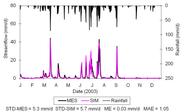
Fig. 6a. Measured and simulated daily streamflow in 2003. MES is measurement; SIM is simulation; STD is standard deviation; ME is mean error between simulation and observation; MAE is mean absolute error between simulation and observation.
