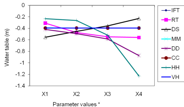
Fig. 3b. Sensitivity of water table to parameter inputs *: X1=10 , X2=30 , X3=50 and X4=70 \text{ m}^{1/3} \text{ s}^{-1} for Manning M (MM); 5, 25, 50 and 100 mm for detention storage (DS); 5, 25, 50 and 100 cm for Drainage depth (DD); 1 \times 10^{-6} , 4 \times 10^{-5} , 4 \times 10^{-4} and 5 \times 10^{-3} \text{ ms}^{-1} for horizontal hydraulic conductivity (HH); 5 \times 10^{-7} , 5 \times 10^{-6} , 5 \times 10^{-5} and 1 \times 10^{-4} \text{ ms}^{-1} for vertical hydraulic conductivity (VH); 30, 50, 70 and 90 cm for plant rooting depth (RT); 0.05, 0.2, 0.4 and 0.8 mm for coefficient of canopy interception (CC); 8 \times 10^{-6} , 8 \times 10^{-5} , 8 \times 10^{-4} and 1 \times 10^{-3} \text{ ms}^{-1} for infiltration rate (IFT).
