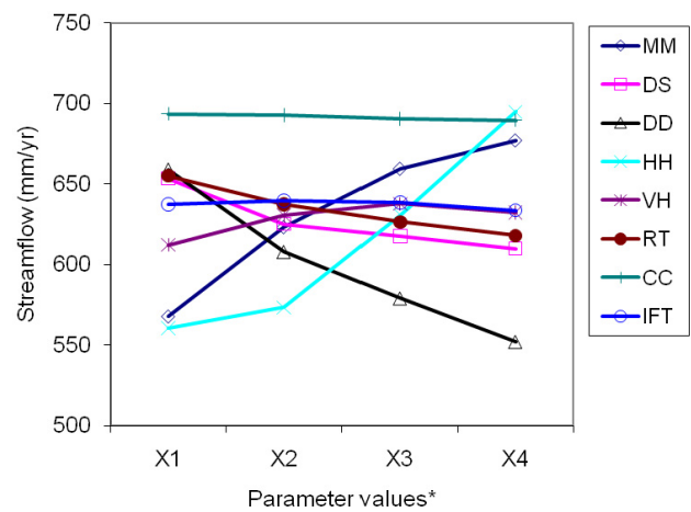
Fig. 3a. Sensitivity of streamflow to inputs *: X1=10 , X2=30 , X3=50 and X4=70 \text{ m}^{1/3} \text{ s}^{-1} for Manning M (MM); 5, 25, 50 and 100 mm for detention storage (DS); 5, 25, 50 and 100 cm for Drainage depth (DD); 1 \times 10^{-6} , 4 \times 10^{-5} , 4 \times 10^{-4} and 5 \times 10^{-3} \text{ ms}^{-1} for horizontal hydraulic conductivity (HH); 5 \times 10^{-7} , 5 \times 10^{-6} , 5 \times 10^{-5} and 1 \times 10^{-4} \text{ ms}^{-1} for vertical hydraulic conductivity (VH); 30, 50, 70 and 90 cm for plant rooting depth (RT); 0.05, 0.2, 0.4 and 0.8 mm for coefficient of canopy interception (CC); 8 \times 10^{-6} , 8 \times 10^{-5} , 8 \times 10^{-4} and 1 \times 10^{-3} \text{ ms}^{-1} for infiltration rate (IFT).
