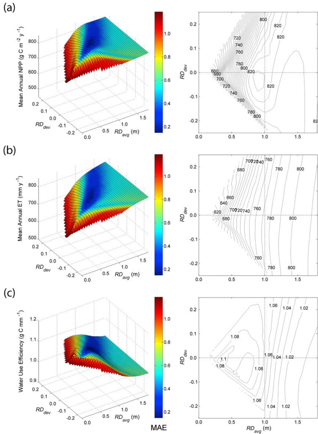
Figure 10. Three- and two-dimensional contour plots of long-term simulated (1941 ~ 2005) average annual (a) net primary productivity (NPP), (b) evapotranspiration (ET), and (c) water use efficiency (WUE) over sampled RD_{avg} and RD_{dev} under constant allocation strategy. The color bar represents MAE of simulated LAI (Figure 9a).
