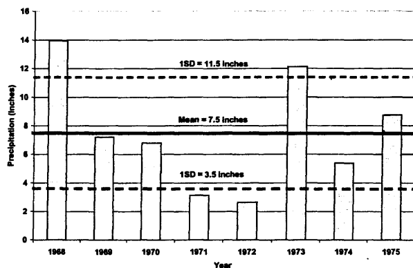
Figure 2. Precipitation for the December through April period at the Log Canyon recording precipitation gauge in the forest opening. The graph presents the average with the one standard deviation lines.
