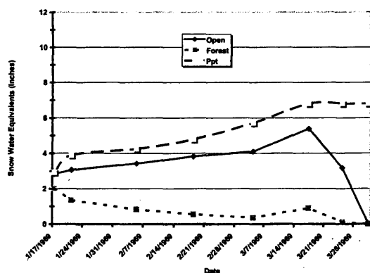
Figure 4A-D. Snowpack fluctuations in snow water equivalents for the forest opening and forest during the winters of 1969 (A), 1973 (B), 1974 (C), and 1975 (D). The accumulated precipitation from the Log Canyon gauge is shown.
