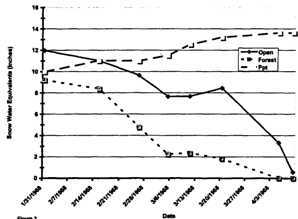
Figure 3. Snowpack fluctuations in snow water equivalents for the forest opening and forest during the winter of 1968. The accumulated precipitation from the Log Canyon gauge is shown.
