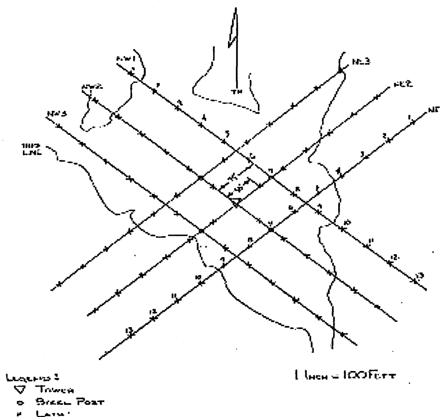
Figure 1. Map of the forest opening at Castle Creek West Fork and the layout of the snow survey lines. Survey points are 50 ft apart and parallel lines are 75 ft apart. The tree line is shown. The same design was used in the forested plot.
