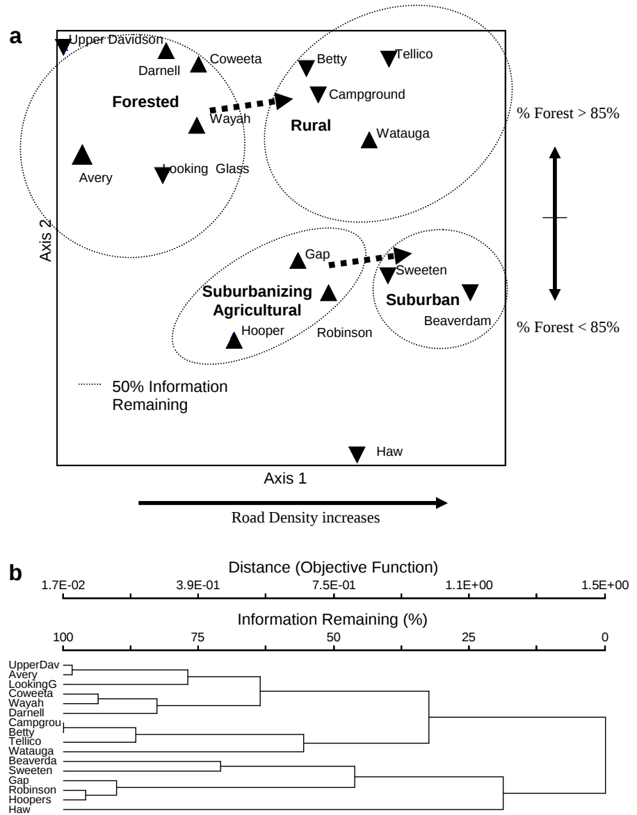
Fig. 5 Nonmetric multidimensional scaling ordination ( a ) and cluster analysis ( b ) results for fishes observed at 16 sites with comparable catchment size and outlet elevation. Dotted lines in a represent the 50% Information Remaining criterion
