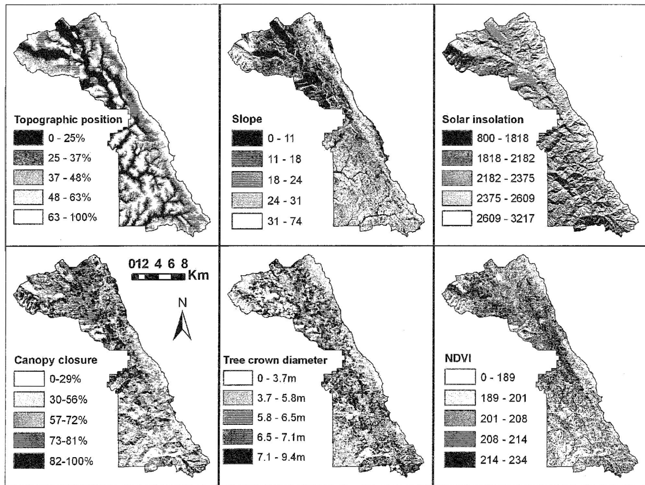
Figure 2. Maps of habitat characteristics used to evaluate resource selection by barred owls in the Eastern Cascade Mountains, Washington, USA, based on data collected from 2004 to 2006. Habitat characteristics are 1) topographic position, 2) slope, 3) solar radiation, 4) canopy closure, 5) overstory tree crown diameter, and 6) normalized difference vegetation index (NDVI).
