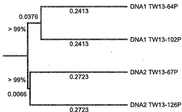
Fig. 3 UPGMA cluster analysis of UniFrac distances based upon the maximum-likelihood LSU tree obtained for the 456 clones. The taxon labels indicate the source soil DNA extract (1 vs. 2) and the pig-tagged primer used. Branch lengths from the UniFrac distance metric are given below or near branches, and jackknife support for the two nodes from 100 resampling runs are also shown. Note that the arrays of sequences obtained from the same soil sample with the different pig-tagged primers cluster together.
