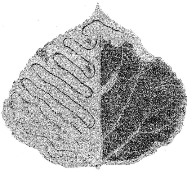
Fig. 1 Serpentine mines caused by Phyllocnistis populiella mining in a quaking aspen leaf
