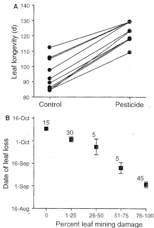
Fig. 5 Effect of leaf mining on date of leaf longevity. a The effect of pesticide treatment on the duration of leaf attachment, from the beginning of the study (1 June 2003) until leaf drop. Each symbol represents the mean of five leaves on a shoot; values for shoots within a single tree are connected by a line. b Mean ( \pm SEM) date that leaves were last observed attached to the tree at different levels of leaf mining damage. Numbers above symbols are sample sizes
