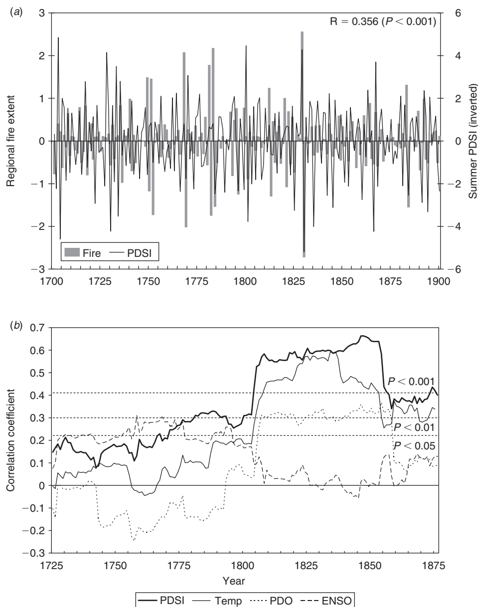
Fig. 5. (a) Pearson product moment correlation coefficients of first differences for regional fire occurrence and Palmer Drought Severity Index (PDSI) and (b) 50-year running correlation, plotted on the 26th year of the period, between fire occurrence, PDSI, summer temperature (TEMP), El Niño–Southern Oscillation (ENSO), and Pacific Decadal Oscillation (PDO). The PDSI values and corresponding correlation coefficients were inverted for presentation.
