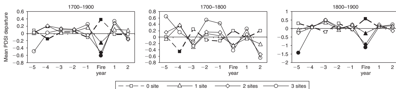
Fig. 4. Superposed epoch analysis (SEA) of reconstructed Palmer Drought Severity Index (PDSI) with non-fire years and fire years of different extent ( \geq 1 , \geq 2 or \geq 3 sites) in the southern Cascade Range, California, for the periods 1700–1800 and 1800–1900. There were too few fires to conduct an SEA for burns of larger extent (four or more sites burned). The analysis window includes up to 5 years before and 2 years after each fire or non-fire year. Values with filled symbols were statistically significant ( P < 0.05 ).
