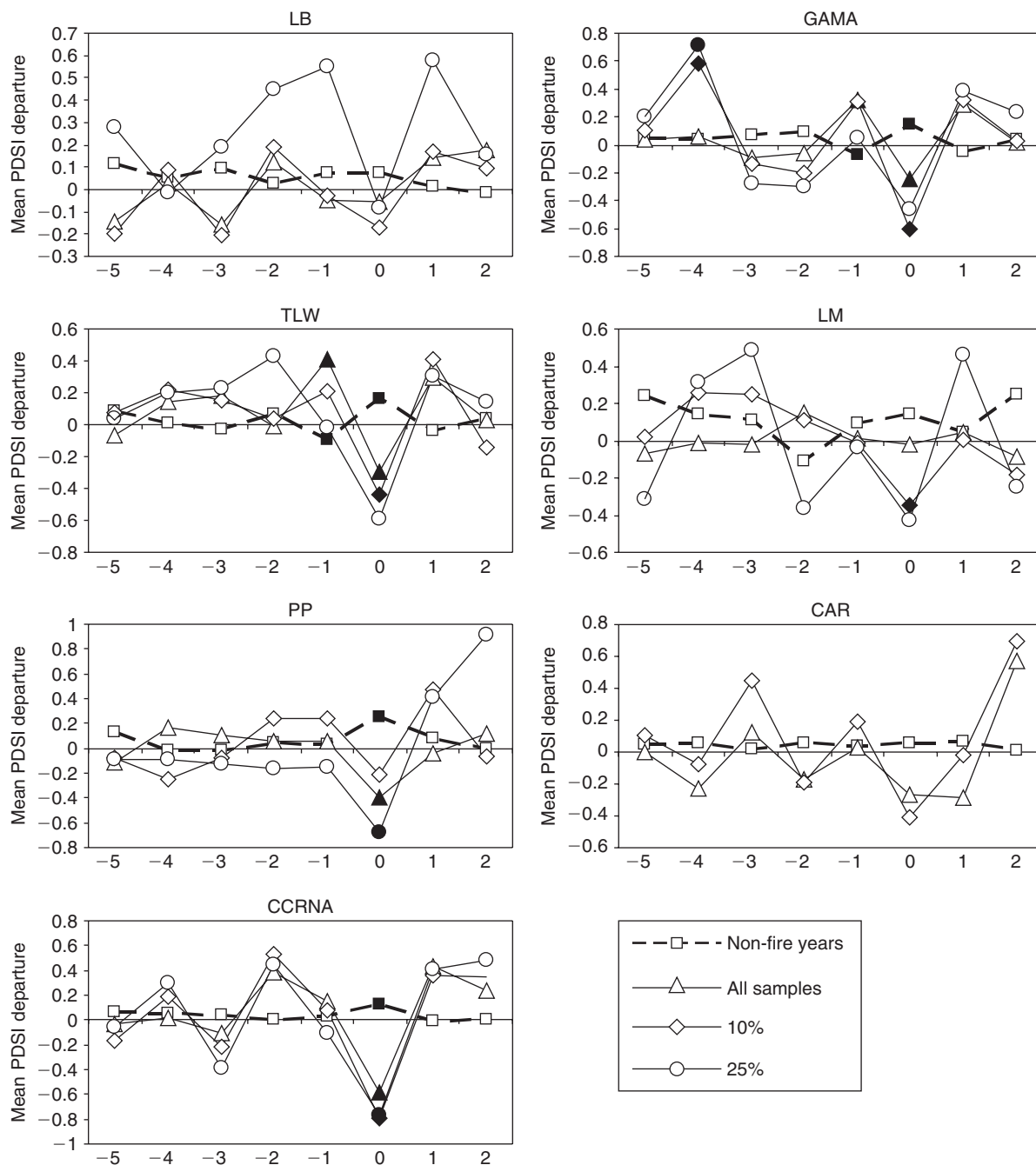
Fig. 3. Superposed Epoch Analysis (SEA) of reconstructed Palmer Drought Severity Index (PDSI) (Cook and Krusic 2004) with non-fire years and fire years of different extent (i.e. at least one sample, \geq 10\% , and \geq 25\% of samples scarred) in the southern Cascades, California, for the period 1700–1900. The analysis window includes up to 5 years before and 2 years after each fire or non-fire year. Values with filled symbols were statistically significant ( P < 0.05 ).
