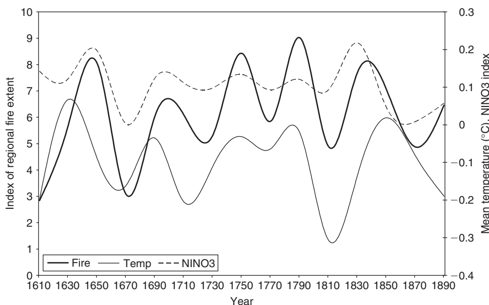
Fig. 6. Interdecadal variation in regional fire extent, Palmer Drought Severity Index (PDSI), summer temperature (TEMP), and El Niño–Southern Oscillation (ENSO) (NINO3). All series were computed from 20-year, non-overlapping means (sums in the case of fire extent) and were smoothed using a cubic spline for presentation.
