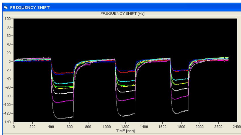
Figure 2. LibraNose 2.1 e-nose sensor-array output derived from Ganoderma lucidum -decayed Celtis australis wood block one year after artificial inoculation. Three replication analyses were performed per sample during a 2,400 s run cycle. Notice that there is a complete reversal of sorption of volatiles to the sensors as indicated by frequency shifts at three separate instances during the run.
