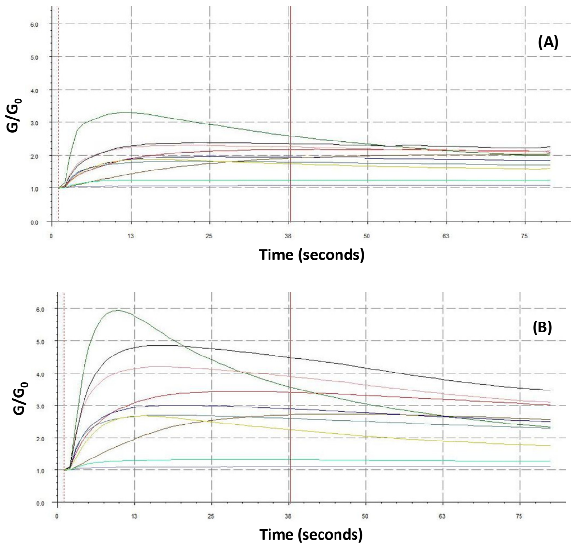
Figure 5. Typical sensor-response outputs from representative samples of healthy wood blocks (controls), and inoculated wood blocks (decayed). Sensory array output from: (A) a non-inoculated sample of Acer saccharinum , (B) and a decayed wood sample of A. saccharinum after inoculation with Armillaria mellea . Histograms of normalized intensity responses of individual sensors to headspace volatiles produced by the same Q. lyrata -samples for non-inoculated (C), and decayed wood (D), respectively. G/G_0 is the ratio of the conductivity response of the sensors to the sample gas (G) relative to the carrier gas ( G_0 ) over time. The following data were adjusted relative to the carrier gas baseline.
