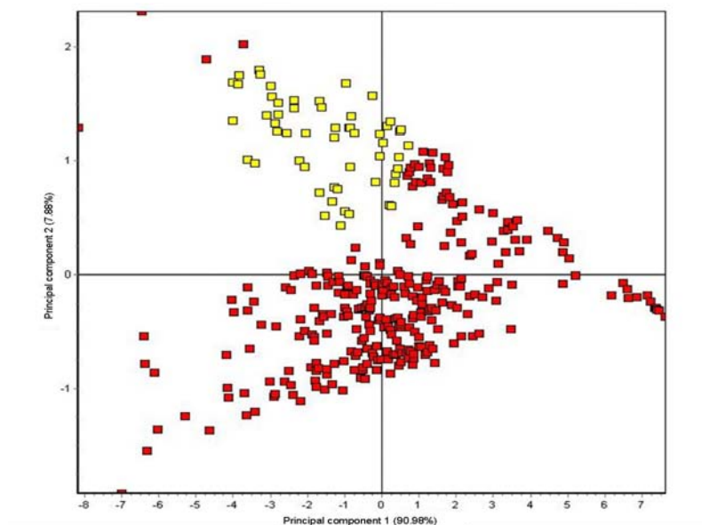
Figure 3. Aroma map plot showing discrimination of volatiles from healthy control wood blocks (yellow labels) and volatiles from artificially-inoculated decayed wood block (red labels) using principal component analysis (PCA) of mean changes (shifts) in quartz crystal oscillation frequency ( \Delta f ) in response to differences in VOC mixture composition in headspace volatiles from different sample types.
