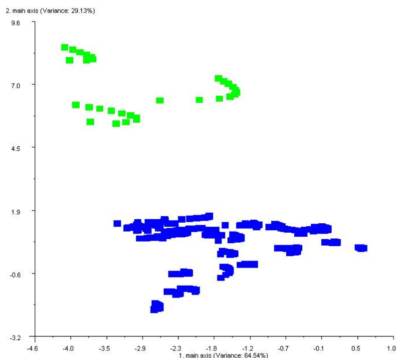
Figure 6. Discrimination of healthy (controls) and decayed (artificially inoculated) wood blocks samples by PCA based on differences in analyte principal components within headspace volatiles relative to standard deviations from the mean ( \Delta\sigma ). Color-coded labels are as follows: Green labels indicate volatiles from healthy, undecayed controls and blue labels indicate volatiles from decayed wood samples.
