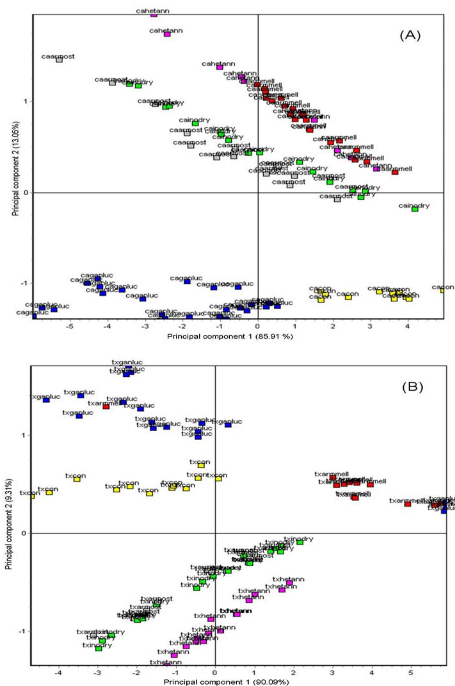
Figure 4. Aroma map plot showing discrimination of volatiles from decayed wood samples of (A) Celtis australis , (B) Tilia spp. and (C) Acer negundo by principal component analysis (PCA) of mean changes in crystal oscillation-frequency ( \Delta f ) data. Different color labels 1 indicate different wood decay fungi responsible for decay and corresponding headspace volatiles produced. The first two letters of each label indicate specific tree species according to the following abbreviations: ca = Celtis australis ; tx = Tilia sp.; an = Acer negundo . The subsequent letters following in the label indicate the wood decay fungus responsible for decaying the wood blocks for 12 months following artificial inoculation: ganluc = Ganoderma lucidum ; hetann = Heterobasidion annosum ; armmell = Armillaria mellea ; armost = A. ostoyae ; inodry = Inonotus dryadeus . Con = undecayed or healthy (control) wood blocks.
