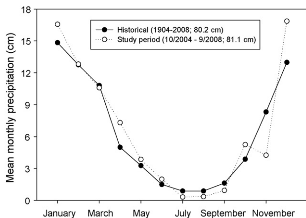
Fig. 1. Historical and 2004–2008 mean monthly precipitation at Truckee, California, USA (~15 km SSW of study site).
