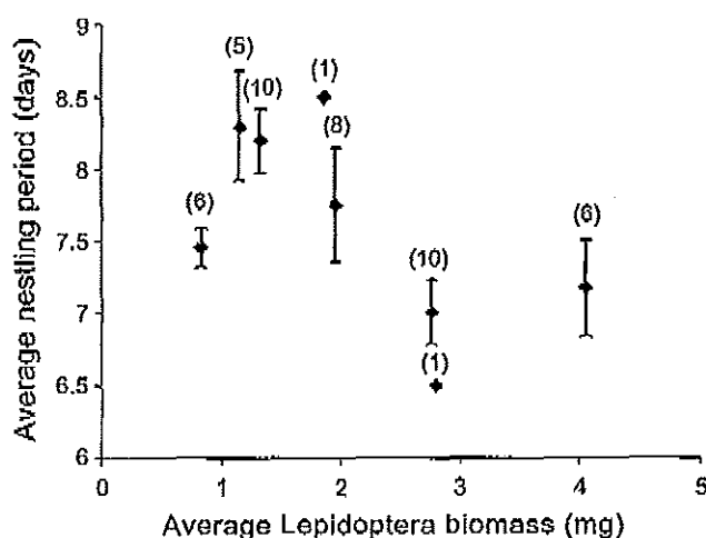
FIG. 4. Average nestling-period length (2002–2004) of a plot-year group in relation to estimated biomass (mg) of lepidopteran larvae, in Ovenbirds at Coweeta Hydrologic Laboratory, Nantahala National Forest, North Carolina. Sample sizes are given in parentheses.
