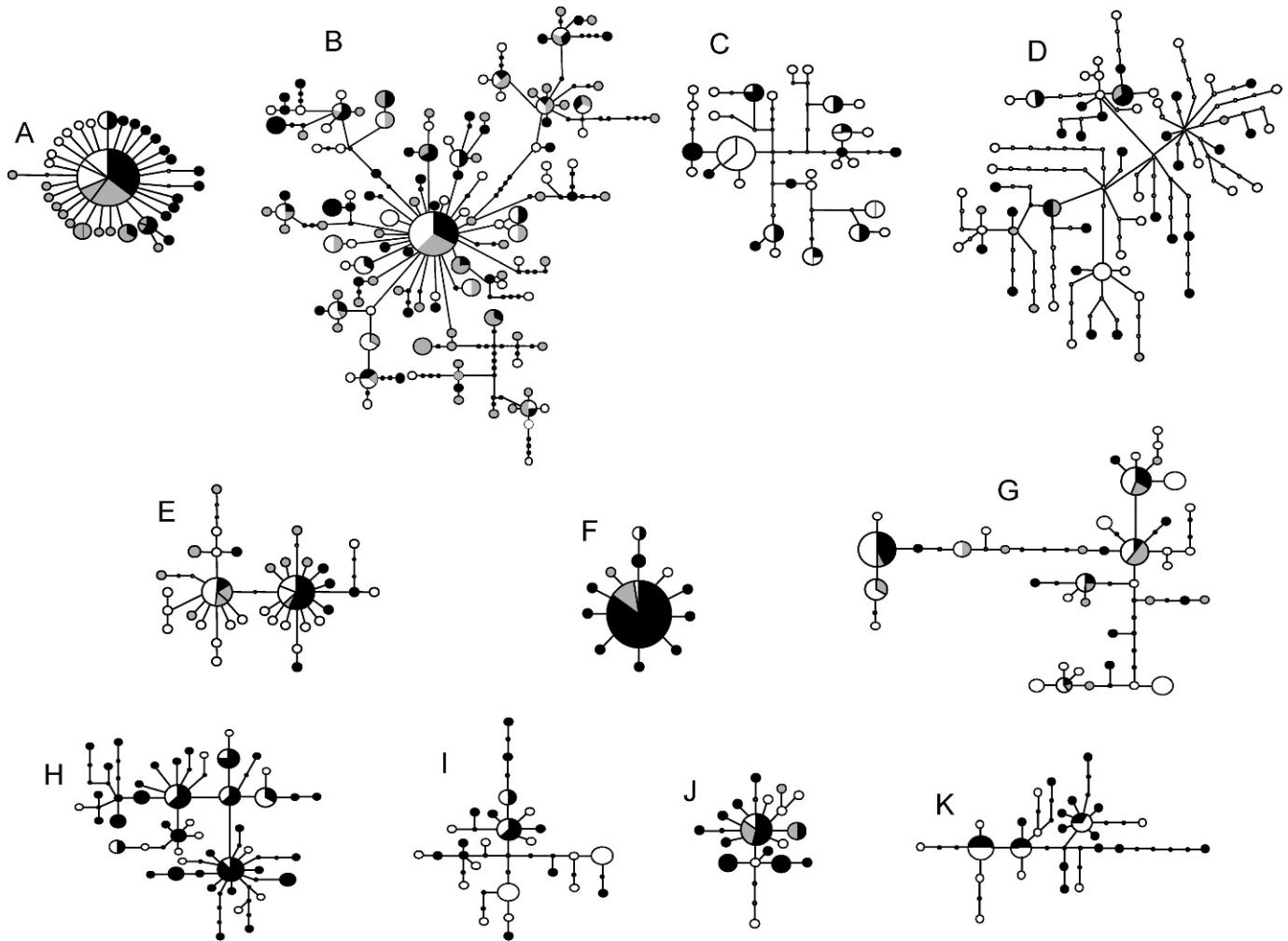
FIG. 2. Haplotype networks for 11 amphidromous species from Puerto Rico: Atya lanipes (A), Atya scabra (B), Atya innocens (C), Xiphocaris elongata (D), Macrobrachium faustinum (E), Micratya poeyi (F), Micratya sp. (G), Sicydium buscki (H), Sicydium punctatum (I), Sicydium sp. (J), and Neritina virginea (K). Each circle represents a haplotype. The size of the circle represents the relative frequency of the haplotype in the sample, and the colors represent the region where each haplotype was found (see Fig. 1).
