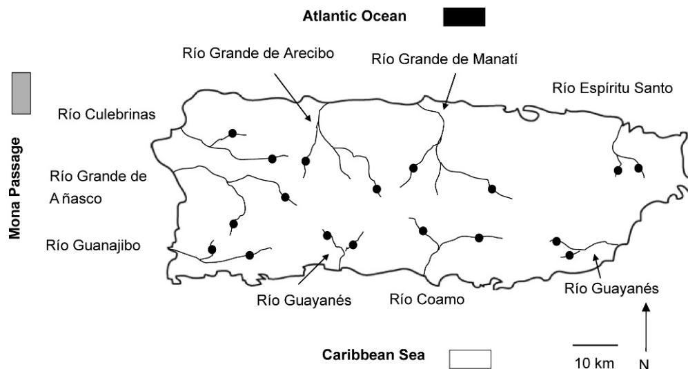
FIG. 1. Sampling locations in Puerto Rico. Shadings indicating marine regions are used in Fig. 2 to show regional distribution of haplotypes.
