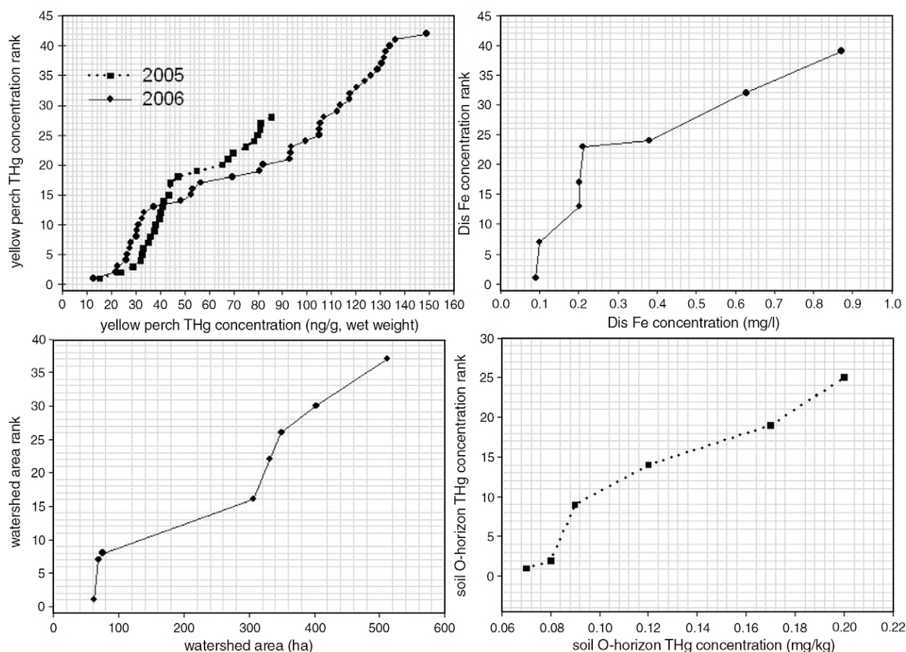
Fig. 3. Concentrations, watershed areas and associated ranks for the 2005 and 2006 models.
