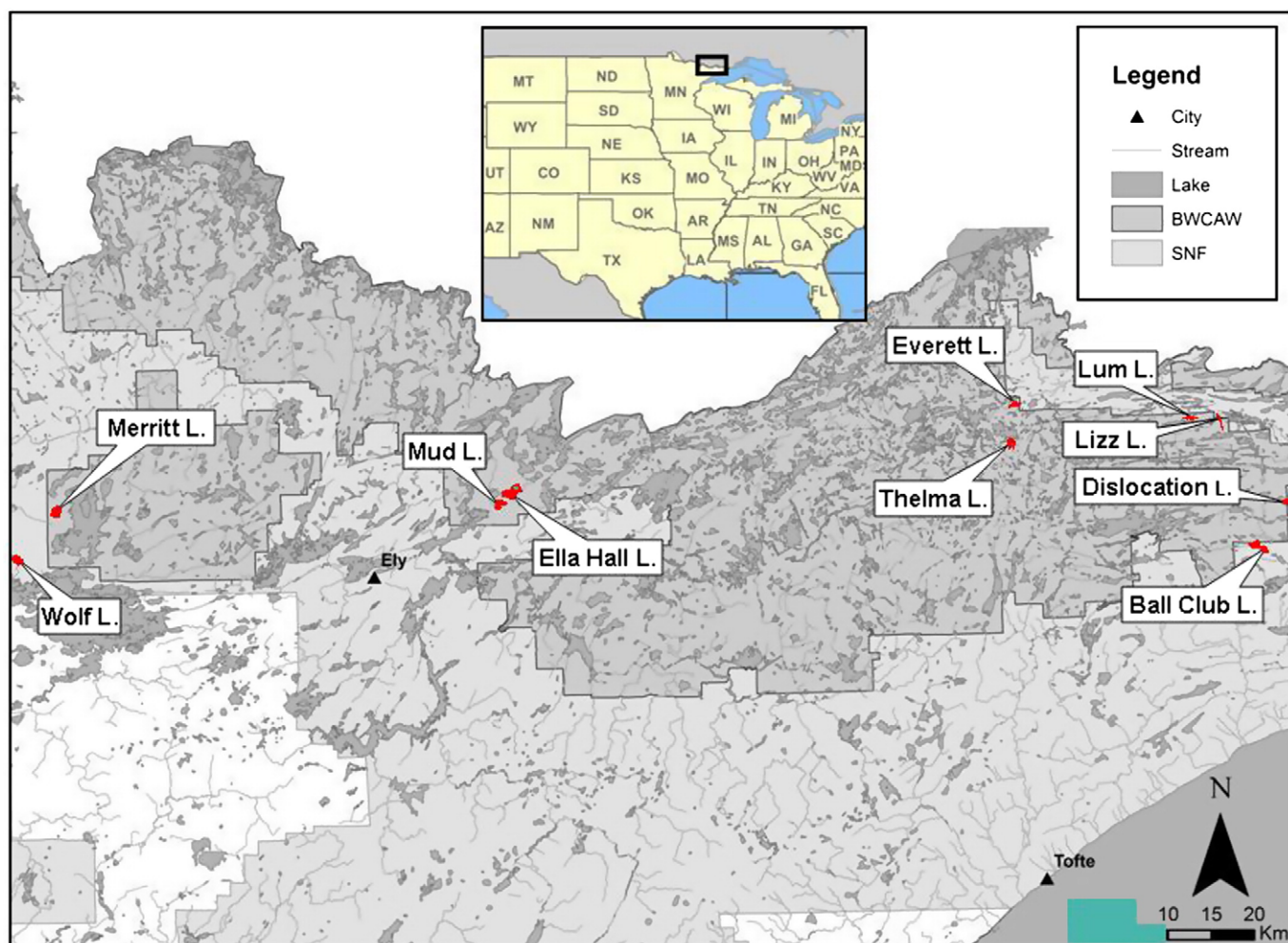
Fig. 1. Lakes and surrounding watersheds used for evaluating the spatial variation of total mercury in age 1 yellow perch, upland soil and lake water.
