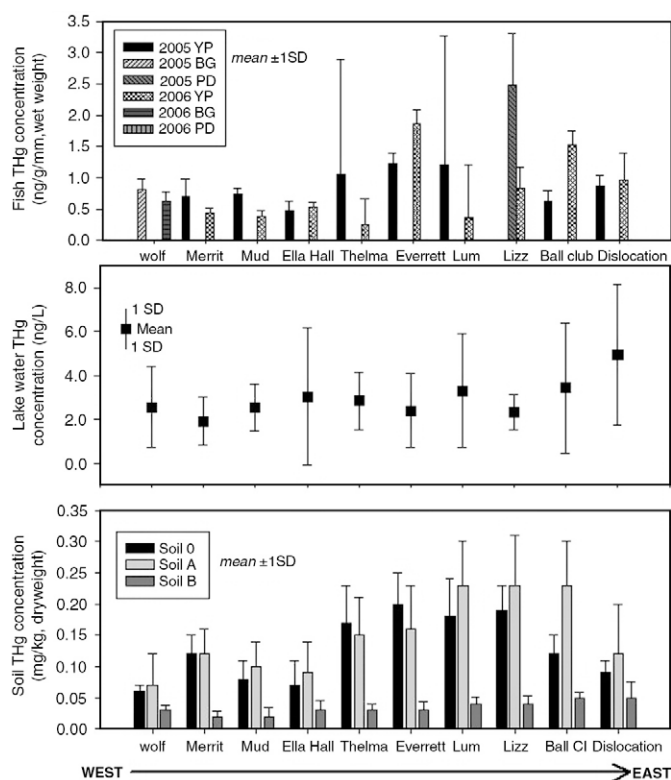
Fig. 2. Spatial representation of THg levels in lake water, upland soil and all fish species (PD = pumpkinseed fish, BG = bluegill and YP = yellow perch) for both years.
