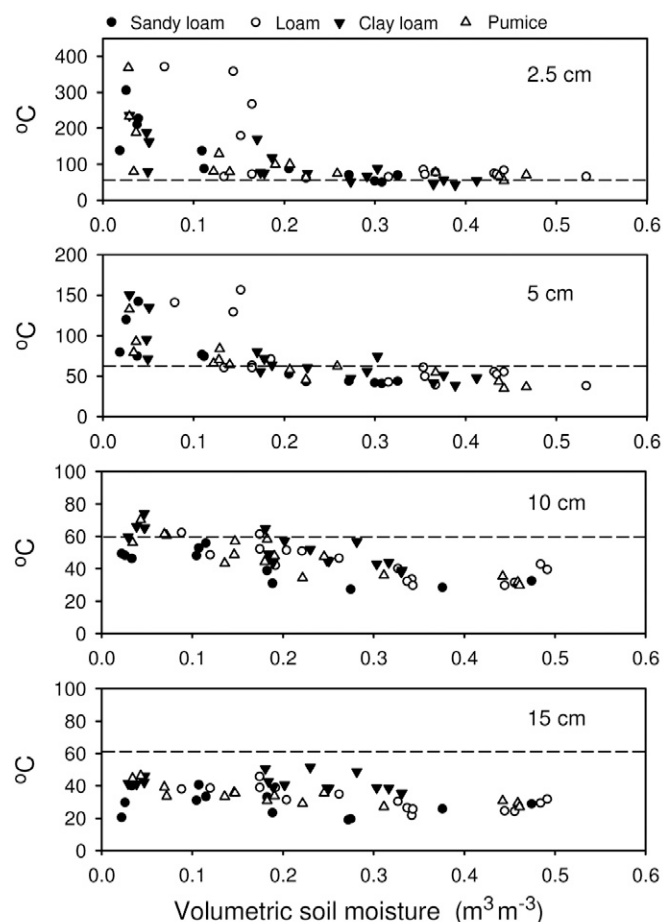
Fig. 2. Maximum soil temperatures during burning. Temperature profiles were recorded at 2.5, 5, 10, and 15 cm beneath the mineral soil surface during controlled burning ( n = 60 ). A gradient of pre-burn soil moisture contents, from air dry to field capacity, was compared in each of four soil types. Dashed lines at 60^\circ\text{C} represent the lethal threshold for plant roots.
