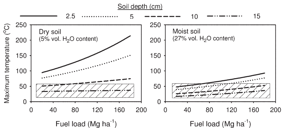
Fig. 5. Predicted maximum soil temperatures when burning woody fuels. Separate predictions are presented for dry (5% volumetric moisture) and moist (27% volumetric moisture) soil. The gray-hatched rectangle in each graph represents temperatures below the lethal threshold for roots of 60°C. The coefficient of variation associated with each response curve is 18.2%.
