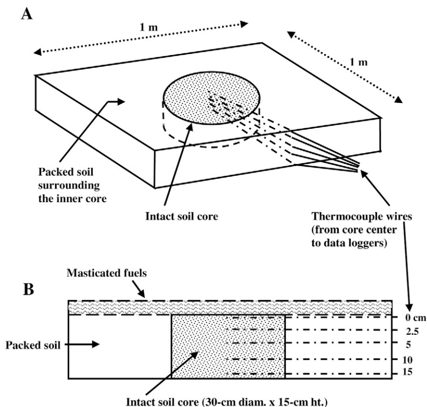
Fig. 1. Plot design: (A) view looking down on plot before fuel layering, (B) side view of plot after fuel layering. The mineral soil surface of each 1- by 1-m plot was level with the surrounding soil.
