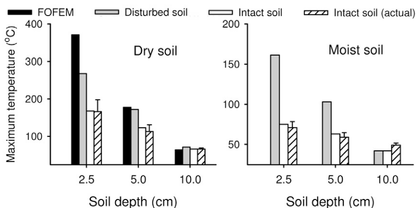
Fig. 4. Comparison of maximum temperatures in the soil profile as predicted using the FOFEM fire-effects model, an equation for disturbed soil (Busse et al. 2005), Eq. [2] from our study, and actual values from our study. All predictions used the same fuel-load profile and fuel moisture input values. Disturbed clay loam soil was collected from a forested site using shovels, then was hand sorted to remove rocks and large organics and packed to approximate the field bulk density value of 1.0 Mg m -3 before burning. Intact soil was collected from the same site by excavating large-diameter cores. Volumetric moisture content was 5 and 27% for dry and moist soil, respectively. Error bars represent standard error ( n = 4 ), and are only available for the empirical values for intact soil.
