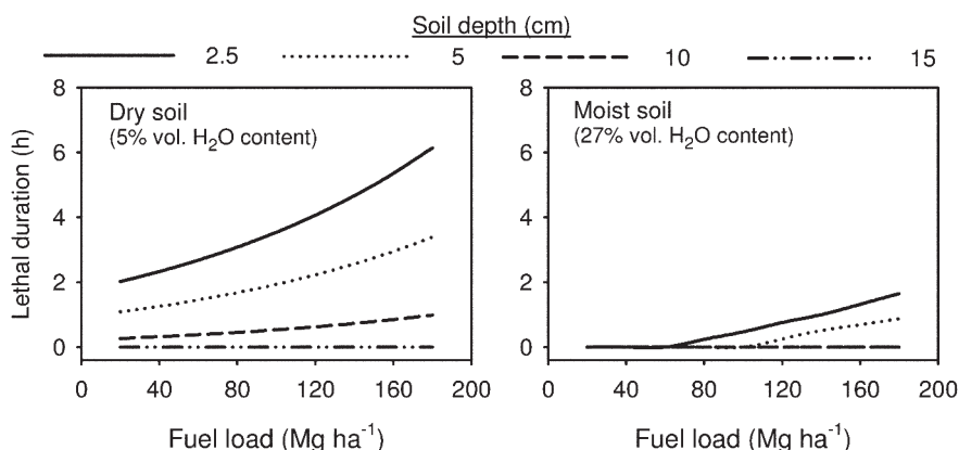
Fig. 6. Predictive model for lethal heat ( >60^{\circ}\text{C} ) duration when burning woody fuels. Separate predictions are presented for dry (5% volumetric moisture) and moist (27% volumetric moisture) soil. The coefficient of variation associated with each response curve is 17.7%.
