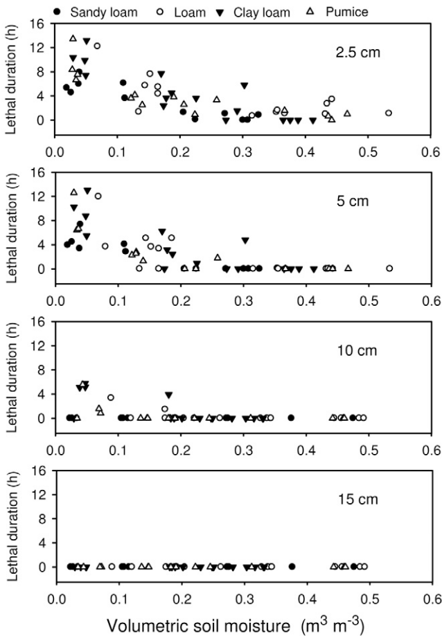
Fig. 3. Lethal heat ( >60^{\circ}\text{C} ) duration during burning. Temperature profiles were recorded at 2.5, 5, 10, and 15 cm beneath the mineral soil surface during controlled burning ( n = 60 ). A gradient of pre-burn soil moisture contents, from air dry to field capacity, was compared in each of four soil types.
