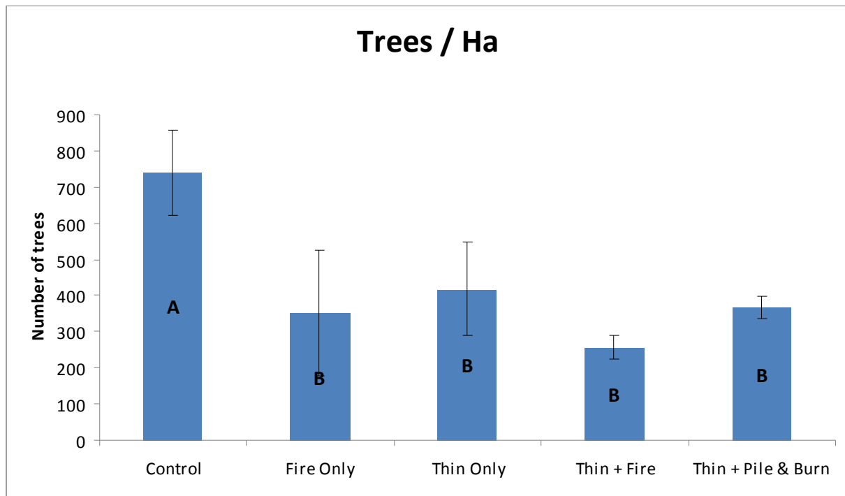
Figure 8. Mean resulting trees per hectare (with standard deviations)(n = 3 per treatment) for control and treatment plots at the Klamath Mountains study site calculated with the I-tree Eco software. Differing letters indicate statistically significant differences ( \alpha = 0.1 )
