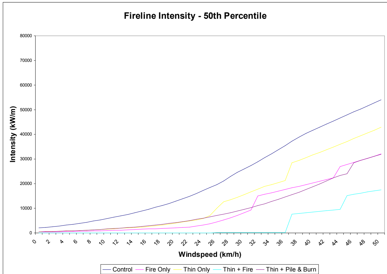
Figure 3. Calculated fireline intensity outputs from NEXUS for the Klamath Mountain study site illustrating changes resulting from increased windspeeds under 50 th percentile weather conditions.
