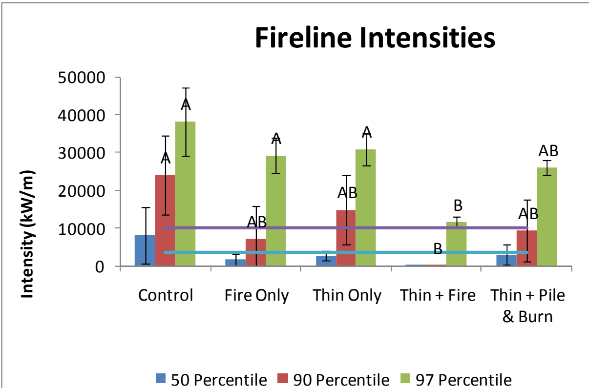
Figure 7. Mean fireline intensities (with standard deviations) under 50 th /90 th /97 th weather scenarios for different fuel treatments (n = 3 per treatment). Lower line (3,500 kW/m) indicates suppression capabilities of ground crews, upper line (10,000 kW/m) indicates overall upper suppression capabilities. Differing letters illustrate Tukeys statistical differences ( \alpha = 0.10 ).
