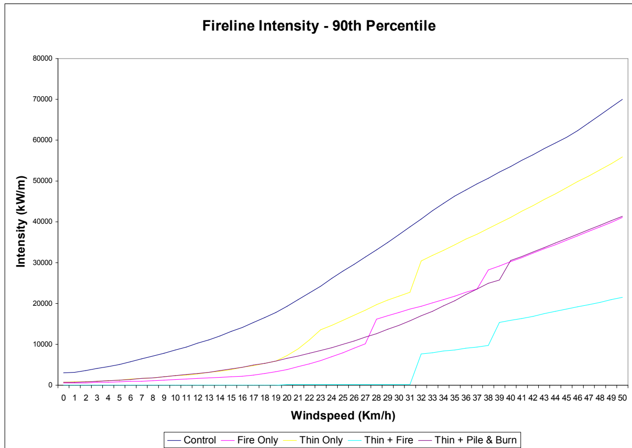
Figure 4. Calculated fireline intensity outputs from NEXUS for the Klamath Mountain study site illustrating changes resulting from increased windspeeds under 90 th percentile weather conditions.
