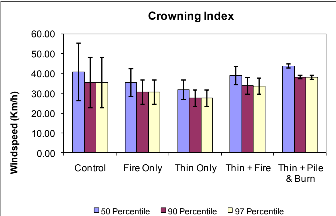
Figure 6. Mean crowning index (CI) for the various fuel treatments under 50 th /90 th /97 th percentile weather conditions in the Klamath Mountains (n = 3 per treatment). No statistical difference was observed ( \alpha = 0.10 )
