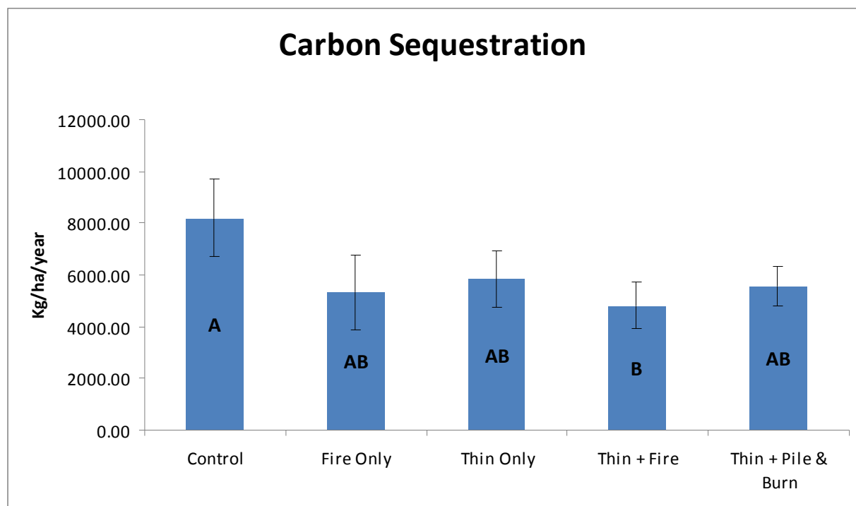
Figure 9. Mean carbon sequestration rates (with standard deviations) (n = 3 per treatment) for control and treated plots at the Klamath Mountains study site calculated using I-tree Eco software. Differing letters indicate statistically significant differences ( \alpha = 0.10 )
