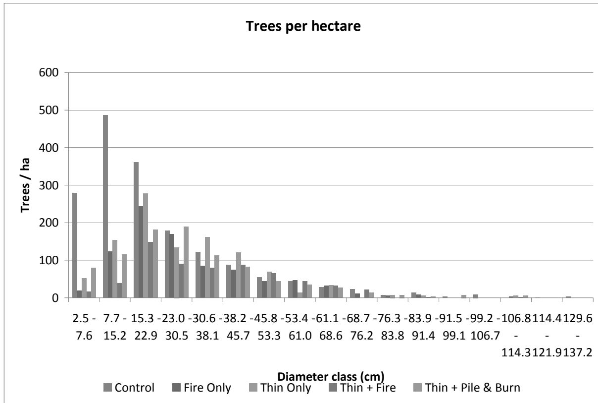
Figure 11. Mean trees per hectare by diameter class for control and treated areas in the Klamath Mountains calculated with the I-tree Eco software (n = 3 per treatment).
