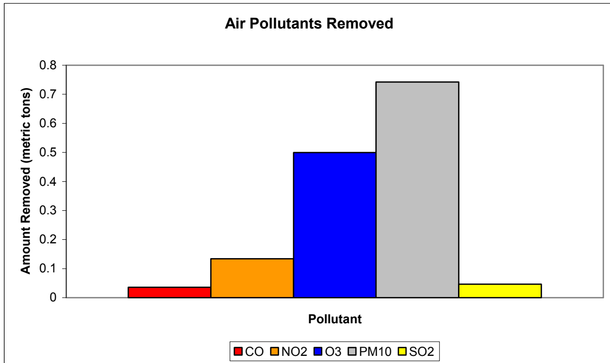
Figure 10. Total amount of pollutants removed from the forest in the Klamath Mountains study site calculated with the I-tree Eco software.
