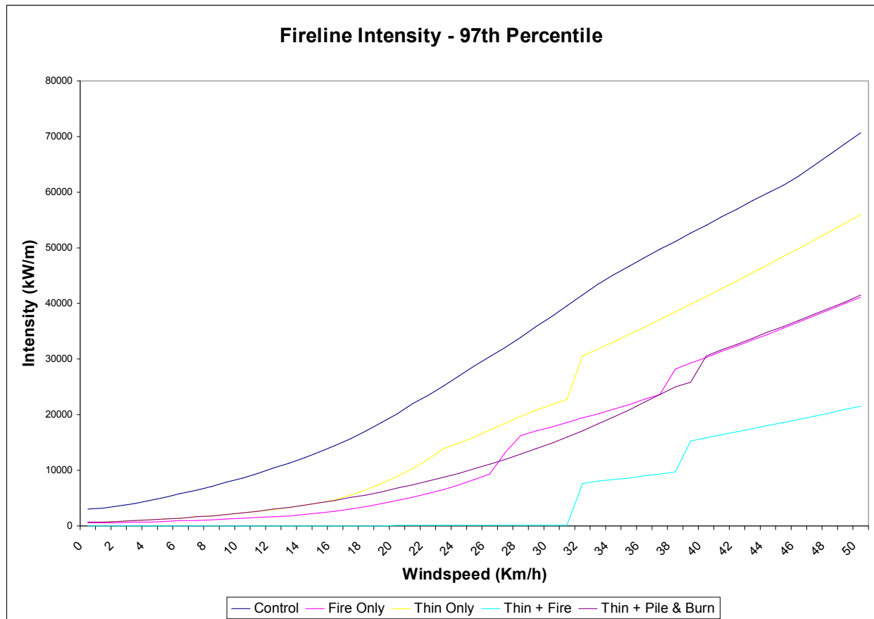
Figure 5. Calculated fireline intensity outputs from NEXUS for the Klamath Mountain study site illustrating changes resulting from increased windspeeds under 97 th percentile weather conditions.
