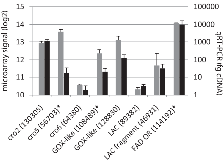
FIG. 3. Transcript levels of P. placenta genes encoding copper radical oxidases (Ppl130305, Ppl56703, and Ppl64380), GMC oxidoreductases with distant similarity to glucose oxidase (GOX; Ppl108489 and Ppl128830), an intact laccase (Ppl89382), a truncated laccase model (Ppl46931), and the highly expressed FAD-dependent oxidoreductase Ppl114192 (Table 4). Gray bars and the left axis represent log 2 microarray signals. Blackened bars and the right axis represent cDNA as determined by competitive RT-PCR. Asterisks indicate protein models whose peptides were identified in concentrated filtrates of aspen-grown cultures.
