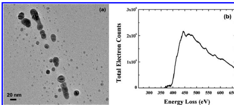
Figure 4. (a) TEM image of an Ag nanoparticle on a CNC surface where an EELS spectrum was obtained. (b) EELS spectrum showing an energy-loss edge at 367 eV.
