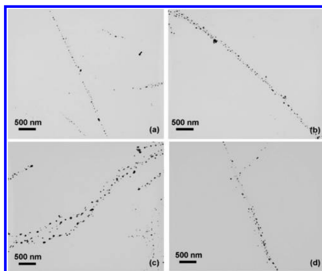
Figure 5. TEM images with varying concentrations of CTAB: (a) 0.1, (b) 0.2, (c) 0.5, and (d) 1.0 mM. These images show that the optimum Ag nanoparticle synthesis on tunicate CNC occurred at 0.5 mM.
