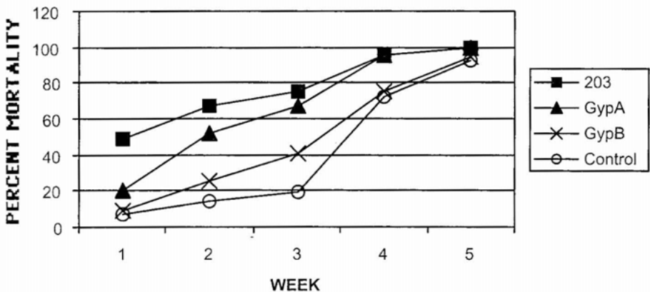
Fig. 1. Average cumulative percent mortality (all sources) calculated weekly for four treatment classes for 5 weeks posttreatment. Mortality recorded for the first week after collection only.
