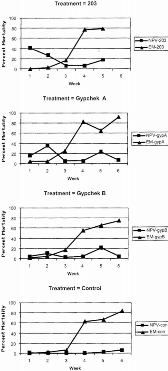
Fig. 2. Mortality from NPV and Entomophaga maimaiga calculated weekly for four treatment classes for 6 weeks posttreatment. Mortality recorded for the first week after collection only.
