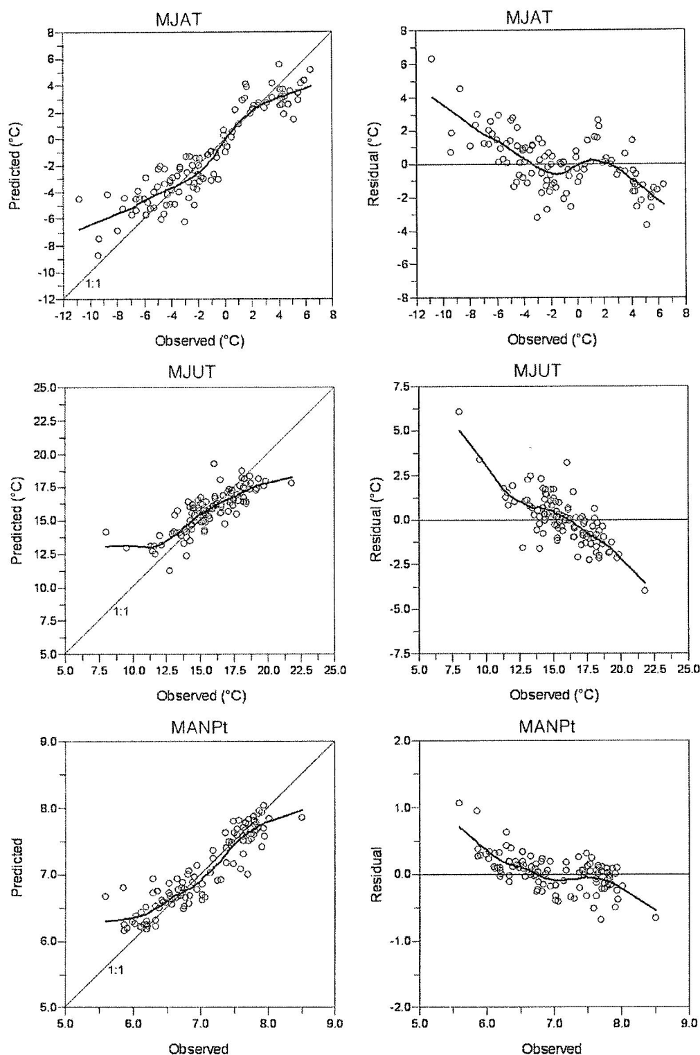
Fig. 3. Weighted averaging-partial least squares regression (WA-PLS) of quadrat frequencies ( F_q ): scatter plots of predicted (by leave-one-out cross-validation [jackknifing]) vs. observed value and residual (predicted-observed) vs. observed value based on the two-component model for MJAT, MJUT, and MANPt. The heavy lines are LOESS (locally weighted polynomial regression; span = 0.45) fits intended to accentuate patterns within the scatter plots.
