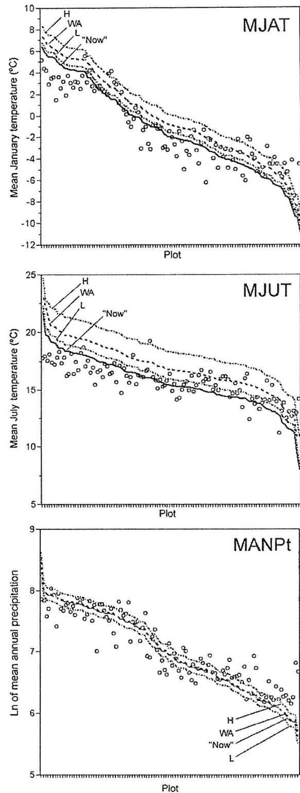
Fig. 4. Assessing the potentials of our MJAT, MJUT, and MANPt transfer functions to ascertain the climate changes predicted for Oregon and Washington by global models for the first 30-year period of this century. "Now" lines show observed climate for 107 Oregon and Washington plots from calibration set (in order from high to low). Points denote climate predicted by two-component WA-PLS model for quadrat frequencies, F_{q_i} , for same plots. H lines depict climate given the highest model prediction for 2000–2029. WA lines depict climate given the weighted average model prediction for 2000–2029. L lines depict climate given the lowest model prediction for 2000–2029.
