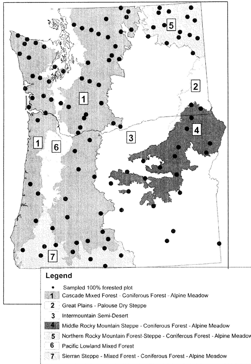
Fig. 1. Map of Oregon and Washington showing the locations of 107 FIA Phase 3 plots included in the calibration set. Vegetation classification follows Cleland et al. (2007).
