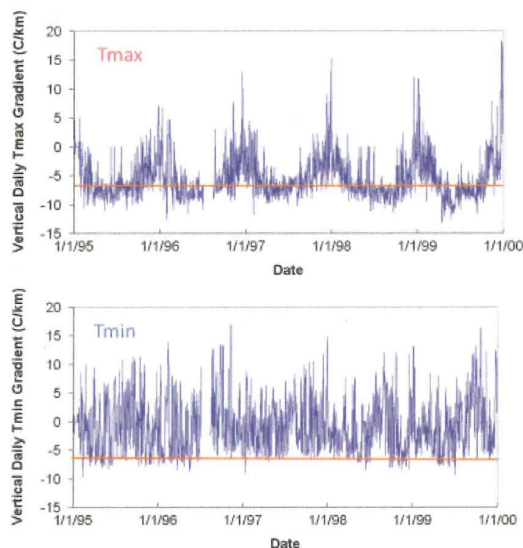
Figure 2. Time series plots of \Delta T_{\text{HV}\max} and \Delta T_{\text{HV}\min} (Hill–Valley daily T_{\max} and T_{\min} differences, respectively, expressed in °C/km elevation), for the period January 1995–December 1999. Orange horizontal line represents a constant, fully synchronous, vertical daily temperature gradient at the environmental (global mean) lapse rate of -6.5 °C/km. T_{\max} and T_{\min} are clearly asynchronous between these two sites, and \Delta T_{\text{HV}\max} and \Delta T_{\text{HV}\min} are often much less negative than the environmental lapse rate. \Delta T_{\text{HV}\max} shows a clear seasonal cycle in vertical gradient, while \Delta T_{\text{HV}\min} does not. This figure is available in colour online at www.interscience.wiley.com/ijoc
