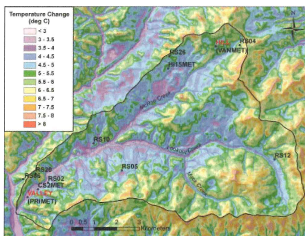
Figure 7. Estimated spatial distribution of December T_{\max} response to a 2.5°C regional temperature increase and a 10-day increase in the A-C index across the HJA (outlined in black). T_{\max} response was modeled with multiple regression for 12 stations (shown on map) using elevation and local topographic position as explanatory variables. Intricate patterns of elevation and topographic position create steep response gradients across the landscape. This figure is available in colour online at www.interscience.wiley.com/ijoc
