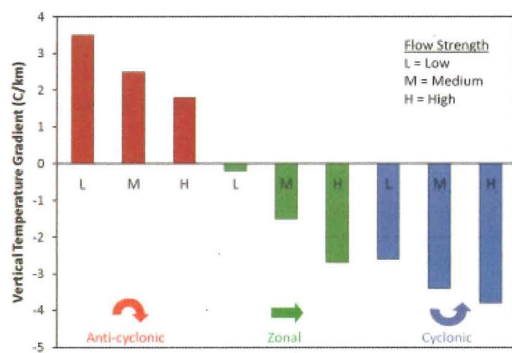
Figure 3. Relationship between 700-hPa (~3000 m) flow strength and curvature and mean daily \Delta T_{HVmin} for all days in the period 1987–2005. Cyclonic, or troughing, curvature days are often cloudy and wet with good atmospheric mixing. Anti-cyclonic or ridging, curvature days are generally clear and dry with poor atmospheric mixing. Zonal flow, with little curvature, exhibits weather that is transitional between cyclonic and anti-cyclonic conditions. Each flow curvature pattern was divided into three flow strength categories: low, medium and high. Average \Delta T_{HVmin} follows a smooth transition from positive in the low flow strength anti-cyclonic flow category to negative in the high flow strength cyclonic flow category. This figure is available in colour online at www.interscience.wiley.com/jloc
