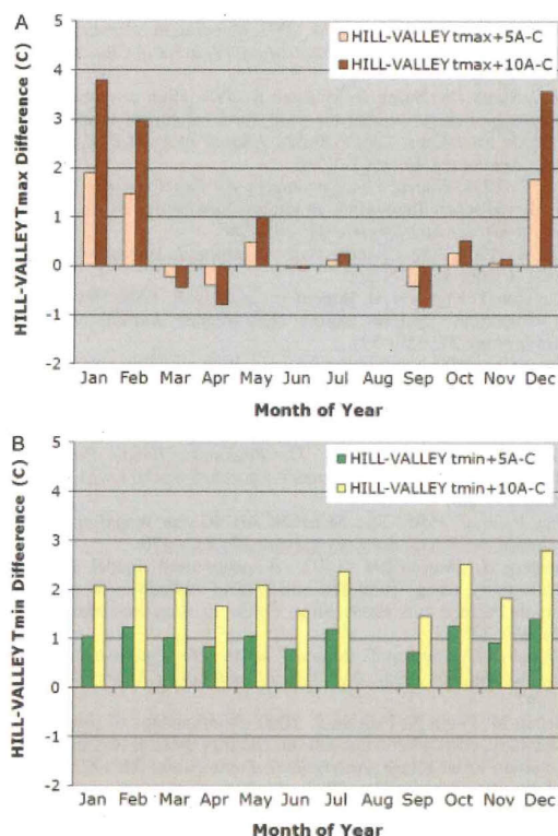
Figure 6. Differences in (a) T_{\max} and (b) T_{\min} responses between HILL and VALLEY for each month, given increases in the A-C index of 5 and 10 days. T_{\max} differences are largest in winter, when cold air pooling can occur at both day and night due to low sun angles. T_{\min} differences are relatively constant throughout the year, but tend to be largest in the fall, when clear, calm conditions are more common. This figure is available in colour online at www.interscience.wiley.com/ijoc
