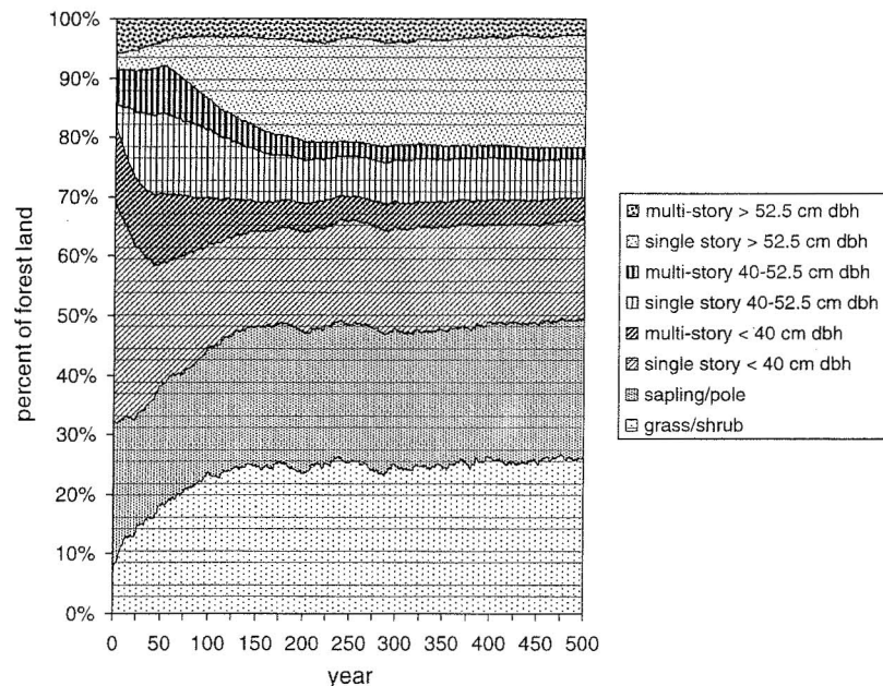
Fig. 4. Percentage of land in various vegetation structural conditions in a portion of the upper Grande Ronde subbasin, Northeastern Oregon.
