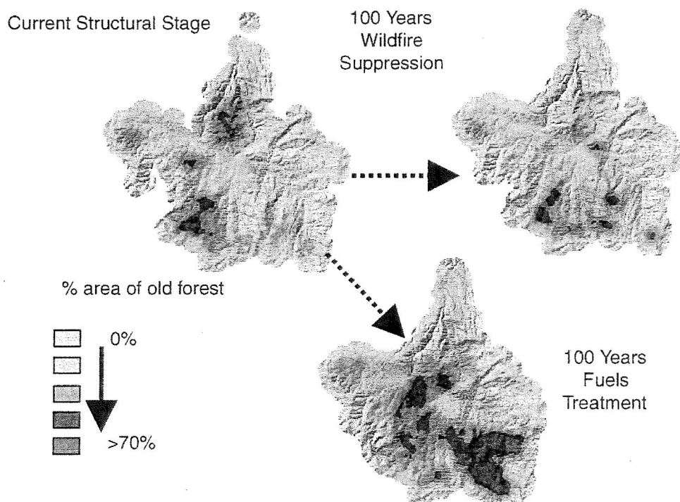
Fig. 5. Percentage of land in old forest structural conditions with and without fuels treatment in a portion of the upper Grande Ronde subbasin, Northeastern Oregon.
