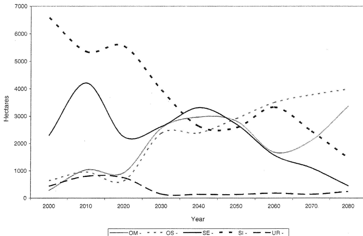
Fig. 10. Results of simulations for the Mt. Emily area showing changes over time in forest structure for an active fuel treatment scenario. Structure classifications follow Keyes and O'Hara (2002) and were determined with the FVS cover extension (Crookston and Stage, 1999). OM, old forest multistory; OS, old forest single story; SI, stand initiation; UR, understory initiation; SE, stem exclusion.
