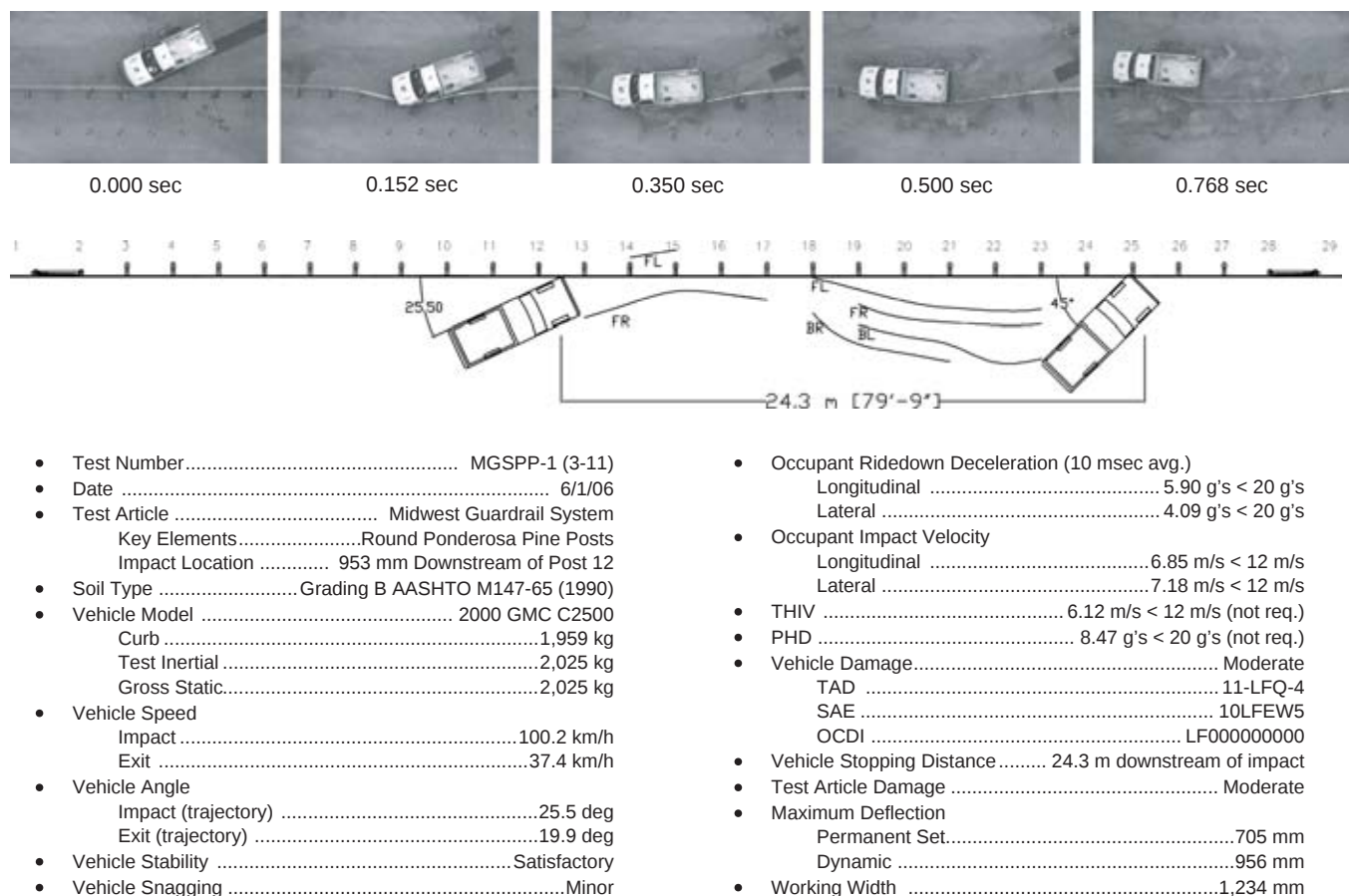
FIGURE 7 Test results and sequential photographs, Test MGSP-1.
