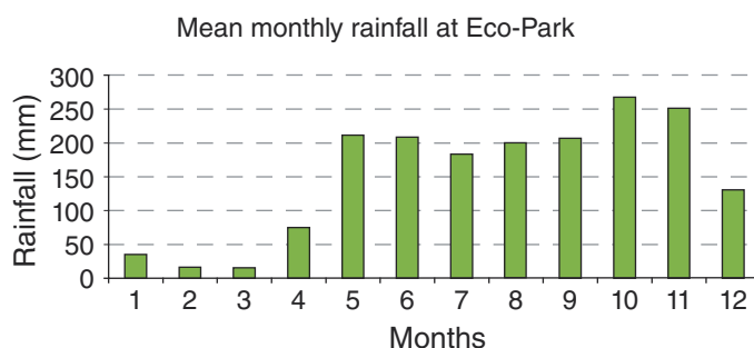
Figure 2—Mean monthly rainfall at Eco-Park.
