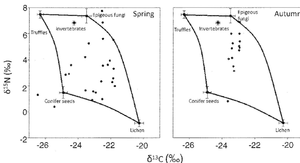
FIG. 2.—Distribution of isotopic values (mean \pm SE) of potential foods and individual flying squirrels ( Glaucomys sabrinus griseifrons ) in spring and autumn on northern Prince of Wales Island, Alaska, for a concentration-dependent mixing model. The lines connecting potential food sources enclose the mixing space for the dual-isotope linear mixing models used to convert isotopic data to estimates of relative contribution. Although \delta^{13}\text{C} and \delta^{15}\text{N} values of several individual squirrels fell out of the mixing space, mean values were well within it in both autumn ( \delta^{13}\text{C} = -23.20\text{‰} \pm 0.06\text{‰} ; \delta^{15}\text{N} = 4.77\text{‰} \pm 0.46\text{‰} ) and spring ( \delta^{13}\text{C} = -23.07\text{‰} \pm 0.26\text{‰} ; \delta^{15}\text{N} = 3.13\text{‰} \pm 0.39\text{‰} ). We removed values for berries from the linear mixing model because berry seeds were not observed in feces.
