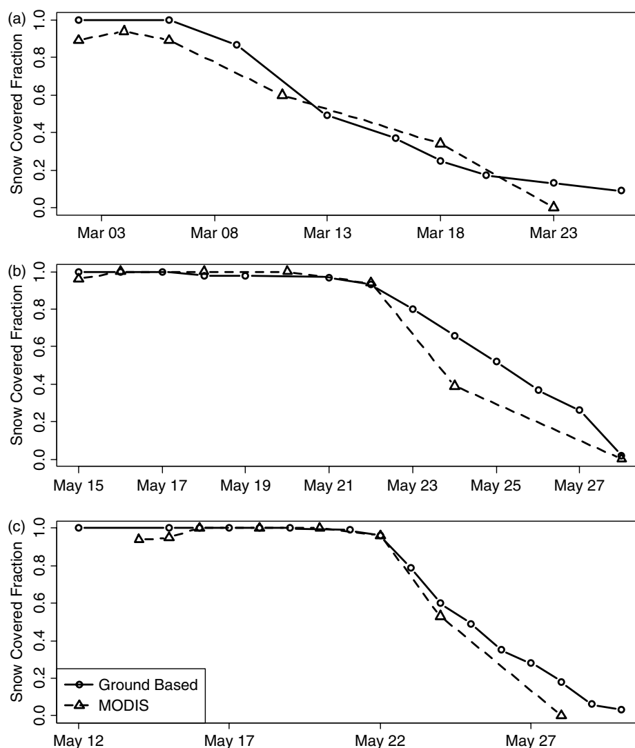
Figure 4. Ground-based FSCA ( FSCA_{ground} ) evaluated against MODIS-based NDSI-derived FSCA ( FSCA_{NDSI} ) for a) Little Deer Point, b) Innavait Creek A, and c) Innavait Creek B
