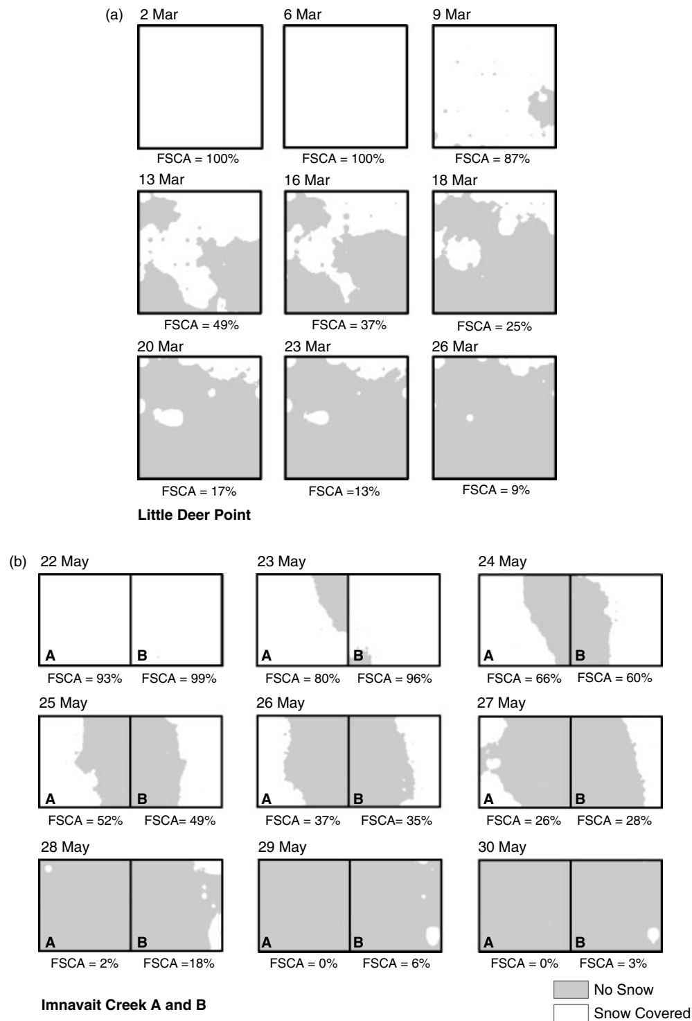
Figure 2. Ground-based FSCA mapped throughout snowmelt
