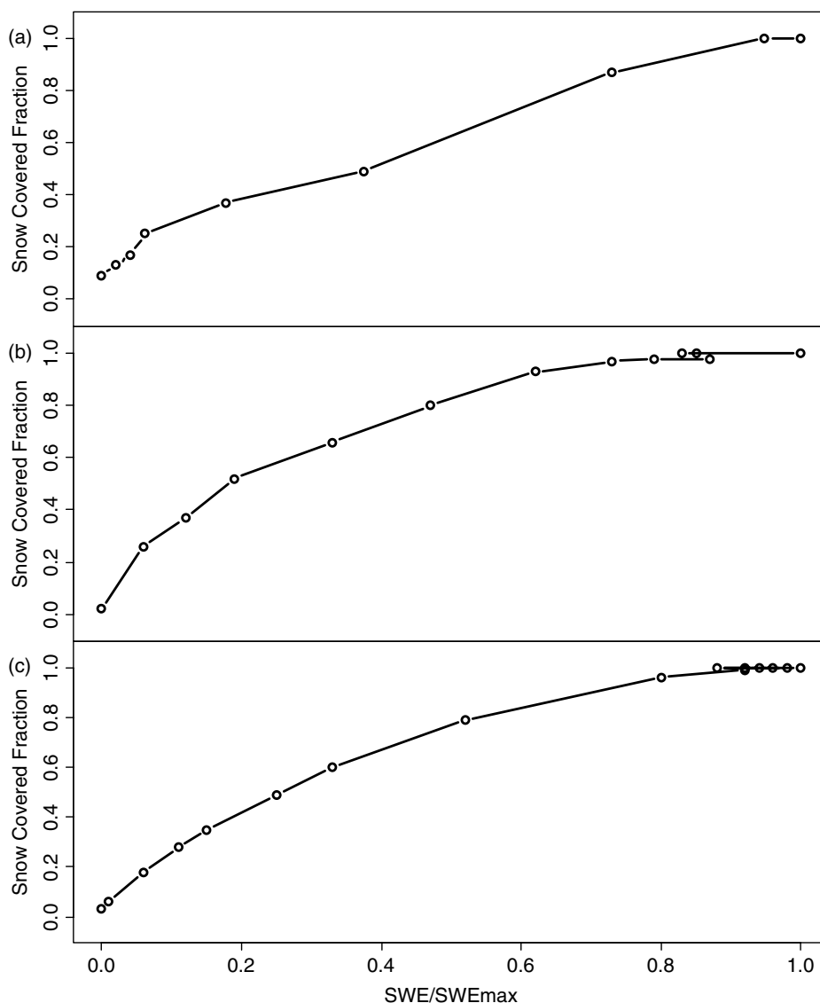
Figure 3. Ground-based depletion curves for a) Little Deer Point, b) Imnavait Creek A, and c) Imnavait Creek B
