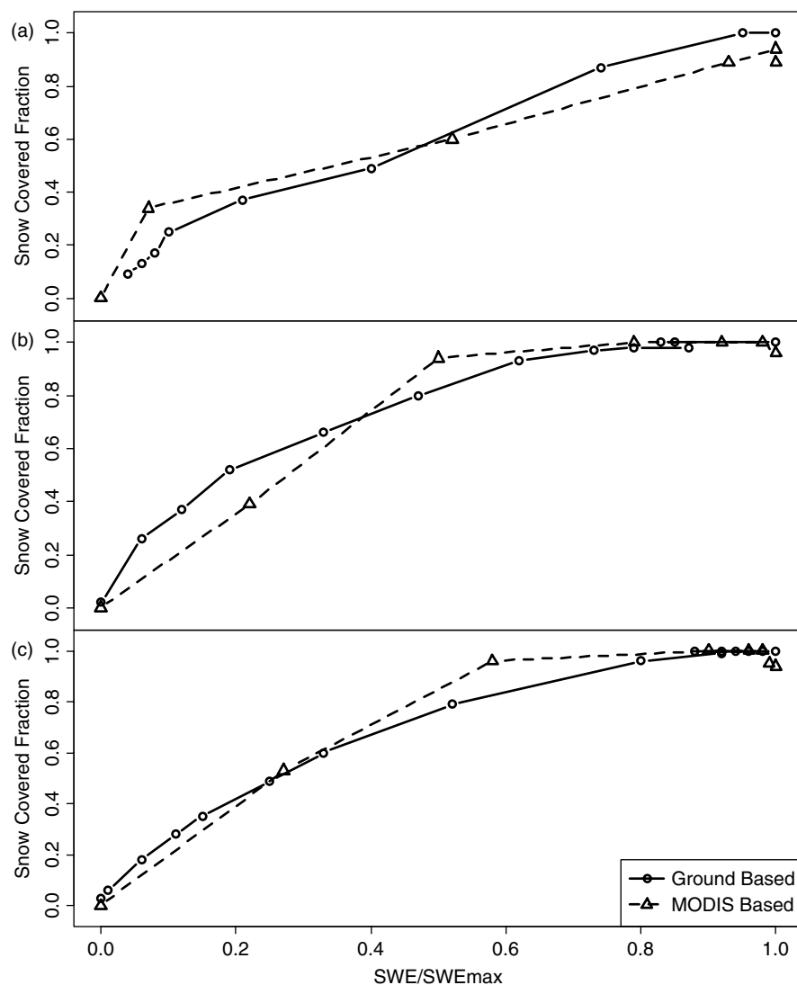
Figure 6. Depletion curves derived from remotely sensed data compared to ground observations for a) Little Deer Point, b) Innavaik Creek A, and c) Innavaik Creek B
