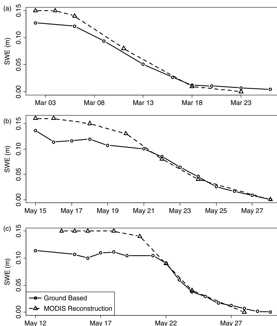
Figure 5. UEB/MODIS reconstructed SWE compared to ground snow surveys at a) Little Deer Point, b) Innavait Creek A, and c) Innavait Creek B
