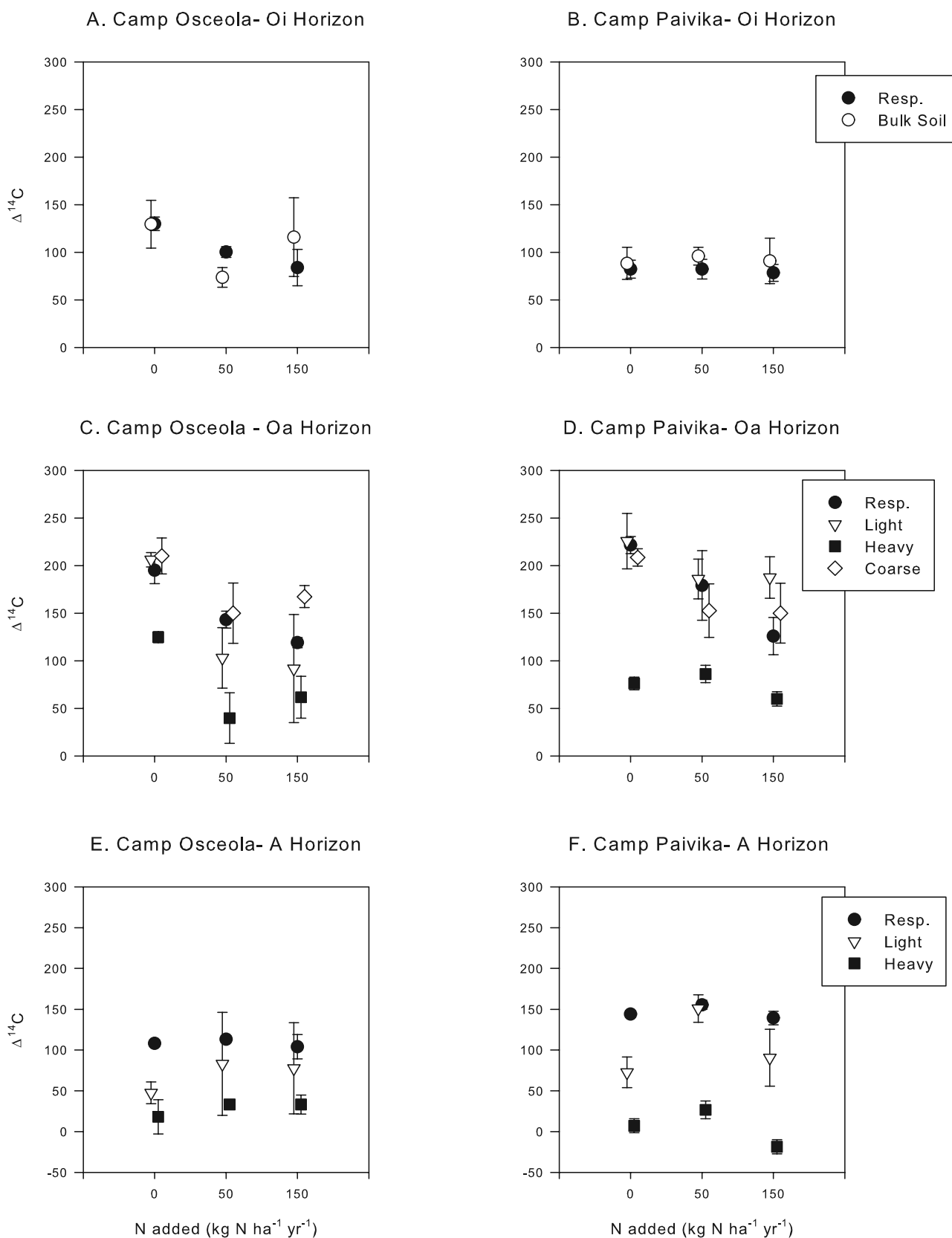
Figure 2. Comparison of SOM and heterotrophic respiration \Delta^{14}\text{C} . Black circles represent respiration, open circles represent bulk SOM, open triangles represent the light fraction ( <1 mm), black squares represent the heavy fraction ( <1 mm), and open diamonds represent the coarse fraction ( >1 mm). (a, c, and e) Camp Osceola is the clean site, and (b, d, and f) Camp Paivika is the polluted site. Error bars represent the standard deviation.
