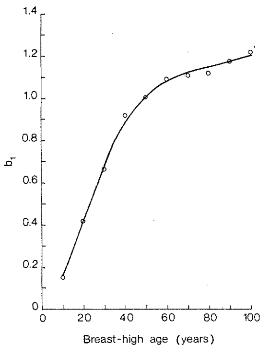
Figure 8.-- b_1 values in the equation HT - 4.5 \text{ feet} = a_1 + b_1 ( SI - 4.5 \text{ feet} ) as a function of age. Plotted points are actual b_1 values. Solid lines are curves expressed by the equation \hat{b}_1 = e^{x3} . Coefficient x3 is defined in the text. Standard error and R^2 values are 0.031 and 0.9966, respectively.
