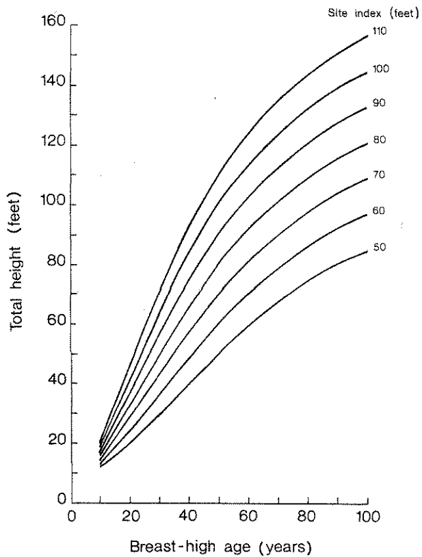
Figure 3.--Height growth curves for grand or white fir east of the Cascades in managed, even-aged stands.
