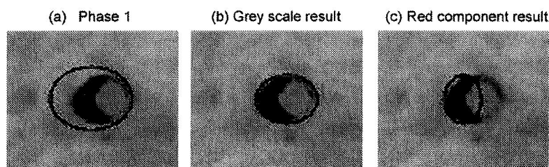
Fig. 6. Over-sized (grey) and under-sized (red) knot detection.
