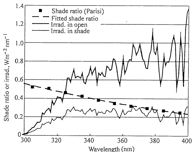
Figure 12.3 Ratio of spectral irradiance on horizontal surfaces in tree shade to irradiance on the horizontal in the open (Parisi et al., 2001b)=square points; polynomial fitted to the shade ratio points=dashed line; spectra of UV irradiance in the open at Lauder, New Zealand on the summer solstice from McKenzie and Liley (Chapter 2, this volume)=heavy black line; and irradiance in tree shade predicted by the Parisi et al. (2001b) shade ratios=thin line
