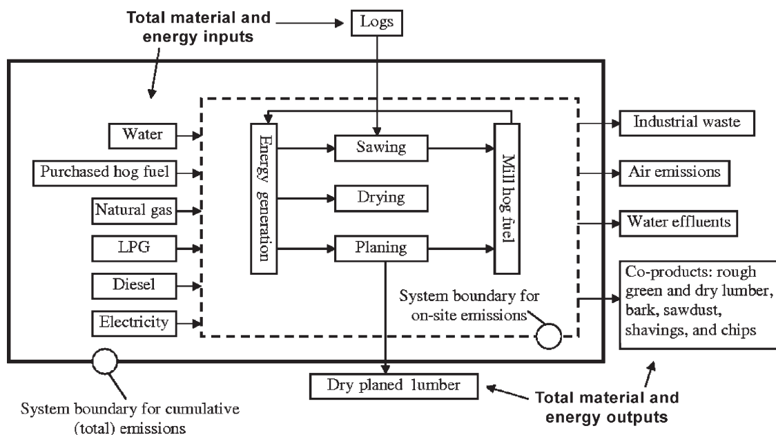
Figure 3. System boundaries for softwood lumber production.
